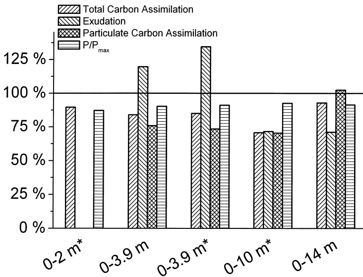
Figure 5. Effects of UV on total C assimilation, exudation and particulate C assimilation of phytoplankton moved through different mixing depths (samples with low UV = 100%, the asterisks indicate incubation at September 15, no marker = September 13, 1999). The modelled inhibition parameter P/P_{max} is given for comparison
