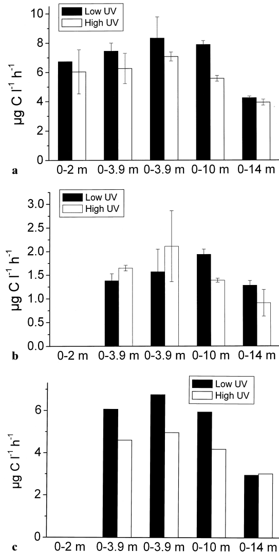
Figure 4. Average and standard deviation of total carbon assimilation (a), exudation (b) and particulate carbon assimilation (c) with high (quartz) and low (Duran) UV on Sept. 13 and 15, 1999
