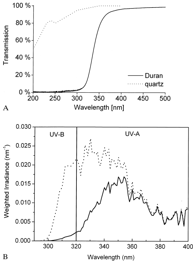
Figure 1. A Transmission properties of the Duran and quartz bottles used for incubation experiments. (Quartz bottle data are redrawn from Fig. 1 of Bühlmann et al. (1987)). B Surface spectral irradiance for local solar noon on September 13, 1999 at Lake Lucerne (see Neale et al., 2001b, this issue) as weighted with the biological weighting function for UV inhibition of photosynthesis by Lake Lucerne phytoplankton and after application of spectral transmission (Fig. 1A) of quartz (broken line) and Duran (solid line) bottles. Vertical line marks the spectral boundary between UV-B and UV-A
