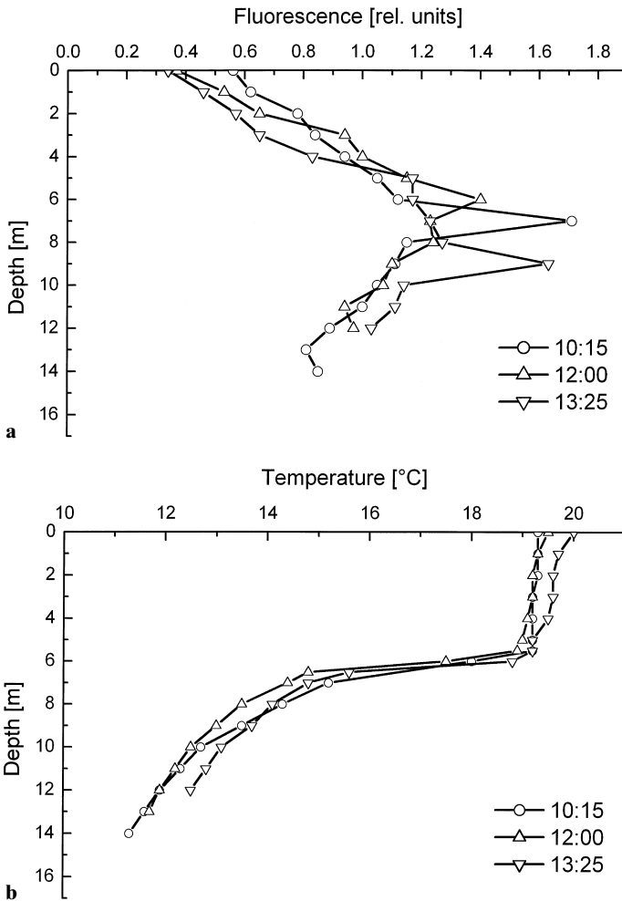
Figure 2. Vertical profiles of chlorophyll fluorescence (a) and temperature (b) at Lake Lucerne on September 15, 1999
