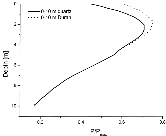
Figure 6. Vertical profile of calculated relative production ( P/P_{\max} ) in quartz bottles with high UV (solid line) and in Duran bottles with low UV (dotted line)
