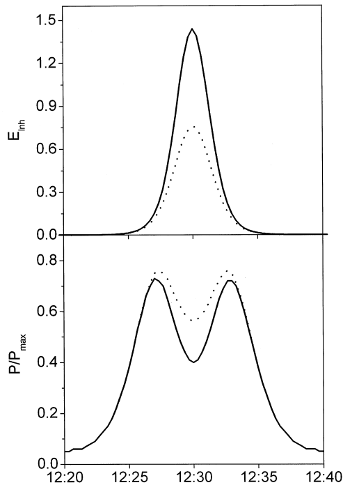
Figure 7. Time course of calculated parameters of UV-inhibition in bottles with high UV (quartz, solid line) and with low UV (Duran, dotted line) moved at a circular path between surface and 14 m depth, September 15, 1999. Top: biologically effective fluence rate for inhibition of photosynthesis E_{inh}^* , bottom: relative production P/P_{max}
