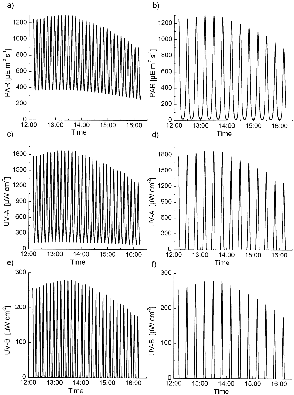
Figure 3. Time course of intensity of PAR (a, b), UV-A (c, d) and UV-B (e, f) available to phytoplankton moved from 0–3.9 m (a, c, e) and from 0–14 m (b, d, f)
