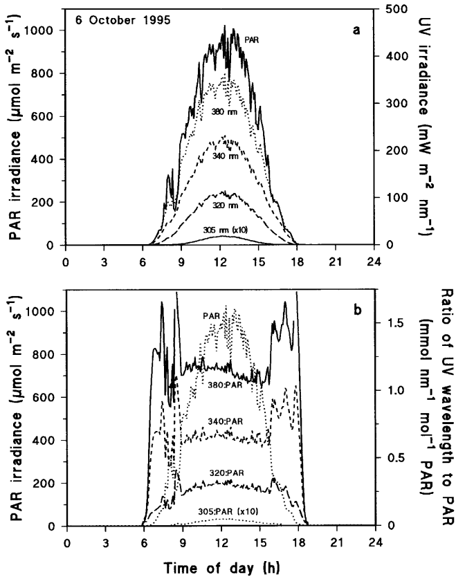
Fig. 9 a Diurnal variation in irradiance in each of four UV wavelengths (305, 320, 340 and 380 nm; right-hand axis ) and of PAR ( left-hand axis ) at Helgoland on 6 October 1995. b Diurnal variation in the ratio of each UV wavelength (305, 320, 340 and 380 nm) to PAR calculated from simultaneous irradiance readings on 6 October 1995
