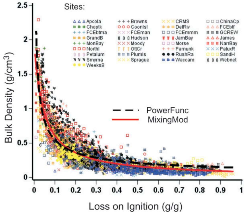
Figure 1. Best fits of the power function (— · —) BD = a LOI^b and ideal mixing model (—) BD = 1/[LOI/k_1 + (1 - LOI)/k_2] to the complete collection of 5075 sediment samples from 33 tidal marshes and mangroves distributed around the United States. The data in Figure 1 are available in Appendix S1, Supporting Information
