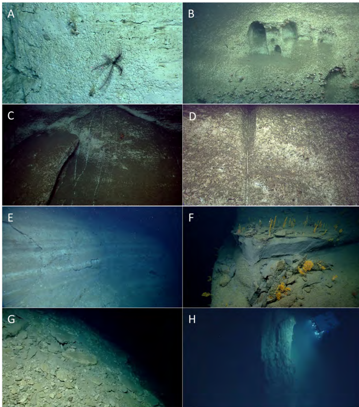
Fig 2. Examples of geology and geomorphology. (A) Vertical exposure of chalk in Atlantis Canyon showing biological and physical erosion morphologies (pits, burrows, horizontal striations). (B) Heavily eroded and partially colonized wall within Atlantis Canyon containing large caves. (C) Downslope abrasion marks along the wall of Alvin Canyon most likely from cascading sediment/water flows. (D) Transition from a well-developed erosional channel/chute to a linear abrasion mark on the wall of Alvin Canyon. (E) Spalling failure of a thin surficial layer of a layered mudstone exposure in Block Canyon. (F) "Recent" rockfall and spalling failure exposing a clean wall section within Oceanographer Canyon. (G) Debris apron at the base of a wall in Block Canyon. (H) ROV D2 inspecting a large displaced block of layered mudstone, Heezen Canyon.
