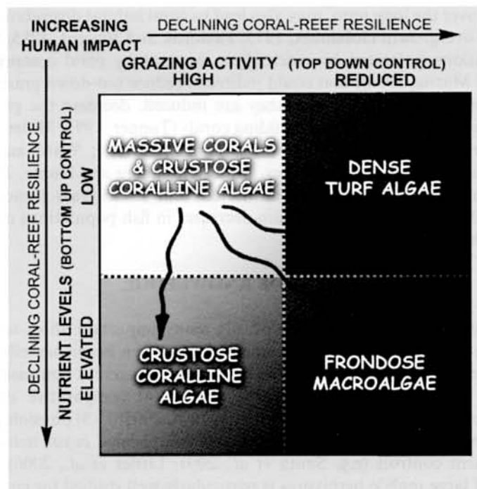
Figure 1. The competition-based Relative Dominance Model (modified from Littler and Littler, 1984a). All of the functional indicator groups occur under the conditions of every compartment of the model; however, the RDM predicts which group will most often dominate . Crustose coralline algae are posited to be competitively inferior and dominate mainly by default, i.e. where fleshy algae are removed by herbivores and some corals are inhibited by nutrients. The dotted lines approximate tipping points where declining herbivory and increasing nutrients reach critical levels that begin to reduce resilience to phase shifts. As a baseline for healthy coral-reef habitats, herbivore abundances and diversity should be high and palatable test plants should show at least a > 50\% \text{ loss} \cdot 6 \text{ h}^{-1} (i.e. < 6\text{-h} half-life) during a replicated series of mid-day in situ exposures. Nutrient tipping points (i.e. thresholds) have proven to be quite low and universal (i.e. \sim 0.1 \mu\text{M SRP} , \sim 1.0 \mu\text{M DIN} ), as corroborated (Bell, 1992, 1995; Lapointe et al. , 1993) by laboratory growth experiments, case studies for macroalgal overgrowth of coral reef communities, and in situ experimental nutrient enrichment research. Light to dark shading indicates declining desirability of each functional group from a management perspective. One vector can partially offset the other (e.g. high herbivory can delay the impact of elevated nutrients, or low nutrients may offset the impact of reduced herbivory). We further posit that latent trajectories (reduced resiliencies to phase shifts) can be activated or accelerated by large-scale natural stochastic disturbances such as tropical storms, cold fronts, warming events, diseases, and predator outbreaks. These are events from which coral reefs have recovered for millions of years in the absence of humans, but when tipping points remain surpassed, less-desirable stable states can persist.
