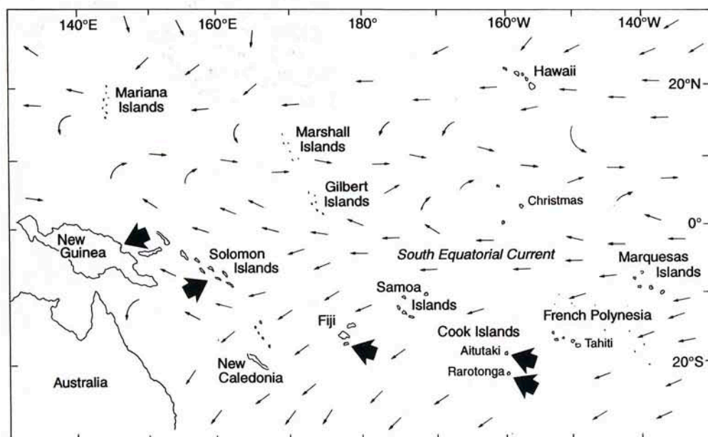
Fig. 1. Study areas (large arrows) and predominant South Equatorial Current system (small arrows). Drawing modified from (23).
