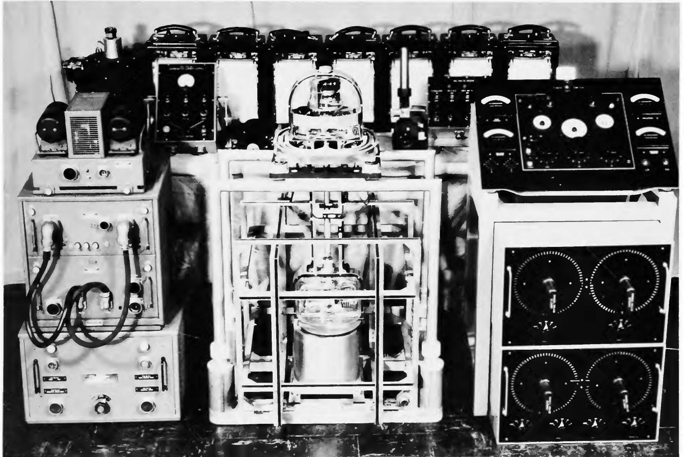
FIGURE 58.—No. 27, Magnetometer, Airborne, U.S. Naval Hydrographic Office, VAM-2B3, 1953.
