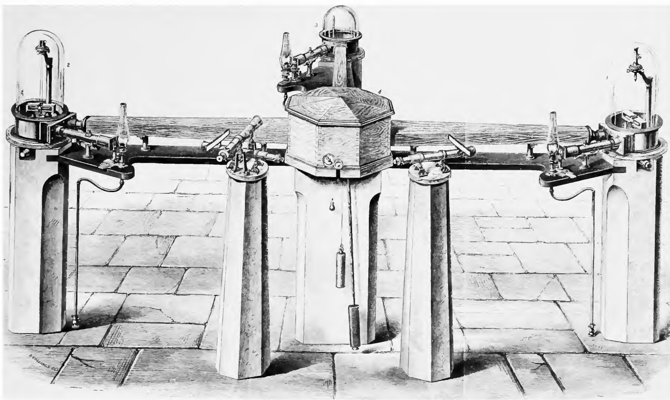
FIGURE 23.—Adie magnetograph. This photo-recording instrument, first described in 1859, was designed by J. Welsh at Kew Observatory and made by the London instrument-maker, Patrick Adie. It is similar, with improvements relating primarily to the photographic registration, to the Brooke magnetograph acquired by the Smithsonian in 1853. The latter no longer exists, but the present collection includes an Adie magnetograph acquired by the Coast Survey in 1882 (No. 8, Figure 36).
