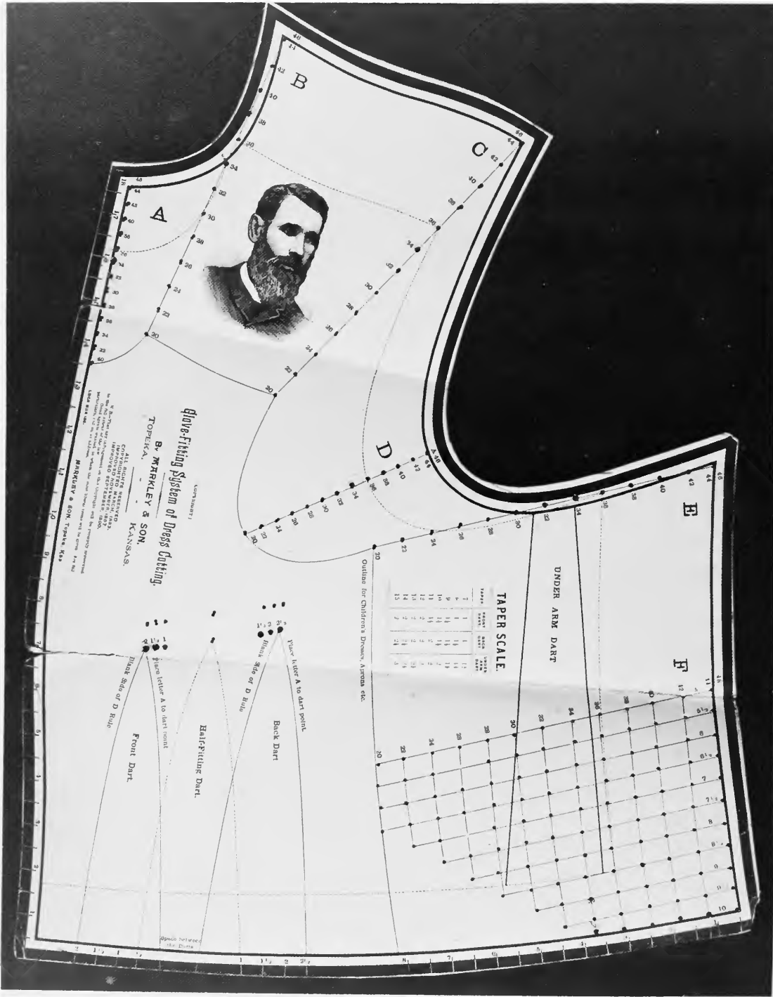
FIGURE 22b (below, right). "Dart Rule," combining a straight edge with an irregular curve.
