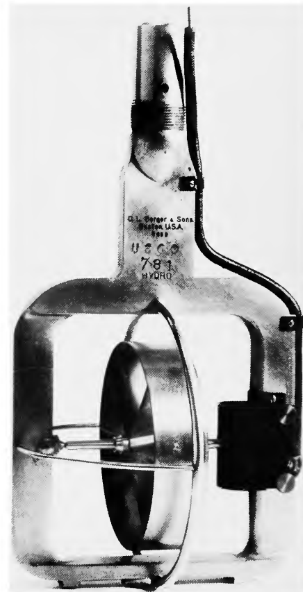
FIGURE 61.—A Fteley-Stearns current meter manufactured by C. L. Berger & Sons, Boston. (NMHT 330410, Smithsonian photo 75409.)
