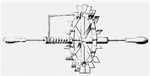
FIGURE 27.—Sir David and his paddle wheel type meter. (Portrait from Harper's Weekly, 11 April 1868; drawing from Ferguson, Lectures on Select Subjects .)
