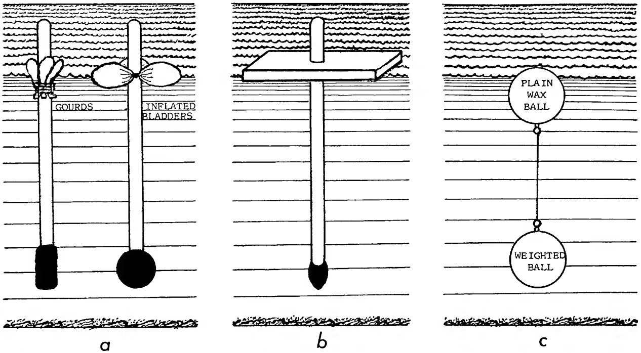
FIGURE 8.—Earliest floats post-dating Castelli's book on water velocities: a , Cabeo's rods, ca. 1646; b , Barattieri's rod float, ca. 1663; c , Mariotte's double float, ca. 1680. (Drawn by A. H. Frazier, from Masetti, "Descrizione.")
