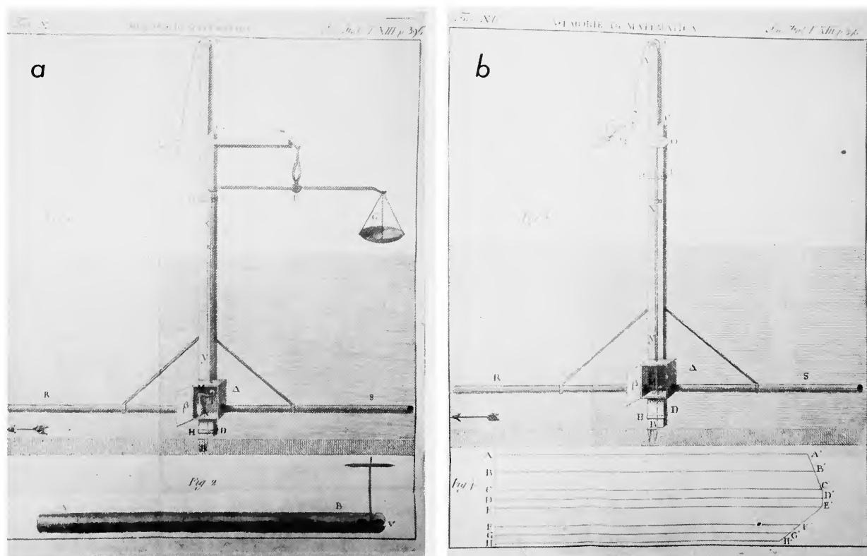
FIGURE 36.—Focacci's two current meters, 1806: a, balance scales are used to measure the force required to open the flap valve within the submerged box; b, pointer enables the operator to count and time the revolutions of the rotor within that instrument's box. Bottom of b is a vertical-velocity curve of the canal being studied, the earliest known publication of such a curve. (From Focacci, "Per Investigare la Celerita' Dell'Acque Correnti," page 396, plates 11, 12.)
