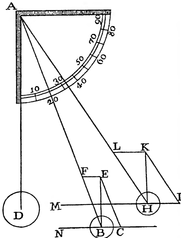
FIGURE 13.—Guglielmini’s “quadrant and ball,” ca. 1690. The force diagrams indicate the proportions one velocity bears to another. (From Guglielmini, Opera Omnia .)
