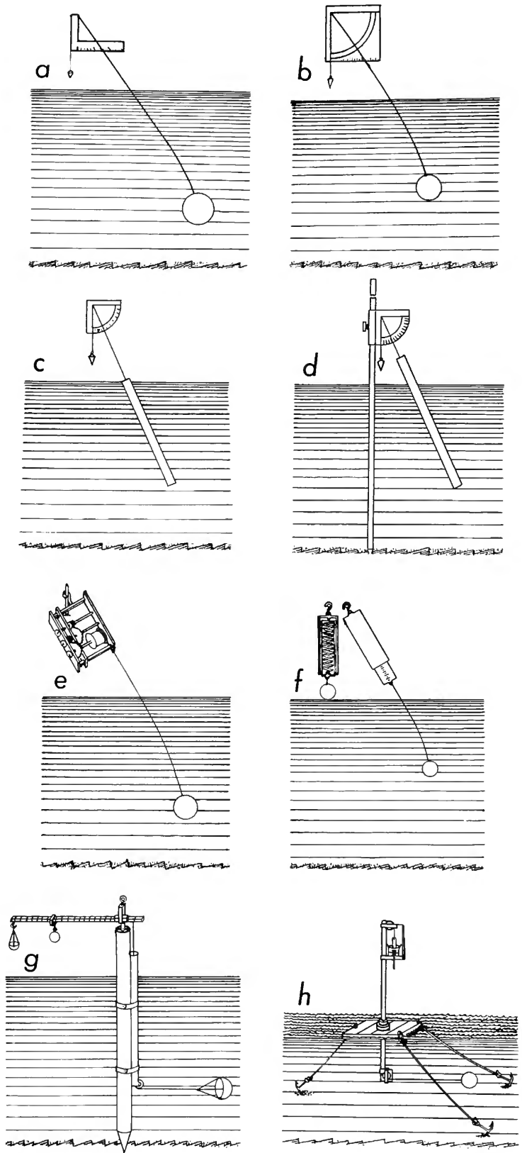
FIGURE 16.—Successors to Guglielmini's quadrant and ball: a, Cava's square, ca. 1721; b, Ximenes' quadrant, ca. 1752; c, Ferrari's sectional rod, ca. 1796; d, Venturoli's compound pendulum, ca. 1796; e Ximenes' clock-spring device, ca. 1752; f, Ximenes' spring-scale device, ca. 1752; g, Lorgna's device, ca. 1777; h, Barbantini's hydraulic counterweight, ca. 1814. (Redrawn by A. H Frazier after Masetti, "Descrizione.")
