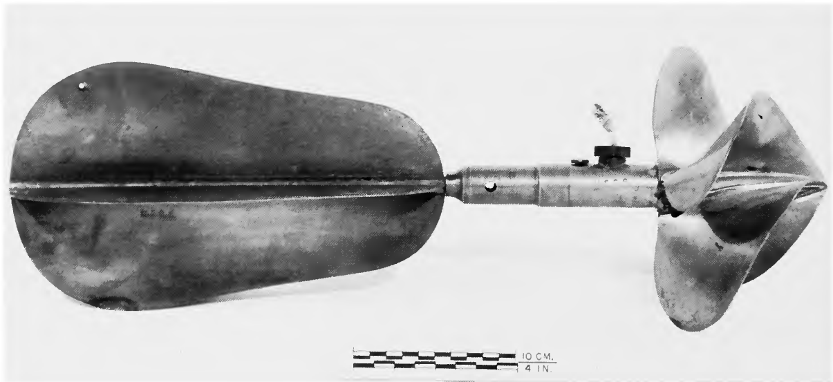
FIGURE 68.—A variation of the Haskell current meter as conceived in 1888-1889 by engineers of the U.S. Irrigation Survey. (NMHT 248697, Smithsonian photo 44537-B. )
