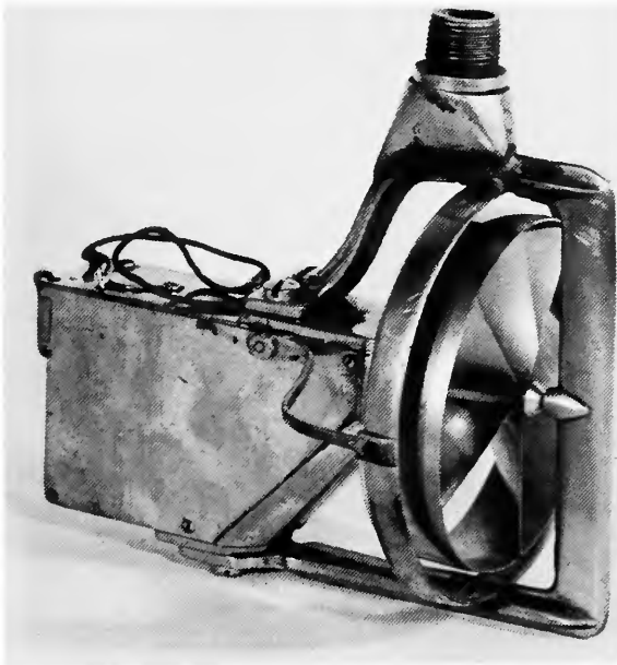
FIGURE 59.—A current meter contributed to the Smithsonian Institution by the Proprietors of Locks and Canals of Lowell, Massachusetts, which may be an experimental model designed by A. T. Safford. (NMHT 314771, Smithsonian photo 44536-C.)
