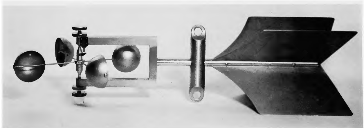
FIGURE 78.—Replica of Henry's cup-type, electric-contact current meter. (NMHT 317670, Smithsonian photo 72258.)
