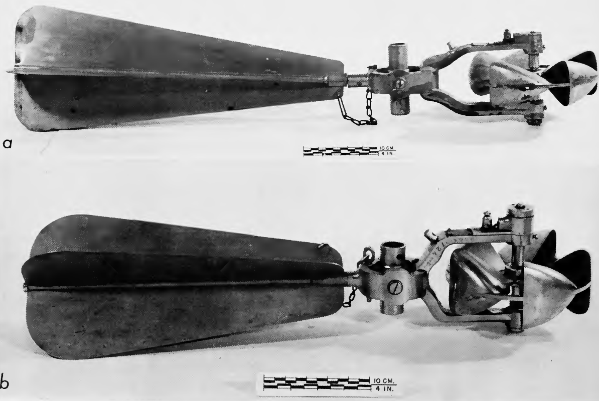
FIGURE 86.—Price's current meters, ca. 1886, manufactured by W. & L. E. Gurley: a , 34-inch-long version (NMHT 311708, Smithsonian photo 44538-D); b , 24-inch-long version (NMHT 289642, Smithsonian photo 44538-G).
