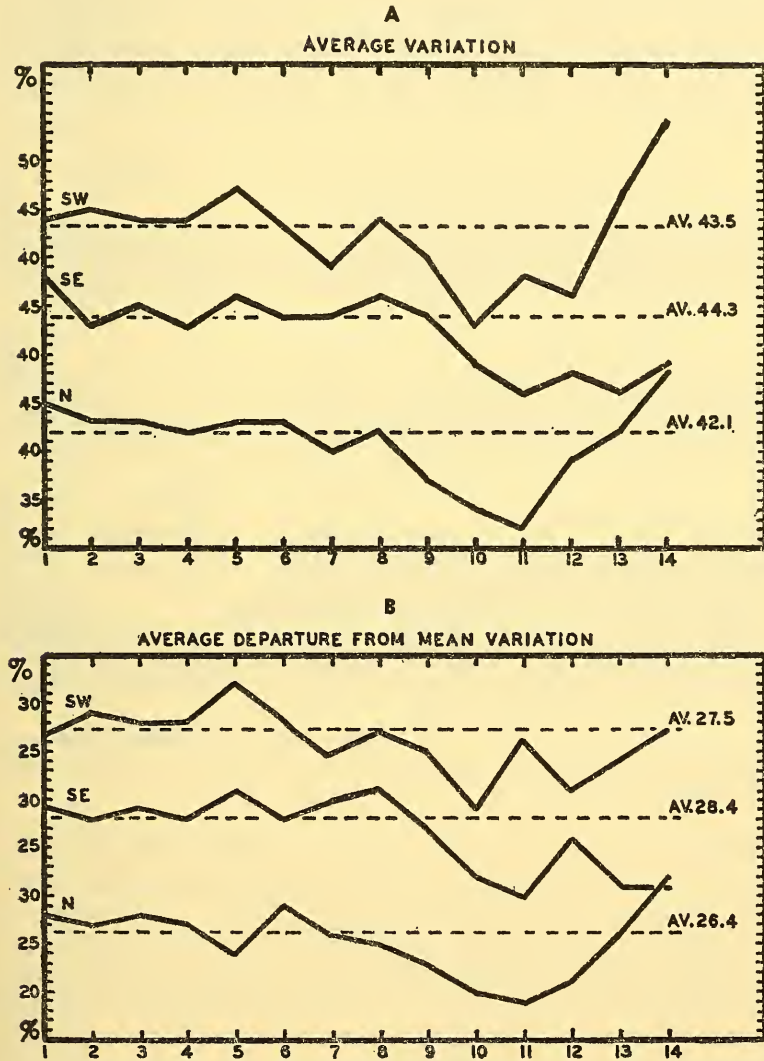
FIG. 30.—Circuit uniformity, OL-SO-57, three radii, all sections T-1 to T-14, Upper series shows average variation and lower shows average departure from mean variation.
