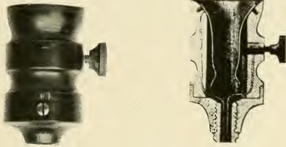
ORIGINAL SOCKET FOR INCANDESCENT LAMPS, 1880.
