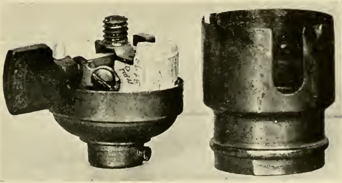
THOMSON-HOUSTON SOCKET.
