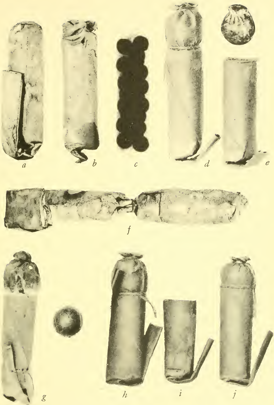
Plate 27.—CARTRIDGES FOR CALIBER 0.54 RIFLES AND HALL'S RIFLES: a , Buck and ball, French style, 1812-30; b , Buckshot, British style, 1812-30; c , X-ray of b , showing shot distributed through powder; d , ball, models 1804 and 1819 flint rifles; e , blank for same and patched ball; f , buckshot, British style, perhaps for cadet musket; g , ball, model 1819 Hall's rifle and bare ball used; h , ball, model 1841 percussion rifle (1849 Ordnance Manual); i , blank, same; j , ball, caliber 0.52 Hall's carbine (1849 Ordnance Manual).
