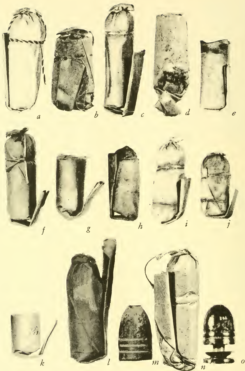
Plate 31.—PISTOL AND PISTOL-CARBINE CARTRIDGES: a , Ball, caliber 0.69, converted pistol; b , blank, caliber 0.69, British type, 1810-20; c , ball, caliber 0.54, model 1816-27 pistols; d , blanks, caliber 0.54, 1820-34; e , blank caliber 0.54, 1820-34; f , ball, caliber 0.54, for model 1819-36 pistols (1841 Ordnance Manual); g , blank, same; h , blank, same (1839 Ordnance Manual); i , ball, caliber 0.54, percussion, 1842; j , ball, same (1849 Ordnance Manual); k , blank, same; l , ball, caliber 0.58, pistol-carbine; m , elongated bullet for l ; n , William's patent bullet, for pistol-carbine; o , William's bullet from n .
