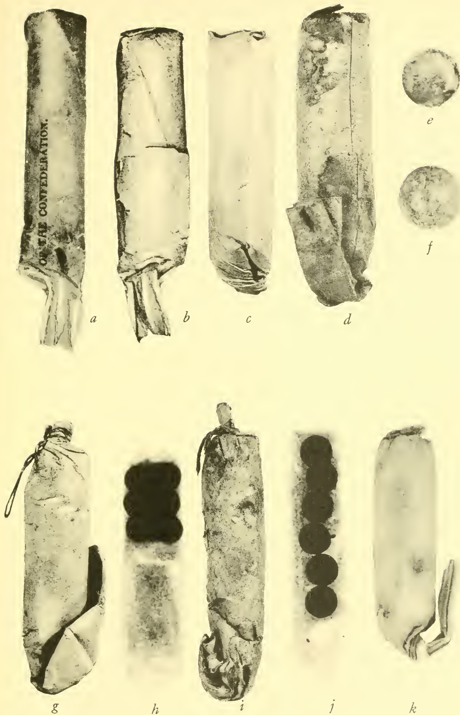
Plate 23.—CARTRIDGES FOR FLINTLOCK MUSKETS: a , Ball, French type, 1780; b , ball, French type, 1812; c , ball, French type, 1820-30; d , blank, French type, 1812 (blue paper); e , round ball, caliber 0.64, used in a , b , and c ; f , round ball, caliber 0.70, used in British musket; g , buckshot, British type, 1812-20; h , X-ray of g , showing 9 shot in 3 tiers i , buckshot, British type, 1780-1812; j , X-ray of i , showing 6 shot distributed through powder; k , blank, British type, 1812-20.
