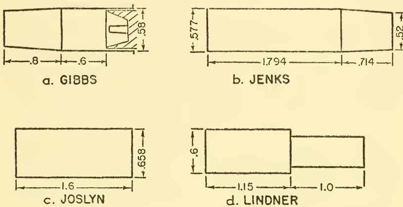
FIG. 17.—Carbine chambers.
