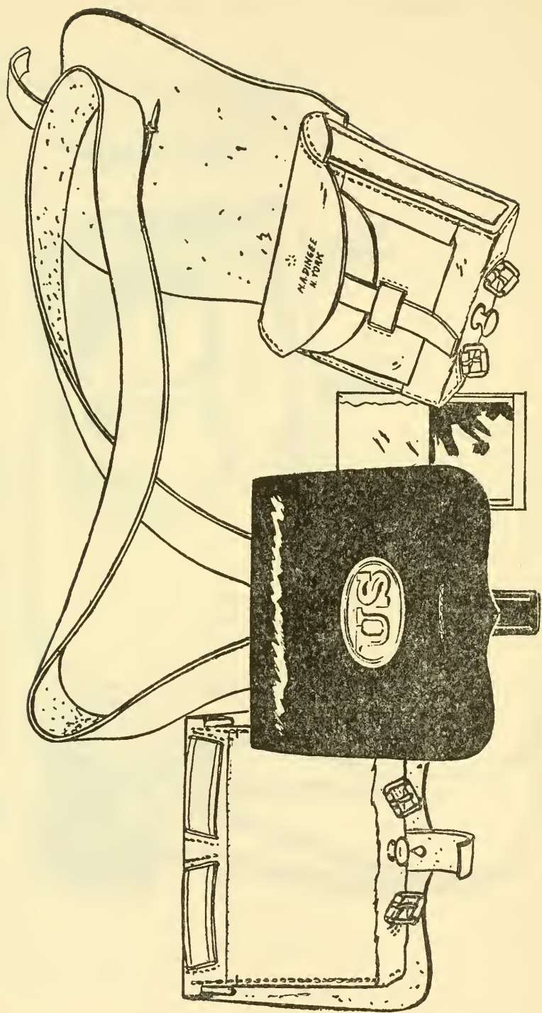
FIG. 12.—Cartridge box for Model 1842 percussion musket. (R. L. Miller.)
