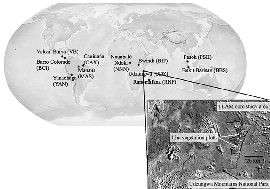
Figure 1 Map of TEAM sites used in this study: Bukit Barisan (BBS, Indonesia), Barro Colorado Island (BCI, Panama), Bwindi Impenetrable Forest (BIF Uganda), Caxiuana (CAX, Brazil), Manaus (MAS, Brazil), Nouabalé Ndoki (NNN, Republic of Congo), Pasoh Forest Reserve (PSH, Malaysia), Ranomafana (RNF, Madagascar), Udzungwa (UDZ, Tanzania), Volcán Barva (VB, Costa Rica), Yanachaga Chimillén National Park (YAN, Peru). Inset gives an example of the distribution of plots at the Udzungwa site.
