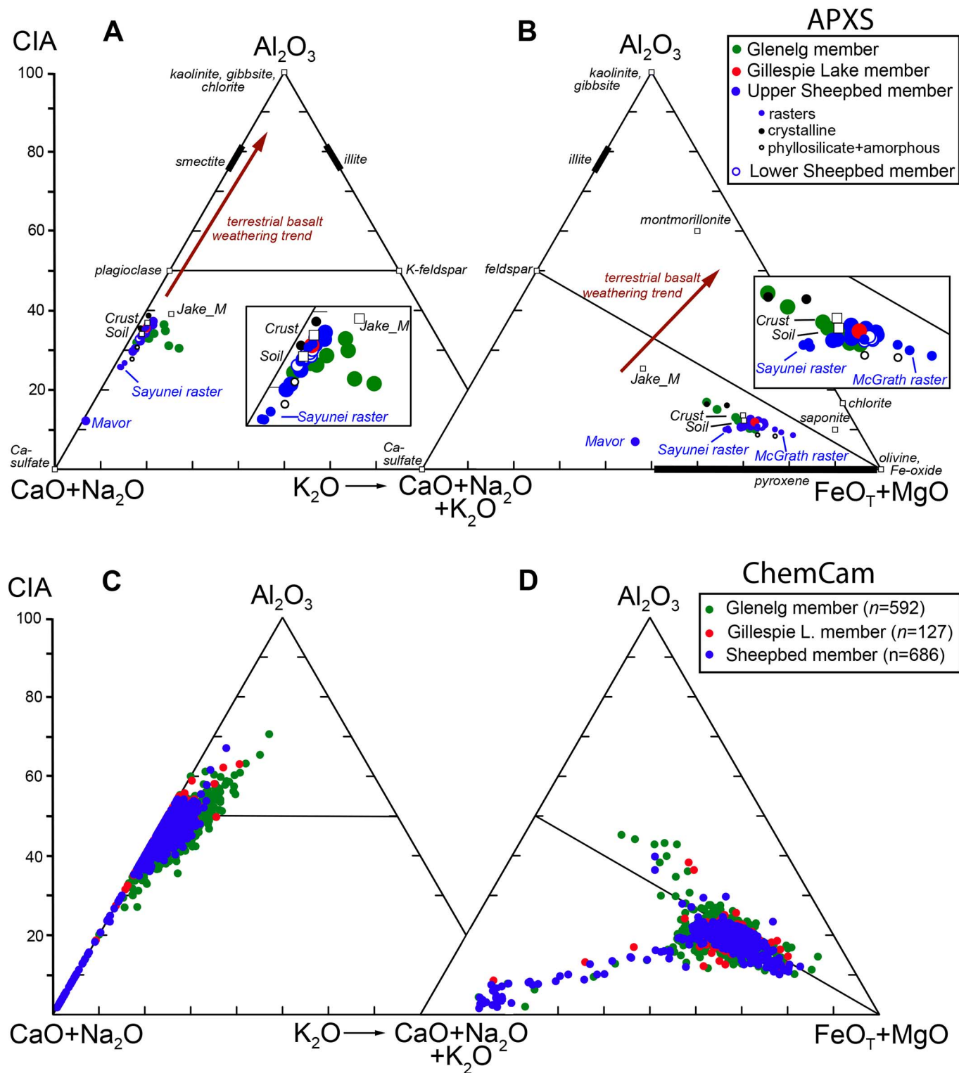
Fig. 2. Al 2 O 3 -(CaO + Na 2 O)-K 2 O and Al 2 O 3 -(CaO + Na 2 O + K 2 O)-(FeO T + MgO) ternary diagrams. (A and B) APXS data; (C and D) ChemCam data. Shown for reference are the CIA scale [measured on (A) and (C) only], and, as open squares, average martian crust (12), local soil (64), and the local rock
