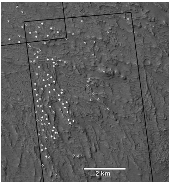
Fig. 11. Distribution of coarse-grained deposits on part of the Saheki K2 fan. These occurrences were mapped on 0.25 m/pixel HiRISE images PSP_007686_1575 (lower black outlined area) and PSP_006686_1580 (upper left black area). Mapping additionally included the remainder of these images and HiRISE image PSP_007899_1580 near the apex of the K2 fan (not shown). Visible coarse deposits and characteristic mottling or speckling in HiRISE images indicated by solid and hollow diamonds, respectively. These are interpreted as deposits of gravel just below the limit of resolution of individual boulders. Image base is CTX image P19_008545_1576 centered at 22.02 ^{\circ} S, 92.96 ^{\circ} E. (For interpretation of the references to color in this figure legend, the reader is referred to the web version of this article.)
