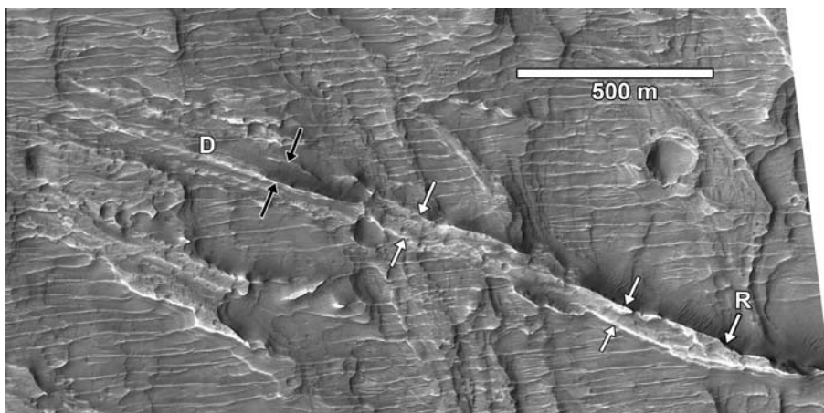
Fig. 6. Down-fan transition from a linear depression (D) through a U-shaped trough (delimited by black arrows) to a linear ridge (R) delimited by white arrows. Feature is interpreted as a fluvial channel with increasing degree of exposure and inversion down-fan due to increasing depth of aeolian deflation. Parallel ridges (black arrows) may be narrow natural levees. Part of \sim 3 m/pixel HiRISE image ESP_029788_1575, centered at 22.123^{\circ}\text{S} , 72.906^{\circ}\text{E} .
