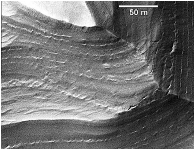
Fig. 14. Detail of thin, light-toned layers interbedded with thicker, massive layers (see Fig. 13 for context). Note the discontinuous appearance of the layers and indications of concave-upward layer cross-section. Part of HiRISE image PSP_007688_1575, centered at 22.008°S, 72.982°E.
