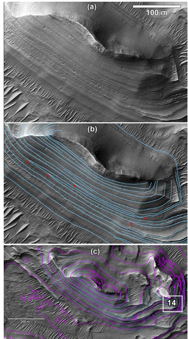
Fig. 13. Layered deposits exposed on slope below narrow ridge. (a) Exposed layers. Note thick, medium toned layers about 2–3 m thick separated by thin, light-toned layers with nodular or discontinuous presentation. (b) Interpretation of layering in (a), showing layer pinch-out locations indicated with an asterisk. (c) Contours from a 3 m/pixel DEM (pink) from HiRISE stereo pair PSP_7688_1575 and PSP_008545_1575 DEM superimposed on layer drawing. Ten meter contour interval. Note very shallow dip of layers broadly to the SE. Box at lower right indicates location of Fig. 14. Image scale is reduced in (c) relative to (a) and (b). Part of HiRISE image PSP_007688_1575, centered at 22.007°S, 72.975°E.
