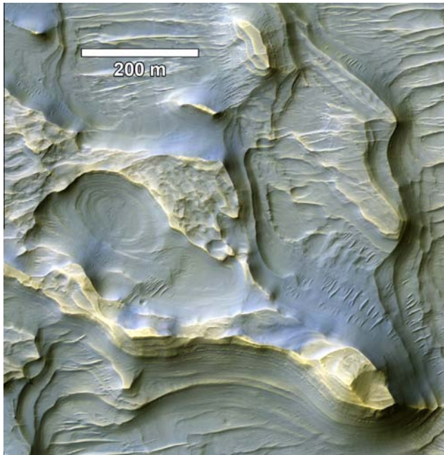
Fig. 4. Detail of inverted ridges and interbedded fine sediment exposed on subjacent slopes sediment capping ridge crests have yellowish cast relative to fine sediment. Fine aeolian sediment concentrated on north side of ridges has distinct bluish tone. Note scalloped indentations on ridge crests, presumably due to wind scour. Part of IRB color \sim 3 m/pixel HiRISE image PSP_007688_1575 centered on 22.092°S, 72.966°E, with colors stretched for clarity. Portions of low areas are occupied by TAR ridges. (For interpretation of the references to color in this figure legend, the reader is referred to the web version of this article.)
