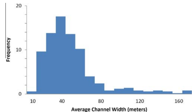
Fig. 12. Histogram of measured channel widths. Average width of segments is 38 m.
