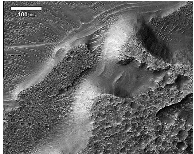
Fig. 17. Benches at two levels (see Fig. 16 for context). Note pitted surface, interpreted to be the result of impact gardening. The bench surface is mantled with coarse blocks, which are mass-wasted onto slopes at terrace edges. Fine, layered sediment that is largely conformable with overlying benches is exposed on slopes below benches. Benches are interpreted to be chemically-cemented lacustrine or playa deposits. Part of HiRISE image PSP_007688_1575.
