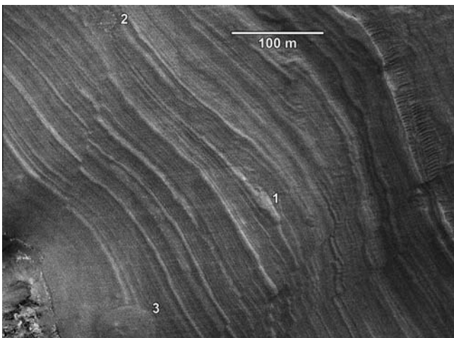
Fig. 15. Thick sequence of beds in eastern wall of a 5.3 km diameter crater superimposed onto fan deposits adjacent to Saheki central peak. Finest visible beds are ~2 m thick. Thicker blobs, as near “1” may be channel deposits. Circular features 2 and 3, obscuring bedding, may be scars of small impacts into interior crater wall. Note faulting in near left and right side of image, presumably due to impact deformation. Bottom of layer sequence at lower left of image where coarse crater floor or central peak materials are exposed. Image DN highly stretched to emphasize layering. Part of HiRISE image ESP_013226_1580, centered at 21.762°S, 73.046°E.
