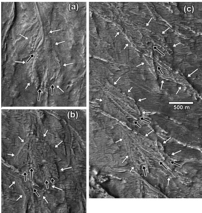
Fig. 8. Splay-like inverted platforms. White arrows show outer limits of splay. Ridges on surface of ridge suggest a spreading, possibly avulsive set of channels. Splays generally terminate down-fan in multiple finger-like ridges, separated by incised linear depressions (black arrows point upstream). All images at same scale. These structures are interpreted as fluvial deposits generally fed by a single channel upstream that spread into local depressions on the fan surface, or as autogenic transverse bars causing upstream deposition. Flows across the splay deposit eventually incise into the distal end of the deposit (black arrows). Images are part of \sim 6 m/pixel CTX image P14_006686_1579. (a) Centered at 21.927^\circ\text{S} 72.634^\circ\text{E} , (b) at 22.019^\circ\text{S} , 72.811^\circ\text{E} , and (c) at 22.141^\circ\text{S} , 72.863^\circ\text{E} .
