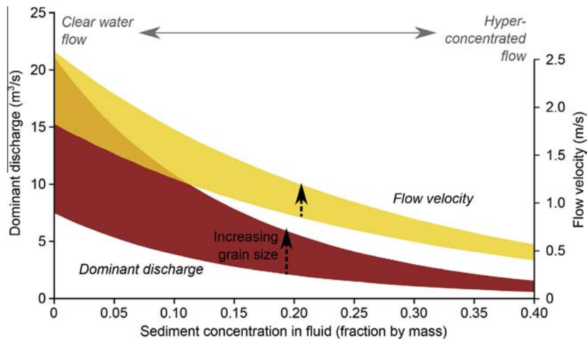
Fig. 31. Variability of calculated dominant discharges and associated flow velocities with sediment concentration in the fluid and grain size. The fields shown correspond to the effects of varying grain size across the interval 0.125 < D_{84} < 0.25 m, consistent with observations from HiRISE (Figs. 10 and 30); higher values of discharge and velocity are derived from the coarser grain sizes.
