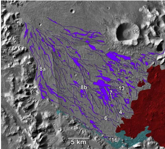
Fig. 3. Interpretive map of southern portion of the Saheki crater K2 fan and related features. The central peak and degraded interior rim are in the upper right and lower left, respectively. Also along the southern edge of the fan are slumps sourced from the crater walls which pre-date the fan material. Numbers indicate locations of additional figures. Purple lines and areas are raised ridges and platforms interpreted to be fluvial distributaries radiating from the fan apex at the upper left. Where the linear ridges or paired ridges are less than about 100 m in width they are shown as purple lines, but broader ridges and level platforms are portrayed as purple areas. Aeolian erosion has raised these into varying degrees of inverted relief. Red areas are crater floor materials interpreted to be megabreccia. Cyan features along southern margin of fan are flat-topped benches interpreted to be lacustrine or playa deposits contemporaneous with the fan. Uncolored areas on the fan are discontinuous distributaries and low areas partially mantled by transverse aeolian ridges (TARs). Mosaic of \sim 6 m/pixel CTX images P17_007543_1586, P19_008545_1576, and B09_007543_1586 centered at 21.96^\circ\text{S} , 72.81^\circ\text{E} .
