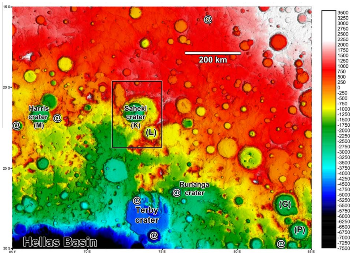
Fig. 1. Regional digital elevation location map of the northern Hellas rim. Image extends from 15°S to 30°S and 65°E to 85°E, Mercator projection. Letters in parentheses indicate crater designation in Moore and Howard (2005). “@” symbols show craters hosting fans identified by Kraal et al. (2008) and Wilson et al. (2007, 2013). Box shows location of Fig. 2. Topographic scale is in meters to Mars datum. North is up in this and all following figures (excluding photographs).
