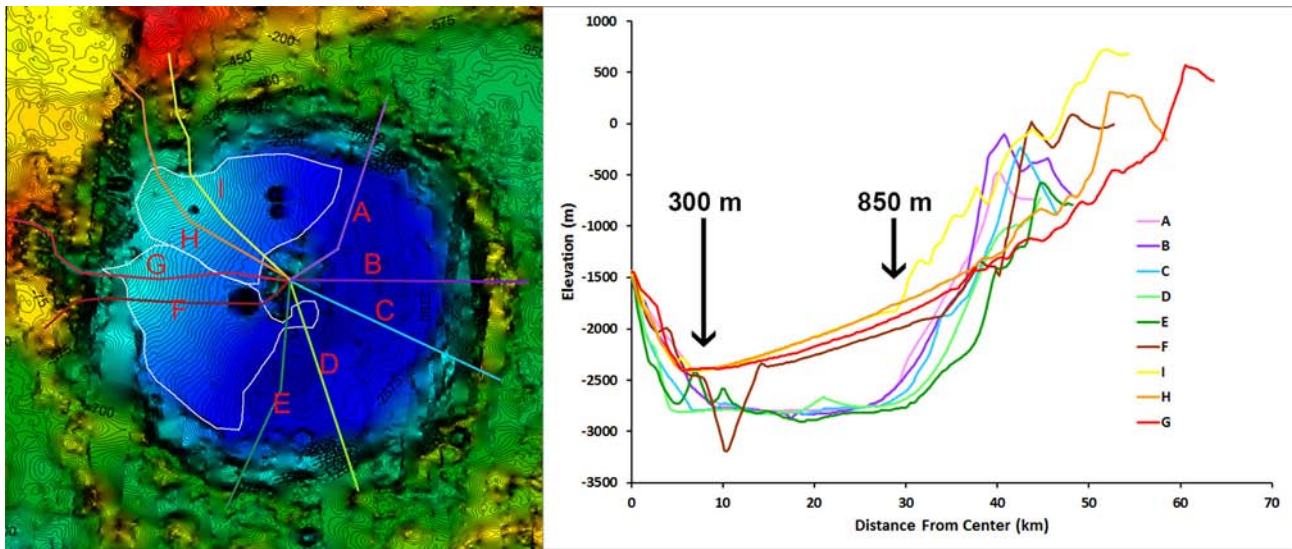
Fig. 5. Radial topographic profiles through Saheki crater. Saheki crater is approximately circular and the eastern half of the crater floor is nearly flat, making radial profiles A through E nearly coincident, whereas F to I cross the K1 and K2 fans permitting depth estimates assuming a symmetrical initial crater. Difference between the two sets of profiles provides an estimate of fan deposit thickness, reaching a maximum of about 850 m near the fan apices. Profiles H and I approximately follow the main valley axes of the source basins upstream from the K1 and K2 fans. Topography from interpolated MOLA PEDR data.
