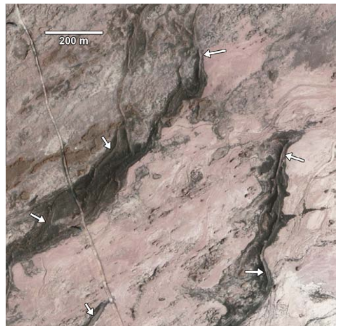
Fig. 24. Channels inverted by aeolian erosion. Arrows point to representative inverted channels. Dark coloration in vicinity of channels is granule deposits winnowed from the channel deposits. Inversion is due to coarser grain size of the channel deposits, protecting them from wind erosion and possibly chemical cementation. Note dirt track crossing image. Recent overbank deposits are pinkish. Older overbank deposits (upper left) are lightly mantled with winnowed granules as in Fig. 21. Maximum inverted channel relief 1–2 m. GeoEye imaging from Google Earth centered at 21.115°S, 69.576°W.
