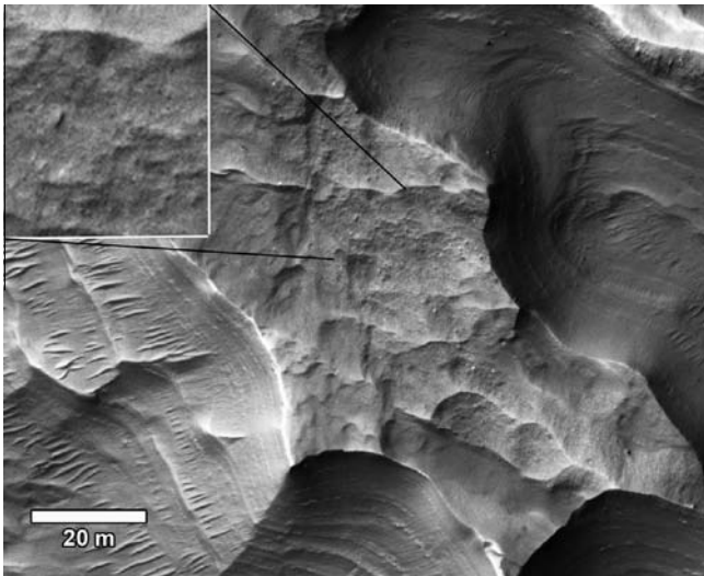
Fig. 10. Detail of inverted ridge showing gravelly sediment and wind scoured surface. Inset is magnified 3 \times . Layered sediments exposed on slopes below ridge. Part of \sim 3 m/pixel HiRISE image PSP_007688_1575 centered at 22.049 ^{\circ} S and 72.944 ^{\circ} E.
