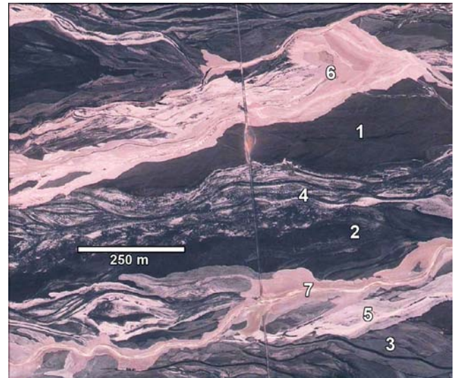
Fig. 26. Complex history of distributary history on part of a fan surface. Numbers indicate sequence of fan activity (1 is oldest). Note that flow 7 has covered the railroad track crossing the image. Inactive parts of fan become darker due to progressive mantling by granule ripples derived from overbank deposits. GeoEye imaging from Google Earth centered at 20.75°S, 69.40°W, taken prior to the 2012 flood deposition.
