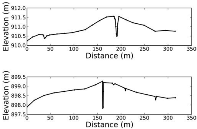
Fig. 28. Surveys across channel and overbank deposits of distributary shown in Fig. 20, showing broad natural levees. Top cross section centered on 21.093°S, 69.478°E, bottom cross section centered on 21.100°S, 69.490°E. The bottom of the channel in the top survey is higher than the surrounding fan surface. Note 25× vertical exaggeration.
