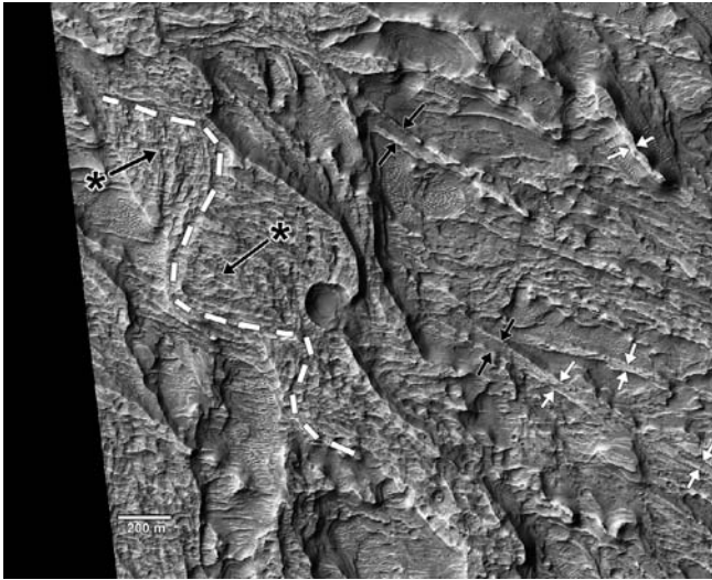
Fig. 7. Flat platforms on the K2 fan. We interpret the ridges to be mantled with gravely sediment deposited by low-sinuosity meandering or braiding streams during deposition. An interpreted meander bend is shown by dashed white lines, and possible point-bar deposits interior to the bend occur near the asterisks, with black arrows pointing in the direction of inferred meandering. Paired white arrows on right hand of image shows ridges representative of those sampled to determine original widths. Paired black arrows show paired narrow ridges interpreted to be natural levees exposed through partial aeolian distributary exposure. Part of \sim 3 m/pixel HiRISE image PSP_007588_1675, centered at 22.016^\circ\text{S} and 72.936^\circ\text{E} .
