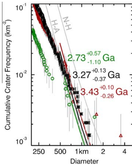
Fig. 19. Crater age determination plots. N–H and H–A indicate Noachian–Hesperian and Hesperian–Amazonian boundaries. Absolute age determination used craters greater than 500 m in diameter to avoid errors arising from aeolian erosion (see text for discussion). Red: K1 fan. Black: Aggregate of four fans in “L” Crater. Green: K2 fan. The young age and large error bars for the K2 fan can likely be attributed to high amount of aeolian modification. (For interpretation of the references to color in this figure legend, the reader is referred to the web version of this article.)
