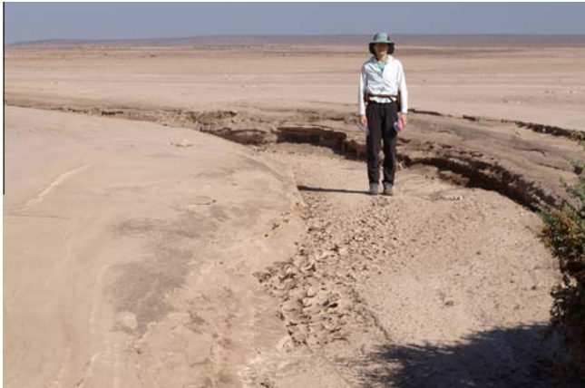
Fig. 21. Fan distributary, showing fine-grained cohesive banks and extensive overbank deposits. Bank crest to bank crest about 3 m. Photo by A. Howard. Location at about 21.097°S, 69.486°W.
