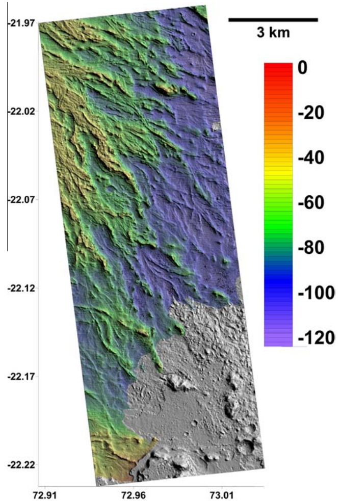
Fig. 9. Shaded relief image of the distal end of the Saheki K2 fan from \sim 3 m DEM constructed from HiRISE stereo image pair PSP_7688_1575 and PSP_008545_1575, centered at 22.10^\circ\text{S} , 72.97^\circ\text{E} . A plane fit to the overall dip ( 0.03 ESE) and strike (NNE) of the fan surface was subtracted from the DEM, and elevations (in meters) relative to that plane are indicated in color shading. Portions of the fan surface at approximately equal stratigraphic level have the same relative elevation. This indicates that the depth of aeolian erosion increases towards the distal end of the fan, which is accordant with higher ridge inversion near the distal end of the fan. Axis labels in degrees North and East. Portions of image not mantled with fan deposits are uncolored.
