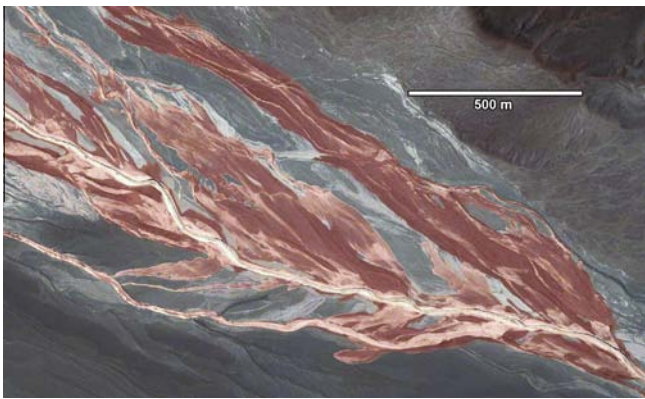
Fig. 22. Atacama fan flood deposits. Red-toned deposits deposited by an early 2012 flood sourced from the Andes foothills to the east. Deposits radiate from the end of an entrenched channel section at left boundary. Broad sheet deposits source from overflow of main distributary channels. Earliest deposits are darkest red, with later overflows and channelized flow being lighter pink. Main distributary averages about 12 m wide. Flooding and sediment deposition continued for 25 km downstream, spanning the length of the alluvial fan. Center of image at 20.765°S, 69.311°W. North is up. Iconos 0.8 m/pixel image, taken 12/27/2012. (For interpretation of the references to color in this figure legend, the reader is referred to the web version of this article.)
