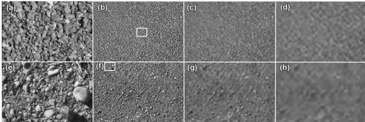
Fig. 30. Effect of image resolution on interpretation of gravel deposits. Images (a and e) are snippets from larger images of gravelly sediment. Sediment in (a) is well-sorted gravel and in (e) is poorly sorted. Images (b and f) show reduced resolution of full images in which the particles representative of about the 84th percentile size are shown at 2 pixels per particle (for full resolution HiRISE images this would correspond to 50 cm particles). Location of snippets in (a and b) are shown as white boxes in (b and c), respectively. In (c and g) resolution is further reduced to 1 pixel per particle, and to \frac{1}{2} pixel per particle in (d and h). In reduced resolution images gravel shows a characteristic mottled texture. Note that scale was not provided for original images. Source for original illustrations: http://www.texturemate.com/content/free-gravel-texture-19-11-2011-001 (a–d) http://aquaponics.wiki.com/wiki/gravel?file=Gravel_small_stones.jpg (e–h).
