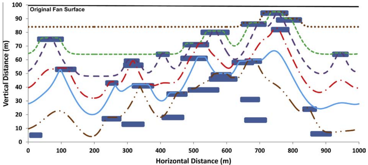
Fig. 29. Interpretive model of aeolian fan erosion in Saheki crater. A hypothetical along-strike cross section of the fan is pictured, with white being fine-grained, wind-erodible overbank sediment, and blue being randomly seeded channel gravels. Wind erosion starts from the black horizontal upper surface and colored profiles show successive stages of modeled wind erosion. See Section 3.2.1 in text and Appendix A for further discussion. (For interpretation of the references to colour in this figure legend, the reader is referred to the web version of this article.)
