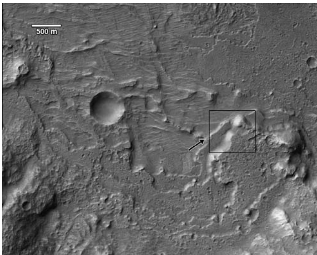
Fig. 16. Flat-topped benches at boundary between southern K2 fan deposits and Saheki crater wall. Note multiple levels and irregular terrace edges. Arrow points to location where inverted fan ridge may be at the same elevation at the adjacent terrace. Box shows location of Fig. 17. Part of CTX image P19_008545_1576_XI_225287W centered at 22.216°S and 72.946°E.
