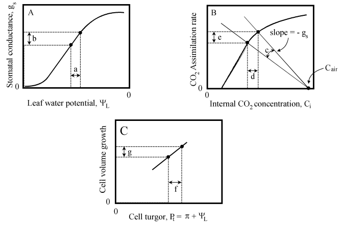
Fig. 2A–C The graphs in Fig. 1 are repeated showing how a change in hydraulic resistance causes a change in various parameters given by double-headed arrows. A An increase R_{plant} causes a decrease in \Psi_L (a). The decrease in \Psi_L causes a decrease in g_s (b). B A decrease in g_s causes a decrease in the slope (c) which causes a decrease in C_i (d) and a decrease in assimilate rate (e). C A decrease in \Psi_L causes a decrease in turgor of growing cells (f) which causes a decrease in cell volume growth rate (g)
