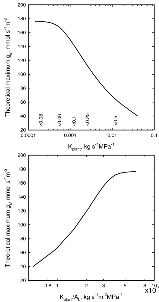
Fig. 5 Upper: Theoretical relationship between maximum possible stomatal conductance, g_s , and whole plant hydraulic conductance is plotted using the measured relationships for A. saccharum in Figs. 3 and 4. The whole plant conductance values on the x -axis correspond to basal stem diameters of 0.022–1.22 m and stem diameters in m corresponding to specific plant conductances are indicated on the x -axis. See text for computational details. Lower: Theoretical relationship between g_s is plotted versus whole plant conductance per unit leaf area: k_{\text{plant}}/A_L
