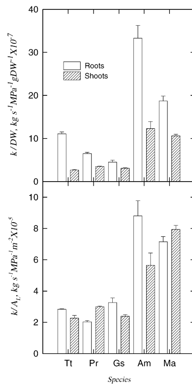
Fig. 8 Hydraulic conductances of shoots and roots scaled to dry weight or leaf-area. Upper : k_r per unit TRDW and k_{\text{sh}} per unit shoot dry weight. Lower : k_r and k_{\text{sh}} both scaled to leaf-area ( A_L ). Error bars are SEM, n=23-36 . Data from all collection dates combined. Species abbreviations as in text. Root and shoot means for Am and Ma were significantly different from corresponding root and shoot means for Tt, Pr and Gs in both A and B (Tukey test, P \leq 0.05 ). (from Tyree et al. 1998)
