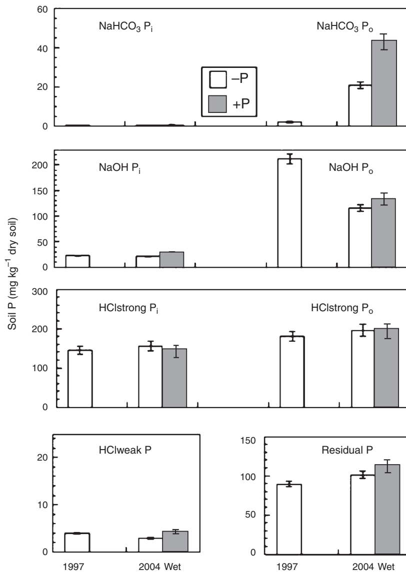
Fig. 2. Soil phosphorus fractions (mean \pm standard error) determined by the Hedley sequential fractionation procedure for subsurface soils (30–45 cm depth interval) in plots with (+P) and without (-P) phosphorus in the nutrient addition experiment on Gigante Peninsula, Panama.
