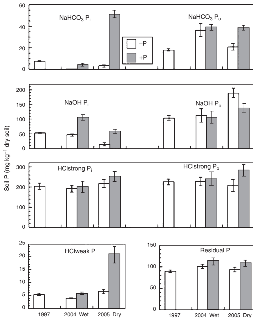
Fig. 1. Soil phosphorus fractions (mean \pm standard error) determined by the Hedley sequential fractionation procedure for surface soils (0–15 cm depth interval) in plots with (+P) and without (-P) phosphorus in the nutrient addition experiment on Gigante Peninsula, Panama.
