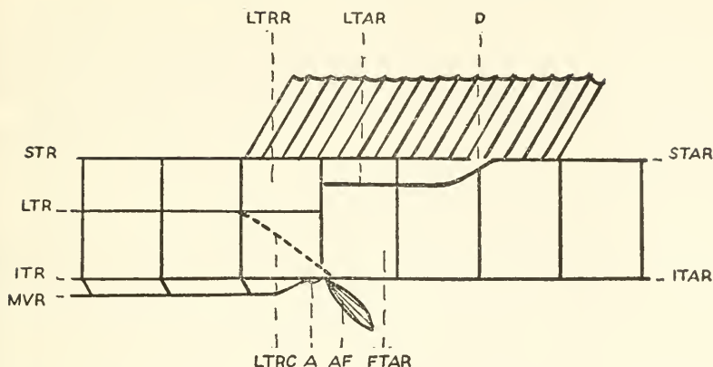
FIGURE 36.—Diagram of the middle part of the body of a hypothetical syngnathid illustrating the terms used in describing this family: (A) anus; (AF) anal fin; (D) discontinuous part of superior tail ridge; (FTAR) first tail ring; (ITAR) inferior tail ridge; (ITR) inferior trunk ridge; (MVR) midventral abdominal ridge; (LTAR) lateral tail ridge; (LTR) lateral trunk ridge; (LTRC) lateral trunk ridge continuous with inferior tail ridge; (LTRR) last trunk ring; (STAR) superior tail ridge; (STR) superior trunk ridge.
