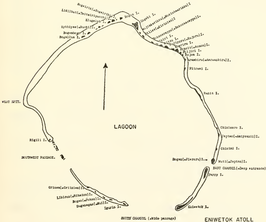
FIGURE 2.—Map of Eniwetok Atoll.
