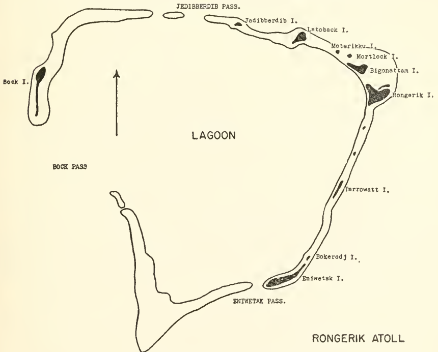
FIGURE 4.—Map of Rongerik Atoll.
