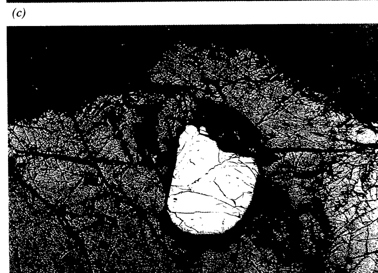
Fig. 3. Photomicrographs of oldhamite and included phases in the Bustee pyroxene-oldhamite clast. (a) A rounded oldhamite spherule which was sheared by a later shock event. Field of view = 2.6 mm. (b) Large (120 \mu\text{m} ) isolated osbornite within host oldhamite. Within the oldhamite, lath-shaped troilite oriented along the crystallographic axes of the host oldhamite can be seen. It appears that this troilite formed by exsolution from the host oldhamite. Field of view = 650 \mu\text{m} . (c) Large (300 \mu\text{m} ), rounded to subhedral, isolated titaniferous troilite within oldhamite host. The oldhamite-silicate boundary is visible at the top of the image. This grain of troilite contains 23.3 wt% titanium. It likely represents an immiscible Fe-rich sulfide melt which crystallized slightly after the Ca-rich sulfide melt in which it is enclosed. Field of view = 1.3 mm.
