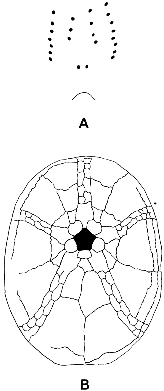
FIGURE 9.— Eurhodia rugosa (Ravenel) ideali , new subspecies: A, phyllode of ambulacrum III on USNM 264589 from Castle Hayne Limestone at locality 12, \times 8 ; B, adoral plate arrangement of USNM 264589 from Castle Hayne Limestone at locality 12, \times 2 .
