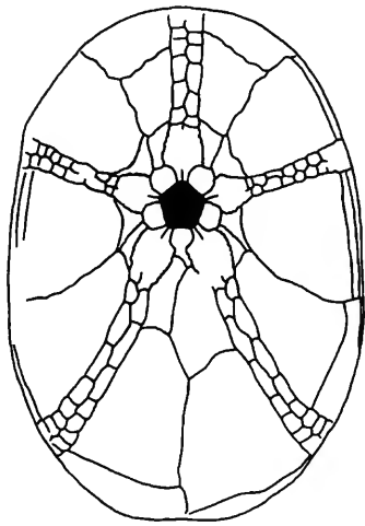
FIGURE 10.— Eurhodia rugosa (Ravenel) depressa , new subspecies: A, floscelle of USNM 264590 from Castle Hayne Limestone at locality 10, \times 3 ; B, adoral plate arrangement of USNM 264591 from Castle Hayne Limestone, locality 10, \times 1 .
