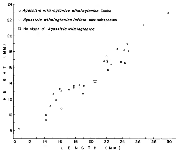
FIGURE 19.—Scattergram showing height of two subspecies of Agassizia wilmingtonica Cooke.
