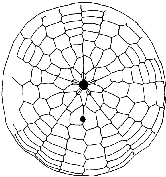
FIGURE 17.— Periarctus byelli (Conrad), adoral plate arrangement in USNM 264596 from Castle Hayne Limestone at locality 12, \times 2 .
