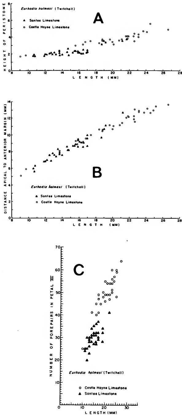
FIGURE 13.— Eurhodio holmesi (Twitchell): A, scattergram showing lack of difference in height of peristome between Santee Limestone and Castle Hayne Limestone specimens; B, scattergram showing lack of difference in position of apical system between Santee Limestone and Castle Hayne Limestone specimens; C, scattergram showing lack of differ-
