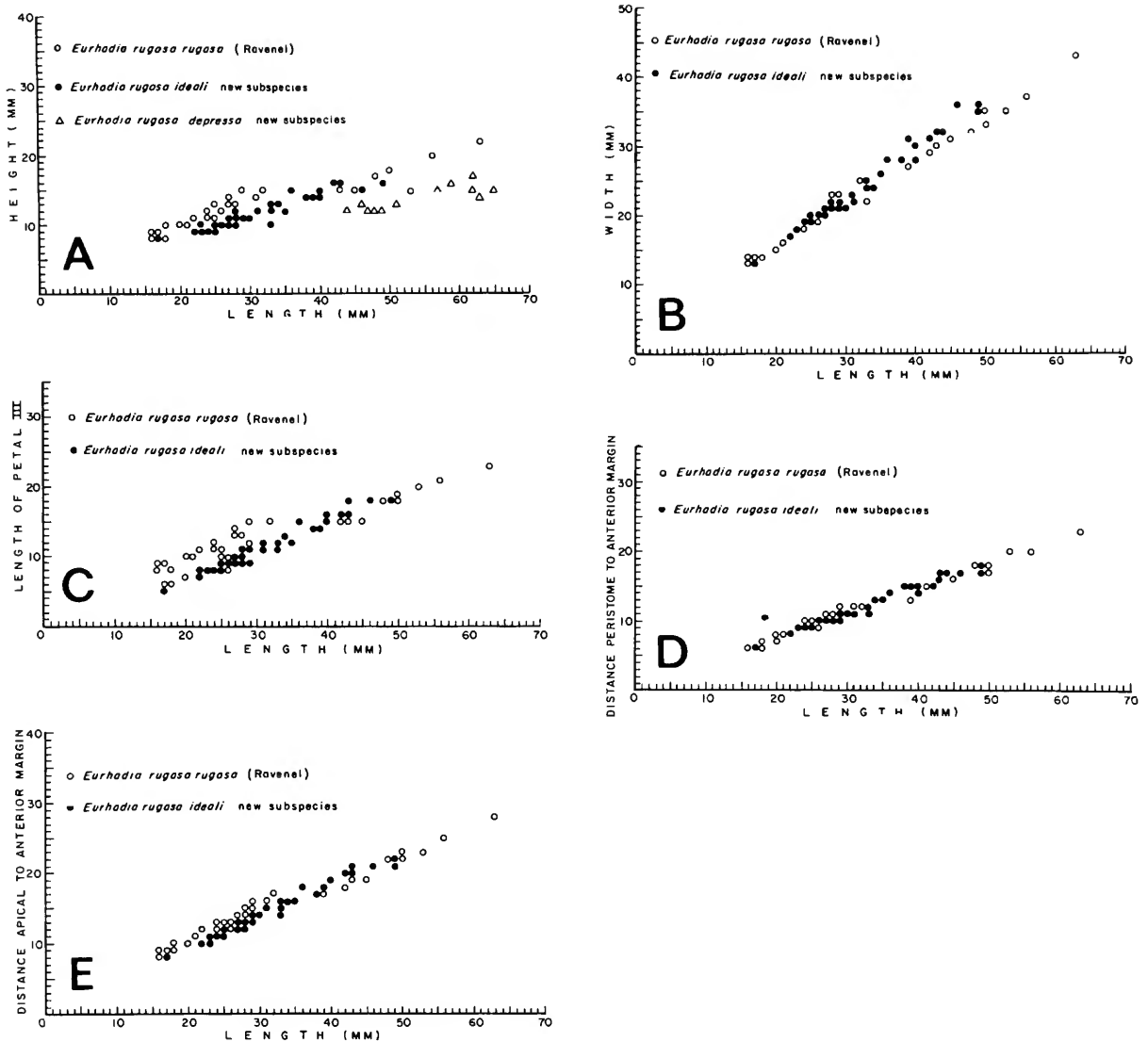
FIGURE 7.— Eurhadia rugosa (Ravenel): A, scattergram showing differences in height relative to length in three subspecies; B, scattergram showing difference in width relative to length in two subspecies of E. rugosa (Ravenel) (note that although width is similar in the smaller specimens, larger specimens of E. rugosa ideali , new subspecies, are narrower than large specimens of E. rugosa rugosa (Ravenel)); C, scattergram showing difference in length of petal III in two subspecies of E. rugosa (Ravenel) (note that although length of petal III is greater in small specimens of E. rugosa ideali , new subspecies, than in E. rugosa rugosa (Ravenel), this difference is absent in larger specimens); D, scattergram of subspecies of E. rugosa (Ravenel) showing similar position of peristome; E, scattergram of subspecies of E. rugosa (Ravenel) showing similar position of apical system in larger specimens.
