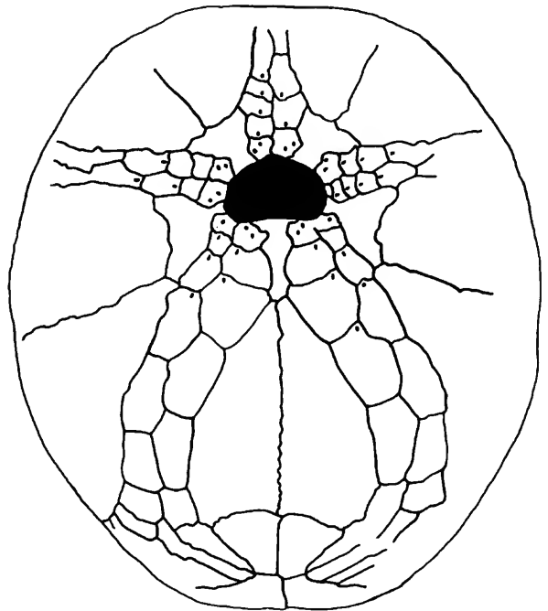
FIGURE 26.— Eupatagus wilsoni , new species, adoral view of holotype USNM 264084 from Castle Hayne Limestone at locality 12, \times 1.5 .
