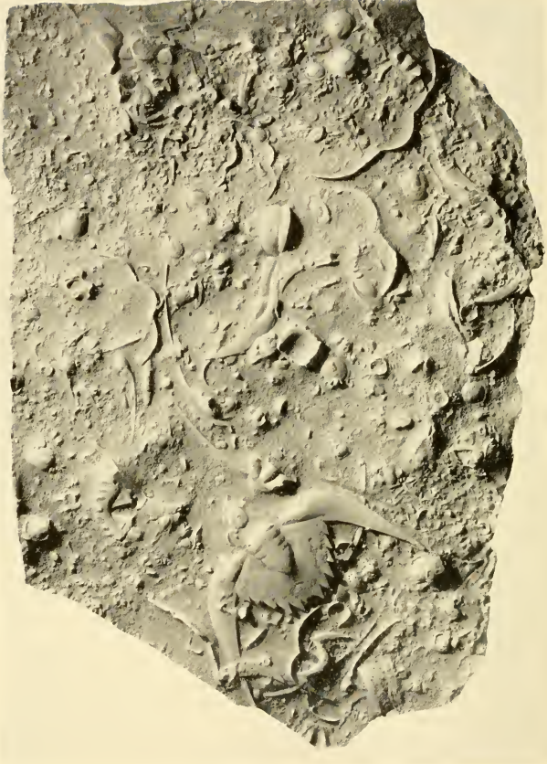
Cream-colored limestone slab, of Middle Cambrian age, from China, containing many fossils. The Chinese make ornamental caskets from such slabs, and these were the means of bringing the fossils to the attention of European scientists
