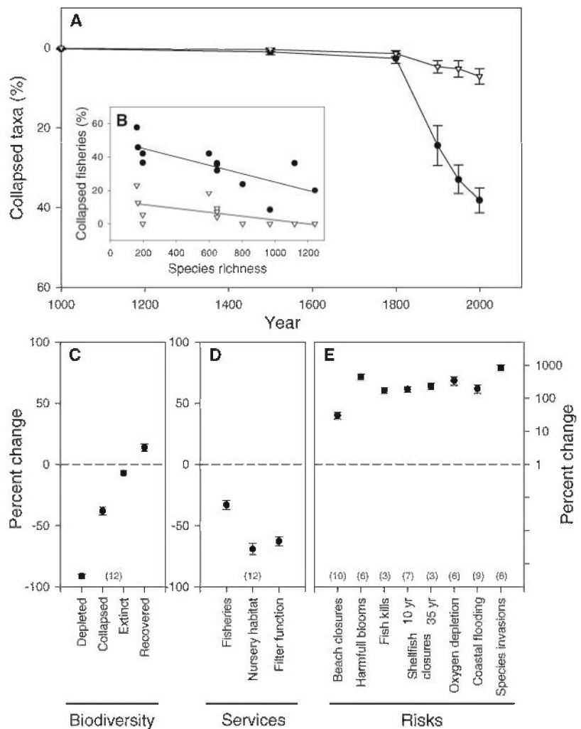
Fig. 2. Regional loss of species diversity and ecosystem services in coastal oceans. (A) Trends of collapse (circles, >90\% decline) and extinction (triangles, 100\% decline) of species over the past 1000 years. Means and standard errors are shown ( n = 12 regions in Europe, North America, and Australia). (B) Percentage of collapsed (circles) and extinct (triangles) fisheries in relation to regional fish species richness. Significant linear regression lines are depicted ( P < 0.01 ). (C to E) Relative losses or gains in (C) biodiversity, (D) ecosystem services, and (E) risks that are associated with the loss of services. The number of studies is given in parentheses; error bars indicate standard errors.
