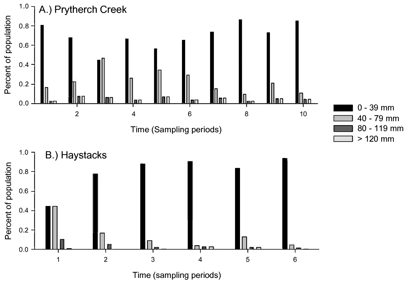
Figure 2. Proportional abundance of four size classes of blue crabs in both Prytherch Creek (A) and Haystacks (B) study sites for each sampling period. The duration between sampling periods averaged 4 d for Prytherch Creek and 7.8 d for Haystacks.
