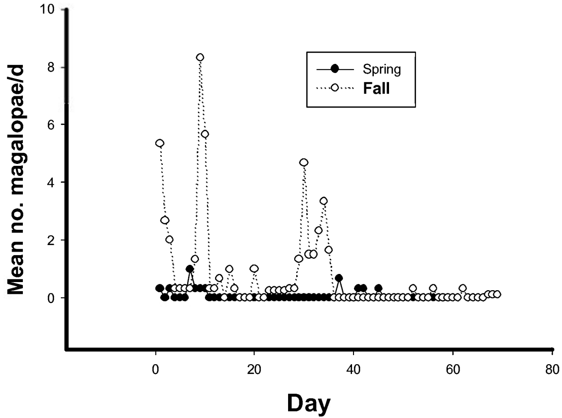
Figure 20. The relative abundance of blue crab megalopae collected on floating, artificial settlement substrates (N = 3) moored on the US Coast Guard dock at Oregon Inlet, NC. During Spring, artificial settlement substrates were checked daily from April 8-June 4, 2002. During late summer-early Fall, artificial substrates were checked daily from August 1-October 31, 2002 (from D. Eggleston, unpubl. data).
