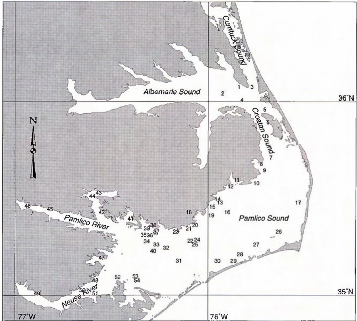
Figure 5. Locations of trawl survey core sampling stations for adult blue crabs conducted by the North Carolina Division of Marine Fisheries (NC DMF Program 195). See Table 3 for the water body and sampling area for a given station number.
