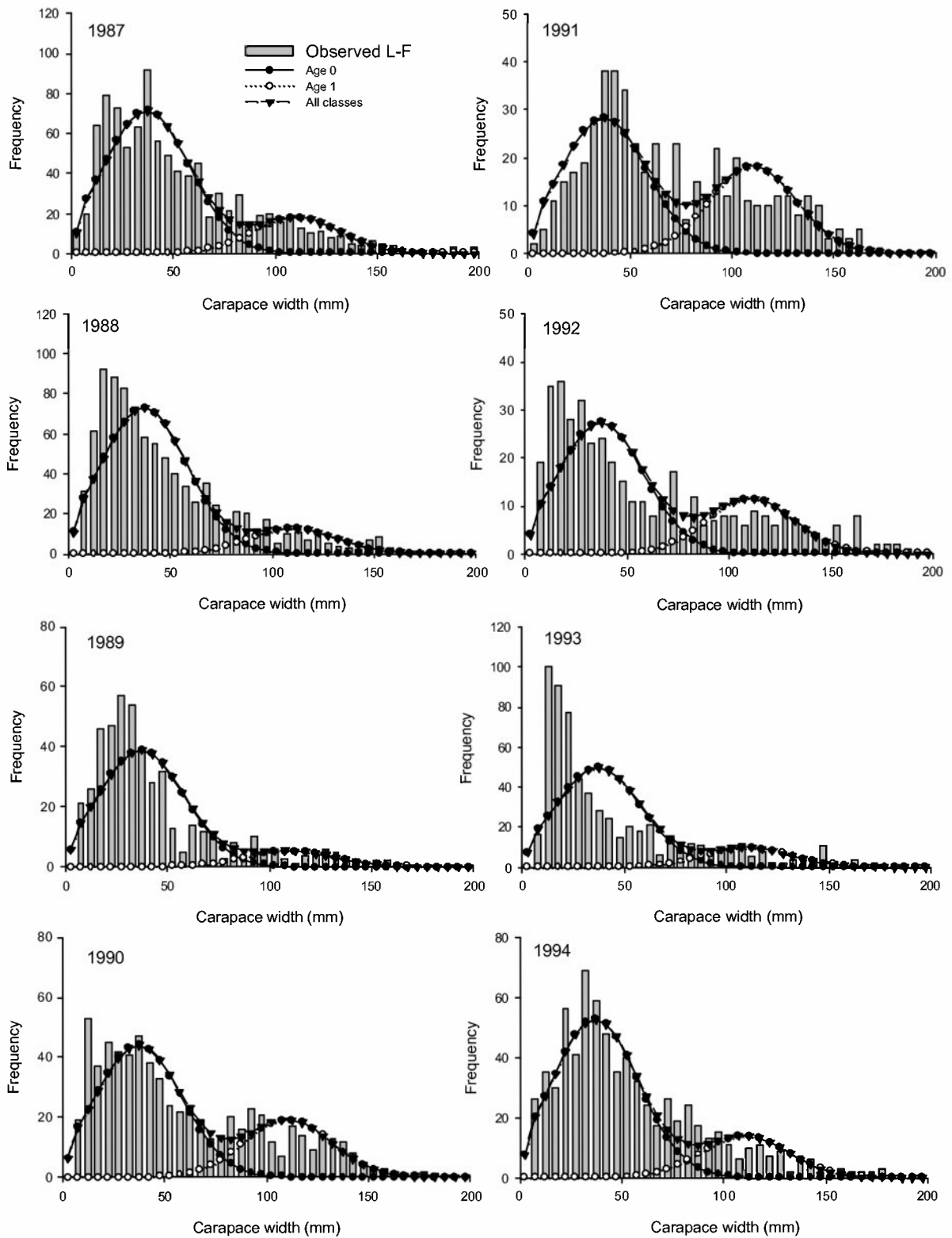
Figure 8. The observed (histograms) and predicted (symbols) size frequency of blue crabs by year collected in NC DMF Program 120 in June from 1987–2002 pooled across all water bodies. The predicted fits shown were produced by minimizing a log-likelihood length-based model.
