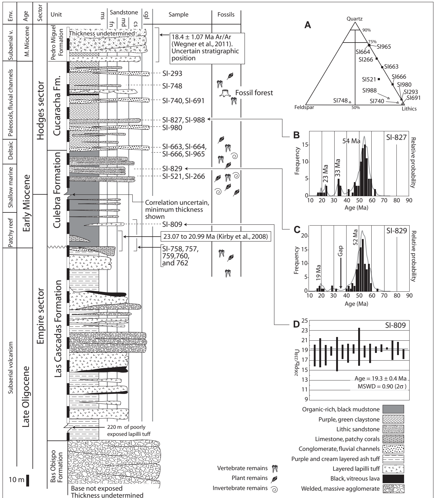
Figure 8. Stratigraphic column measured in surface exposures along the Panama Canal. (A) QFL (quartz, feldspar, lithics) composition diagram for Culebra and Cucaracha arenites; (B–C) U/Pb ages in detrital zircons recovered from Cucaracha and Culebra Formations, respectively; and (D) U/Pb ages in magmatic zircons recovered from a felsic tuff near the base of the Culebra Formation. MSWD—mean square of weighted deviates. See Table 1 for sample coordinates and GSA Data Repository for sample descriptions and coordinates (see text footnote 1).
