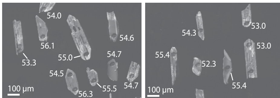
Figure 4. ^{238}\text{U}/^{206}\text{Pb} weighted average age plots of zircons extracted from granitoids in central Panama. Below: Cathodoluminescence images of sample SI-1049 showing an example of the location of magmatic zircon tip analyses. MSWD—mean square weight deviation. See Table 1 for sample summary and coordinates and GSA Data Repository for full analytical tables (see text footnote 1).
