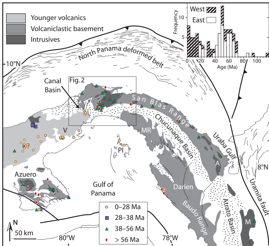
Figure 1. Tectonic setting of the Isthmus of Panama (compiled from: Woodring, 1957; Stewart et al., 1980; Duque-Caro, 1990; Mann and Corrigan, 1990; Silver et al., 1990; Mann and Kolarzky, 1995; Kerr et al., 1997; Coates et al., 2004; Buchs et al., 2010). A—Acandí Batholith; MR—Maje Range, PI—Pearl Islands; M—Mande Batholith; V—El Valle Volcano. Inset shows geochronologic data (compiled from: Guidice and Recchi, 1969; Kesler et al., 1977; Aspden et al., 1987; Defant et al., 1991a, 1991b; Maury et al., 1995; Speidel et al., 2001; Lissina, 2005; Rooney et al., 2010; Wegner et al., 2011), and also includes geochronologic data reported in this study. Histogram shows the same geochronologic compilation separated in two groups: west of the canal in diagonal pattern, and Canal Basin and east of the canal in white.
