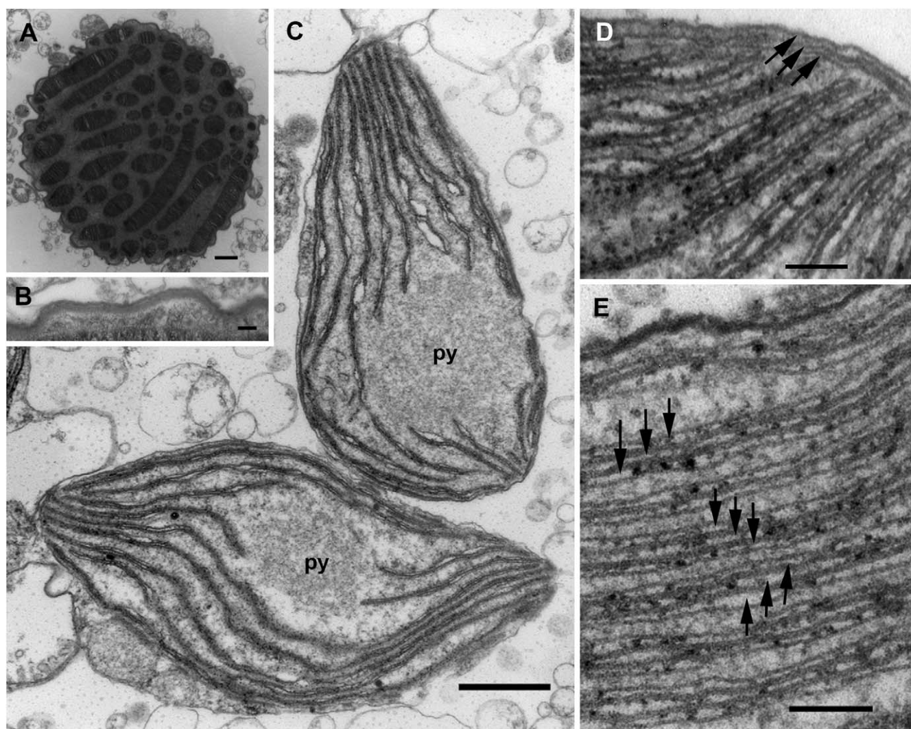
Fig. 3. Transmission electron micrographs of Polykrikos hartmannii . (A) Nucleus with condensed chromosomes. Scale bar = 2 \mu m. (B) Detail of the nuclear membrane. Scale bar = 100 nm. (C) Two spindle-shaped typical dino-chloroplasts with thylakoids in stacks and pyrenoid (py) not traversed by thylakoids. Scale bar = 500 nm. (D) Detail of a chloroplast showing the three outer membranes (arrows) typical for peridinin-containing dino-chloroplasts. Scale bar = 100 nm. (E) Detail of a chloroplast showing thylakoids in stacks of three (arrows) typical for peridinin-containing dino-chloroplasts. Scale bar = 100 nm.
