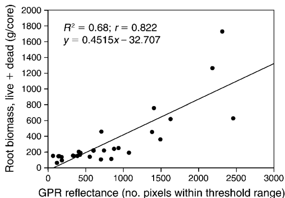
FIG. 3. Relationship between total live plus dead root biomass obtained from soil cores (g/15 cm core diameter to 60 cm depth) and ground-penetrating radar (GPR) root reflectance (total pixels within threshold). Root reflectance was determined by measuring the total number of pixels (pixel intensity) within a specific intensity threshold in each GPR image. The solid line represents a significant linear regression of the mass to GPR signal reflectance.
