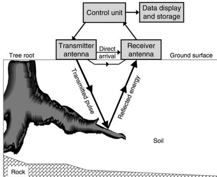
FIG. 1. Basic ground-penetrating radar (GPR) operation. High-frequency electromagnetic waves are emitted from the transmitting antenna complex into the soil and reflect off a buried object back to the receiving antenna. Time and signal strength are recorded by the control unit and produce hyperbolic-shaped images on the display screen.
