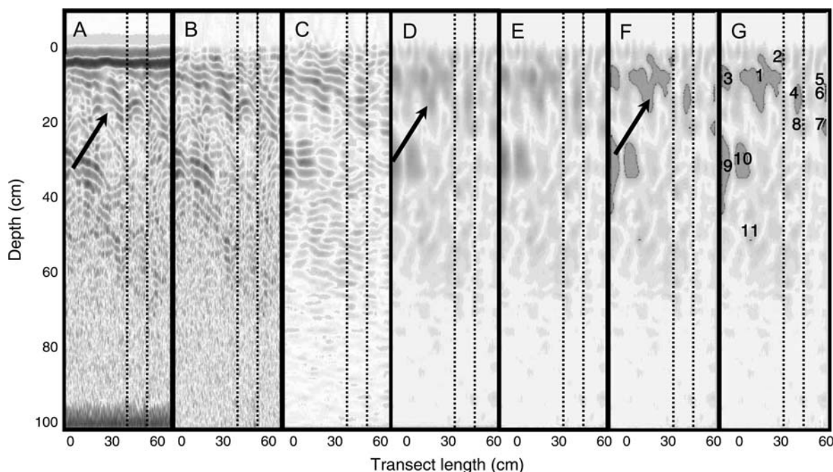
FIG. 2. Representative radar profile and standard image analysis/processing from a scrub-oak ecosystem at Kennedy Space Center, Florida, USA. Arrows point to a common reflector (i.e., root) located at 15 cm depth. Dotted vertical lines show the relative size for an individual core that would be extracted for biomass correlation. (A) Raw radar data from a 1500-MHz ground-penetrating radar antenna; (B) same profile processed in RADAN software with a finite impulse response filter (FIR) background removal to reduce low-frequency noise and bands; (C) Kirchoff migration, used to correct the reflector's (object's) position and hyperbolic geometry; (D) radar profile after a Hilbert transformation to express the magnitude of the signal to enhance the subtle objects and reduce false "echoes"; (E) post-processed images converted to gray scale; (F) roots quantified with Sigma Scan Pro Image Analysis software by setting the image pixel intensity threshold to the 60–255 range, which measures each pixel's intensity on a threshold scale; and (G) quantification of the image, accomplished by summing the number of pixels in each grouping (given a unique number).
