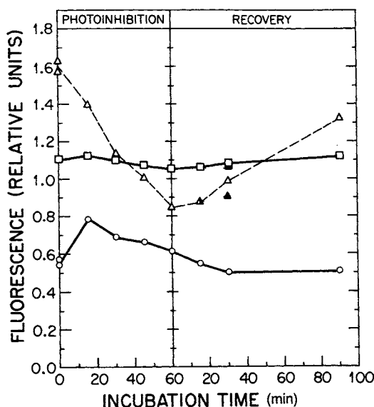
Fig. 2. Variation in Chl fluorescence parameters of Chroomonas sp. (Chang 2) during exposure to high irradiance (photoinhibition) or after return to low light (recovery). High irradiance ( \sim 1,700 \mu\text{mol quanta m}^{-2} \text{s}^{-1} ) was maintained for 60 min before the light was extinguished and incubation was continued in ambient light ( \sim 10 \mu\text{mol quanta m}^{-2} \text{s}^{-1} ). Symbols as for Fig. 1. Filled symbols indicate samples from parallel dark incubations; all other samples were dark adapted for 5 min before measurement. Note that when F_0 and F_{\text{max}} vary in opposite directions, there is minimal variation in F_{\text{cyt}} .
