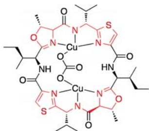
Bis-Cu(II)-ascidiacyclamide complex
