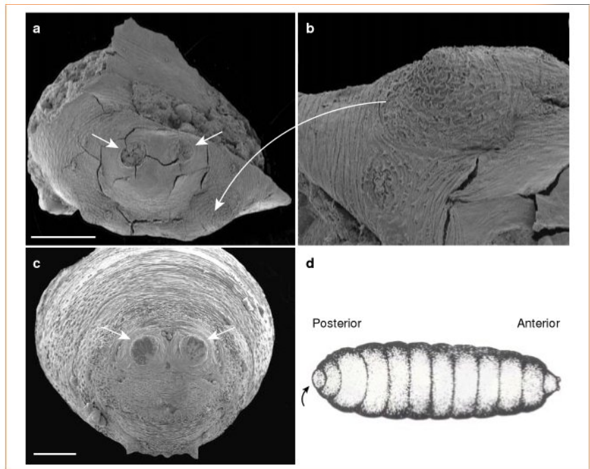
Figure 1 Scanning electron micrographs of the Antarctic fly fossil puparium compared with a modern puparium. The puparium is the hardened integument of the 3rd (last) instar (maggot) from which the adult fly emerges. a , Posterior view of the fossil puparium, which is partly crushed and has silt grains embedded in the chitin. The posterior spiracles are indicated by the pair of white arrows. Scale bar, 0.5 mm. b , Enlarged view of a ventral cuticular welt on the fossil, showing the presence of spines. c , Posterior segment of a modern puparium of a blowfly ( Cochliomyia macellaria ; Fabricius: Calliphoridae). Spiracles are indicated by arrows. Scale bar, 0.5 mm. d , Drawing of a puparium to show the location (arrow) of the posterior spiracles in both the fossil ( a ) and a modern specimen ( c ).
