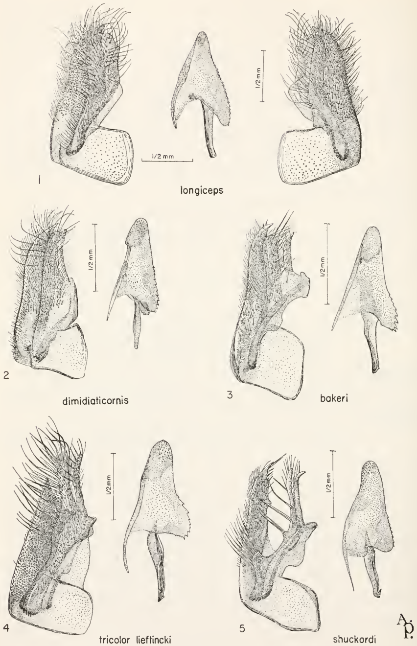
FIGURES 1-5.—Male genitalia, cardo omitted, Hylomesa : 1, internal aspect at left, exterior aspect at right, lateral aspect of aedeagus in center; 2-5, internal aspect at left, lateral aspect of aedeagus at right.
