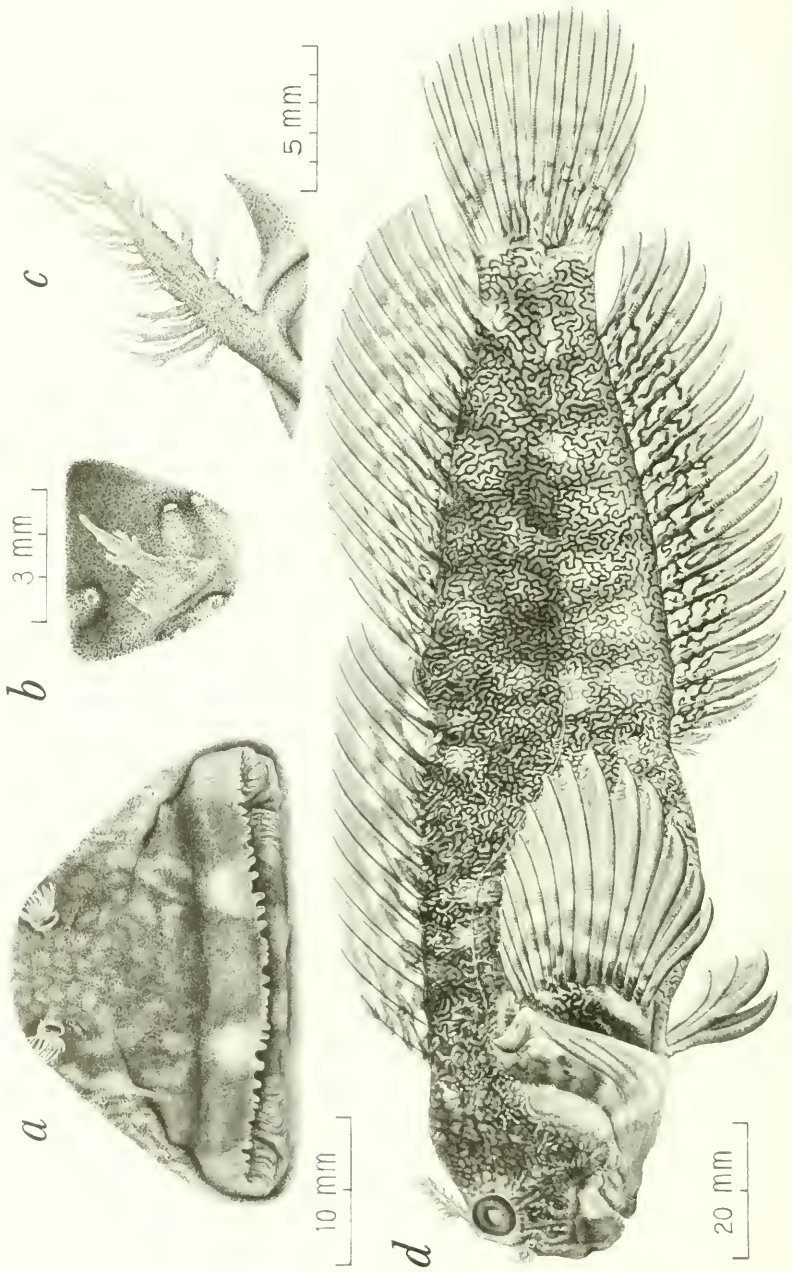
Entomacrodus nermiculatus , ANSP 102198, male, 149 mm SL, Scyphelles: a , upper lip; b , left nuchal cirri; c , left supraorbital cirri; d , lateral view.
