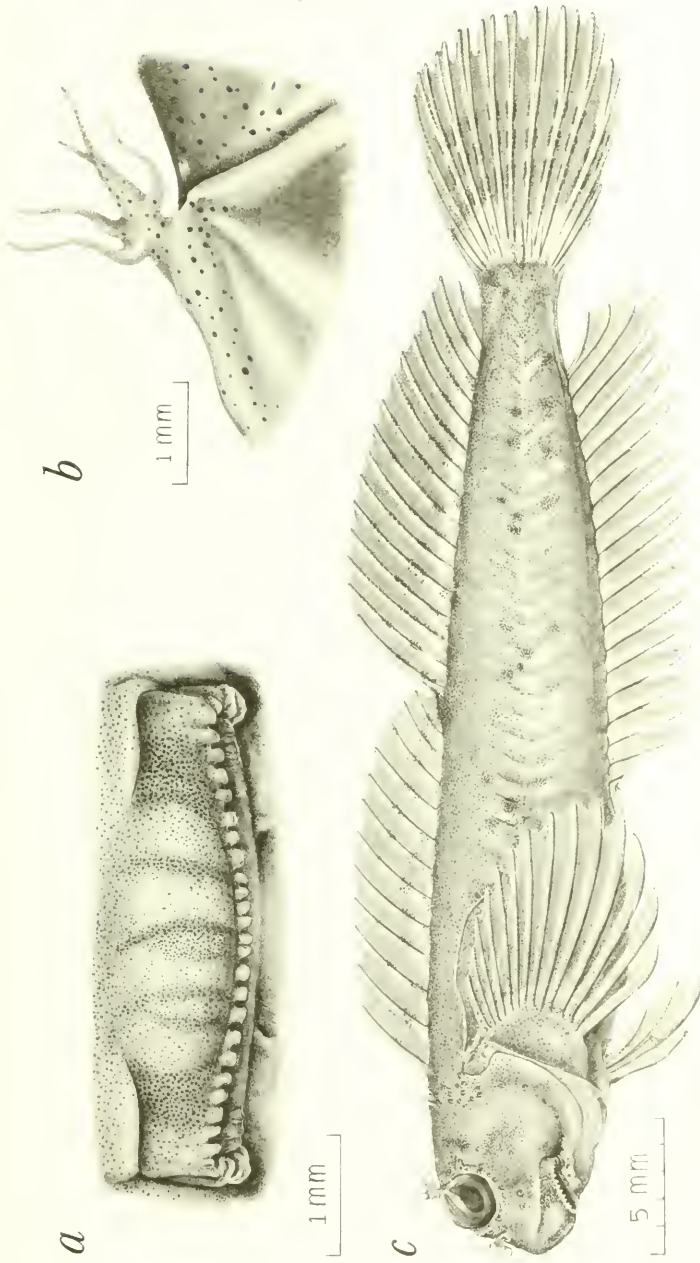
Entomacrodus roferi , SU 62038, female, 36.4 mm SL, Rarioia: a, upper lip; b, left supraorbital cirri; c, lateral view.
