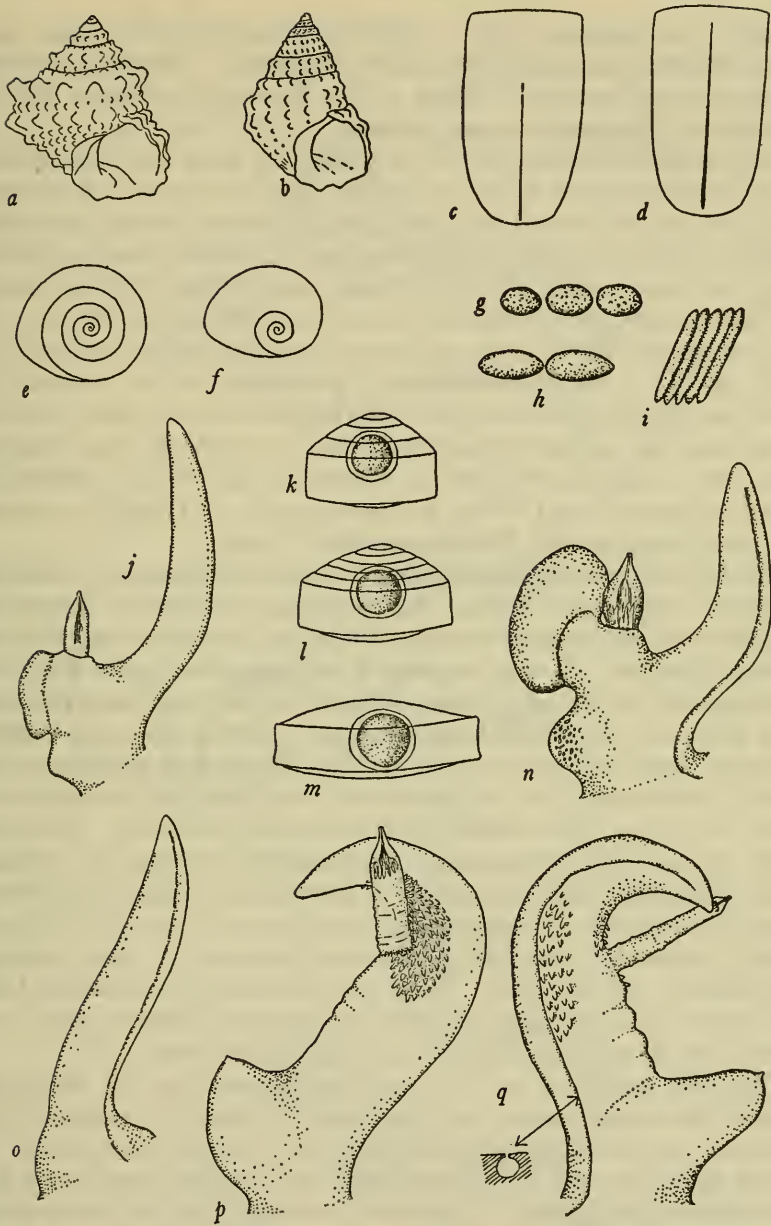
FIGURE 55.— a , Shell of Echininus nodulosus Pfeiffer ( \times 1\frac{1}{2} ). b , Shell of Nodilittorina tuberculata Menke ( \times 1\frac{1}{2} ). c , Underside of foot of E. nodulosus ( \times 2 ). d , Underside of foot of N. tuberculata ( \times 2 ). e , Operculum of E. nodulosus ( \times 2 ). f , Operculum of N. tuberculata ( \times 2 ). g , Fecal pellets of E. nodulosus ( \times 4 ). h , Fecal pellets of N. tuberculata ( \times 4 ). i , Fecal pellets of Modulus modulus Linné ( \times 4 ). j , Penis of Littorina ziczac Gmelin ( \times 6 ). k , Floating egg capsule of L. ziczac (diam. 0.20 mm.). l , Egg capsule of N. tuberculata (diam. 0.24 mm.). m , Egg capsule of Tectarius muricatus Linné (diam. 0.24 to 0.32. After Lebour, 1945). n , Penis of N. tuberculata ( \times 6 ). o , Penis of T. muricatus ( \times 6 ). p , q , Penis of E. nodulosus ( \times 6 ).
