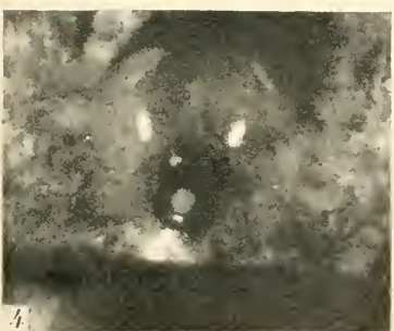
1, 2. Two spirals in legless part of abdomen of Apus longicaudatus , ♂, from Kansas (Stockholm Mus.), dorsal and ventral views, \times 4 (this specimen was examined and described as Apus lucasanus by Packard). 3-6. Eyes and nuchal organs of, respectively, Lepidurus lynchi , new species, ♂, \times 7 ; L. lynchi echinatus , new variety, ♀, \times 6 ; L. coesii , ♂, \times 9 ; and L. packardi , ♀, \times 12 .
