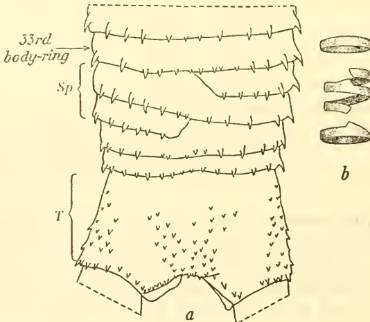
FIGURE 5.— a , Ventral view of portions of the abdomen and telson of a female of Apus longicaudatus LeConte (U. S. N. M. No. 82034) showing a right-handed spiral of two rounds placed within the series of normal rings and beginning and ending in the mid-ventral line, \times 29 . ( Sp , spiral; T , telson.) b , Schematic drawing of the spiral and the rings immediately anterior and posterior to it.
