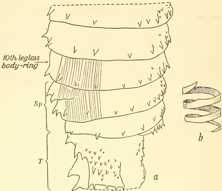
FIGURE 4.— a , Lateral view of portions of the abdomen and telson of a male of Apus longicaudatus LeConte (U. S. N. M. No. 11604) showing a left-handed spiral of about two and three-quarters rounds, beginning dorsolaterally and evenly tapering at distal end, \times 28 . Arrangement of muscle bundles indicated on the left side. ( Sp , spiral; T , telson.) b , Schematic drawing of the spiral.
