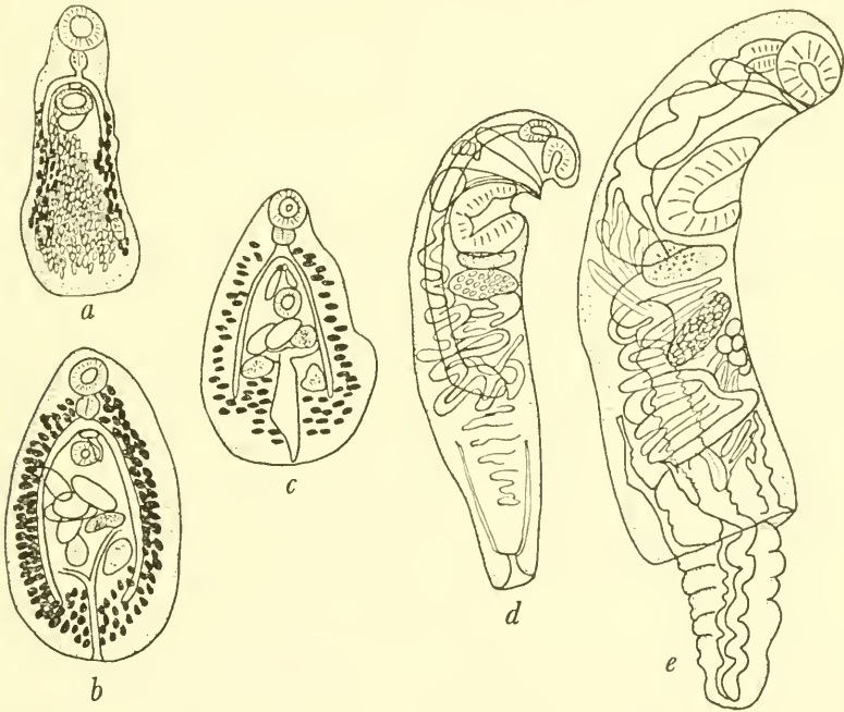
FIGURE 8.—a, Paramonorchoides bivittellus Manter; b, Lepocreadium archosargi , new species; c, Lepocreadium micropogoni , new species; d, Lecithochirium microstomum Chandler; e, Lecithochirium muraenae Manter. \times 38 .
