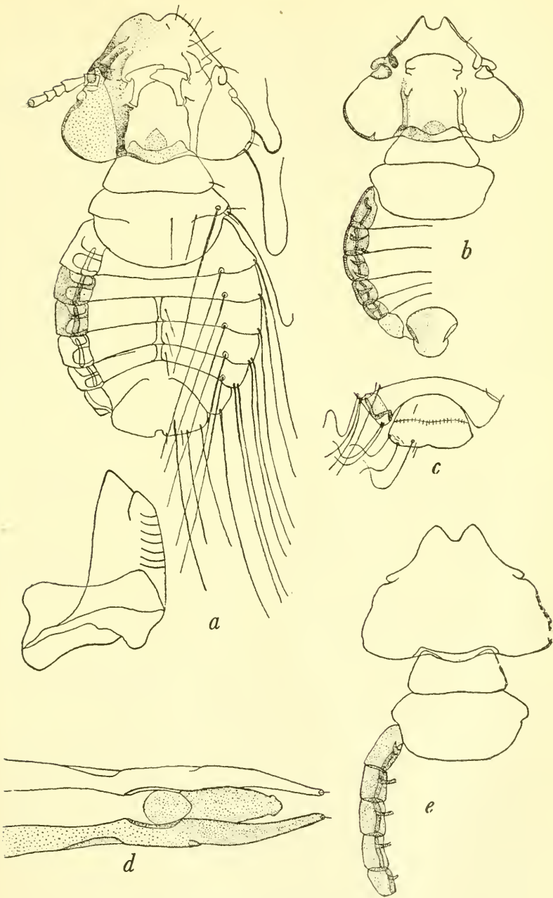
FIGURE 8.—MEGAGINUS
