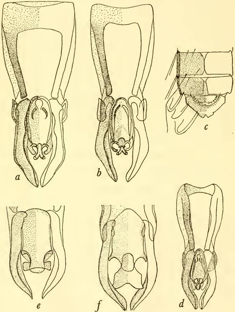
FIGURE 2.—PSEUDOLIPEURUS
