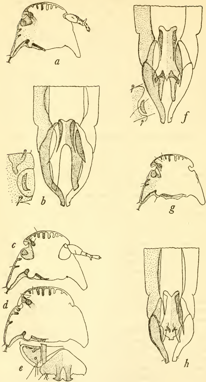
FIGURE 13.—HEPTAPSOGASTER
