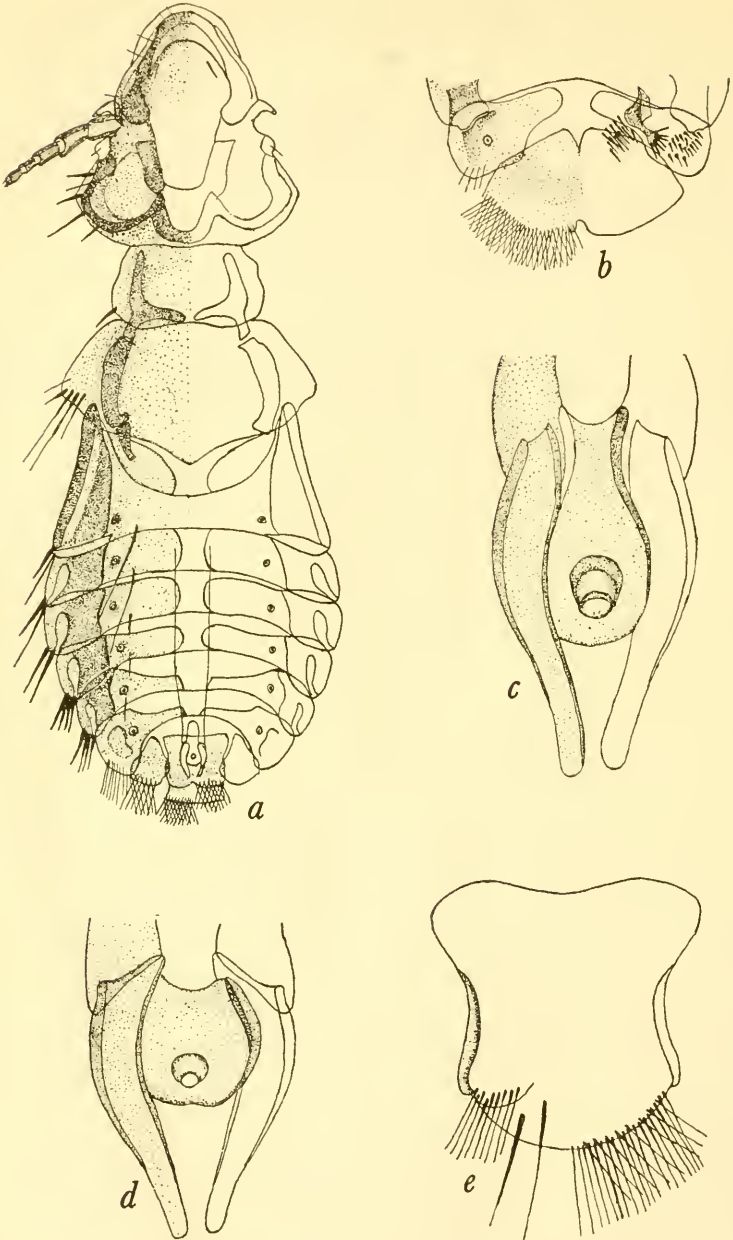
FIGURE 7.—STRONGYLOCOTES
