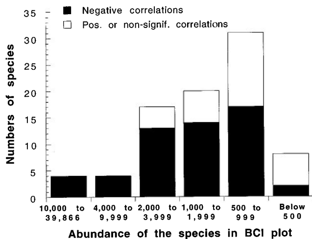
FIG. 1. Number of species that show significant density-dependent effects on r , as a function of the abundance of the species.
