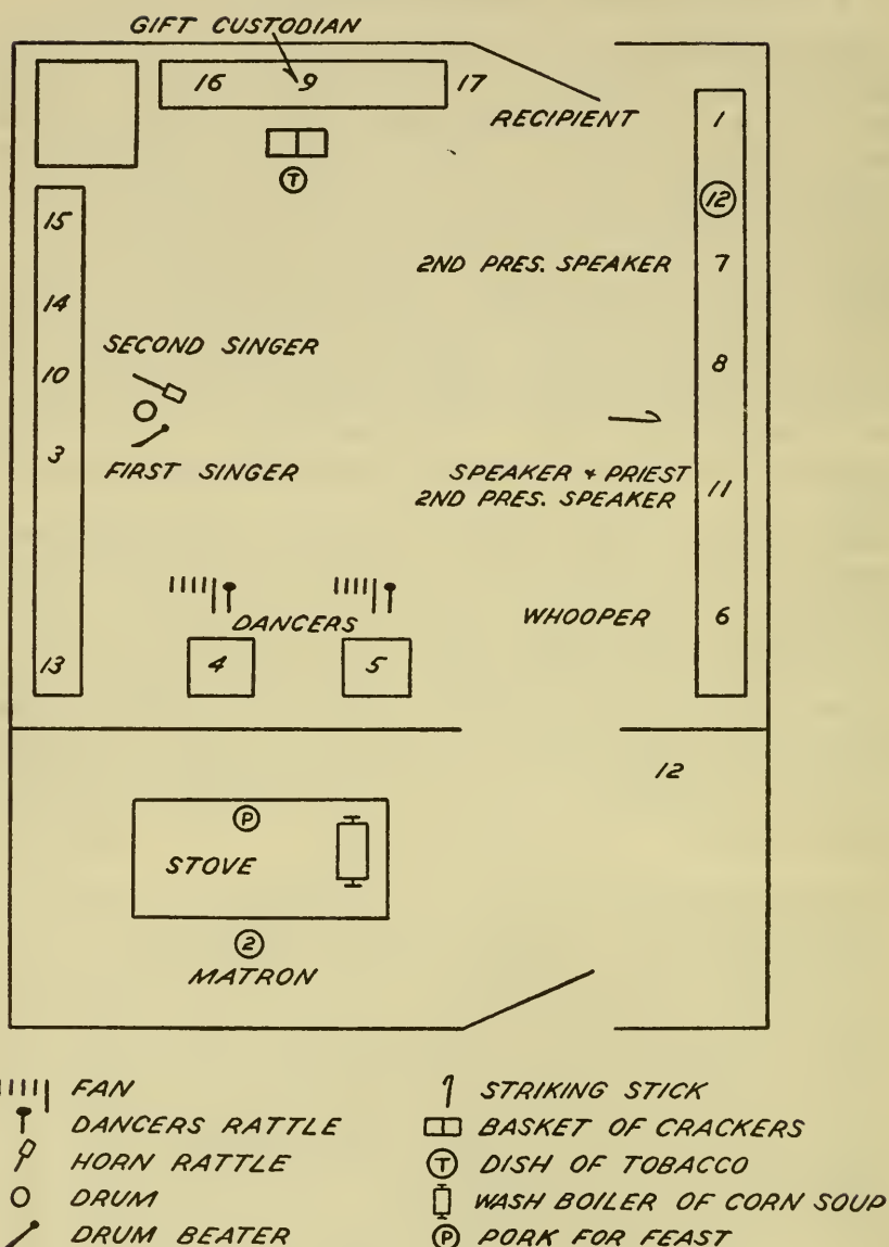
FIGURE 1.—Floor plan of Eagle Dance for Francis Bowen.
