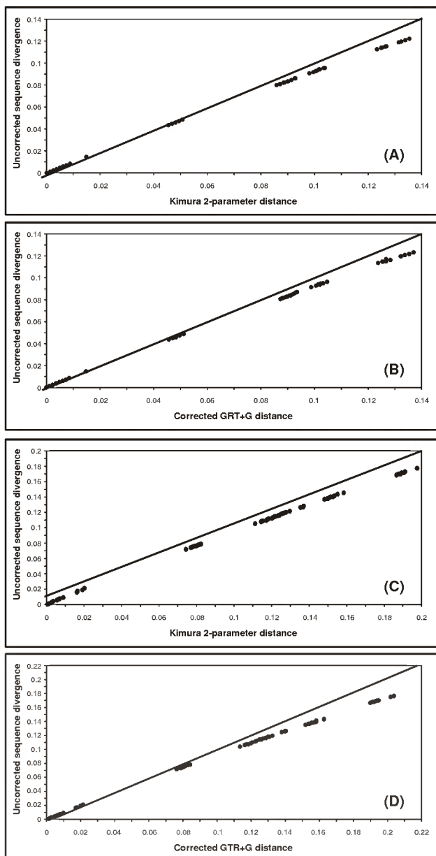
Figure 1. Plots depicting relative rates of transitional saturation for the 12S (A) and 16S (C) Gene sequences; and substitutional saturation for 12S (B) and 16S (D) using pair-wise genetic distances corrected under the GTR evolutionary model.
