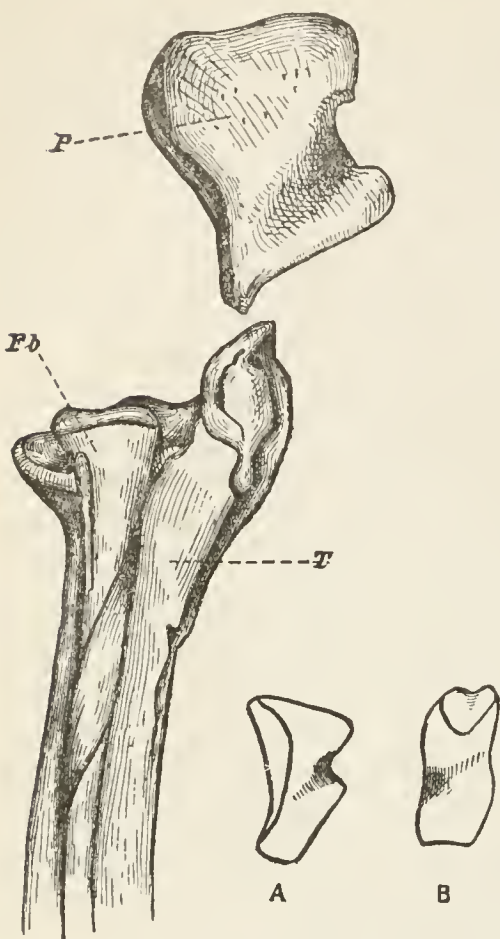
FIG. 1.—Leg-bones and patella, right limb, of Aptenodytes pennanti ; life-size from nature. T, tibia; F, fibula; P, patella; the last slightly raised above its articulation with tibia. (No. 11976, Smithsonian Collection.) By the author. A, patella of Eudyptes chrysocome (from Triston d'Acuha) outer surface, natural size. B, the same seen from in front (after Watson).
