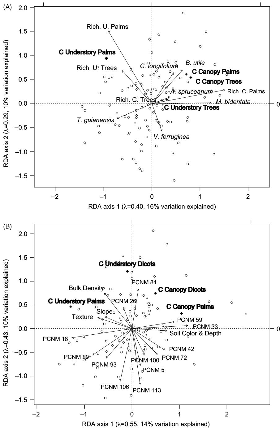
FIGURE 2. Correlation biplots from Redundancy Analysis of tree carbon storage in understory trees and palms and canopy trees and palms constrained by the explanatory matrices of (A) diversity and (B) environment and space (arrows) in Fort Sherman, Panama (see Table S3 for details in explanatory variables). Circles indicate the subplots ( N=117 ). Crosses indicate the centroids of the response variables. Angles between tree carbon storage (variables in bold) and arrows of explanatory variables reflect their correlations. If the projection of tree carbon storage from the center of the axis is parallel to an arrow of an explanatory variable, then they are related. Arrow size is positively related to its effect level.
