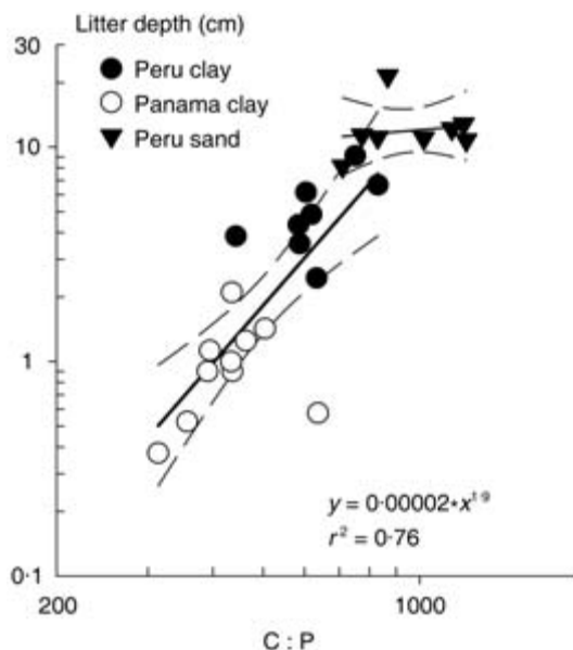
Fig. 2. Standing litter depth covaries with the ratio of carbon to phosphorus in decomposing litter across 26 forest sites in Panama and Peru. The overall regression equation is given; regressions for clay and sandy soils (with 95% CI) drawn separately.
