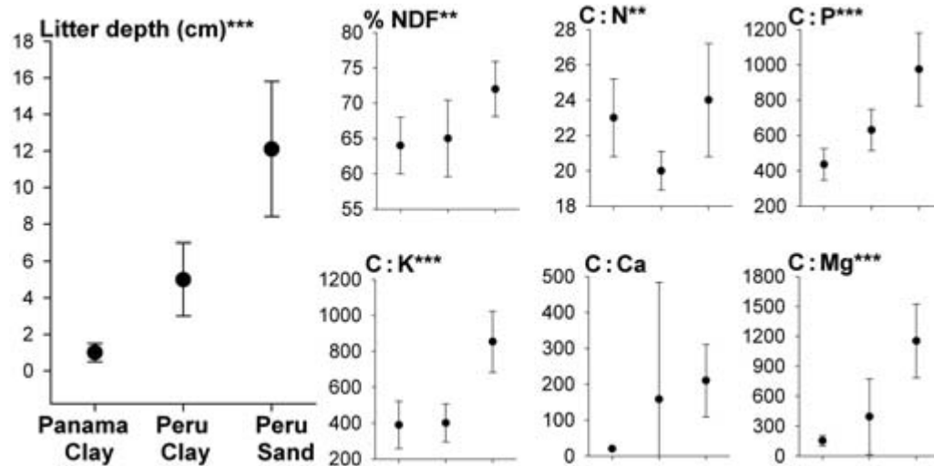
Fig. 1. Litter depth and chemistry (of leaf litter + microbes) for three groups of forest stands—Panama clay soils ( n = 10 ), Peru Clay soils, and Peru sandy soils ( n = 8 for chemistry, n = 9 for litter depth). Means are given with standard deviations. ANOVA significance: * P > F < 0.05 , ** P > F < 0.01 , *** P > F < 0.001 . NDF (neutral detergent fibre) is a measure of the celluloses, hemicelluloses, and lignins in the decomposing litter.
