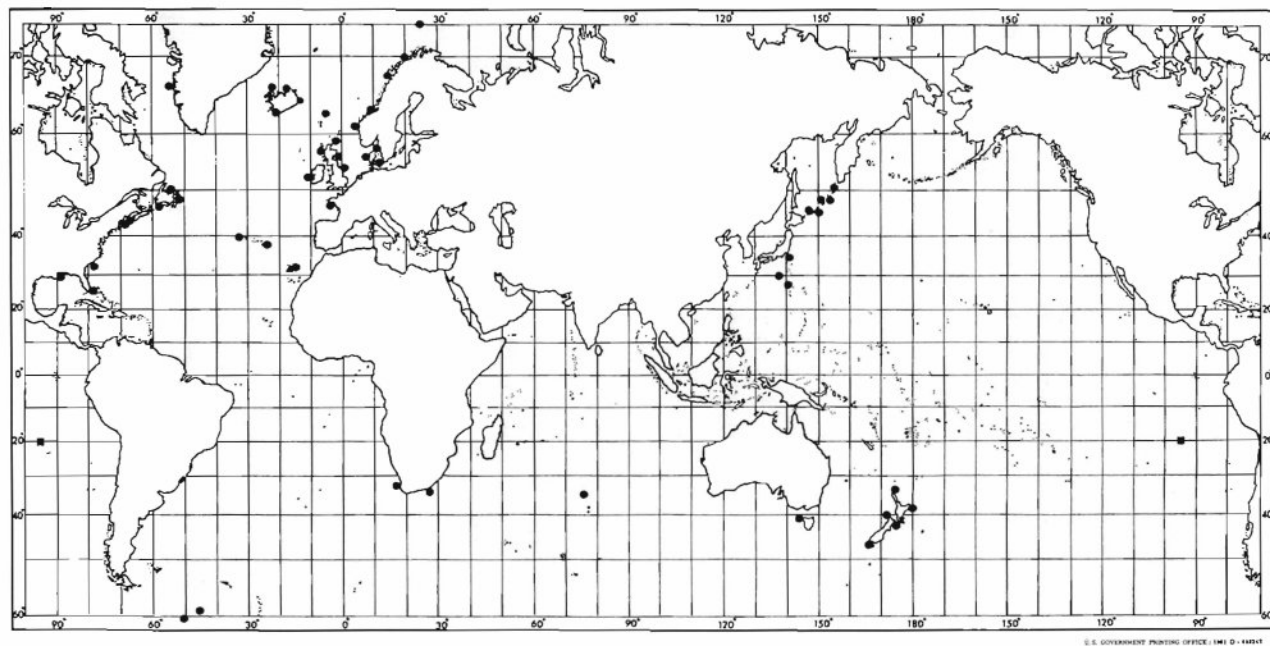
FIG. 6. Locality records of Architeuthis (redrawn after Clarke, 1966, fig. 2). Locations of captures of juvenile specimens reported here indicated by the solid triangle (Atlantic) and the solid square (Pacific). Additional records from New Zealand (Dell, 1970) and Newfoundland (Aldrich, 1968) indicated by 'x's.
