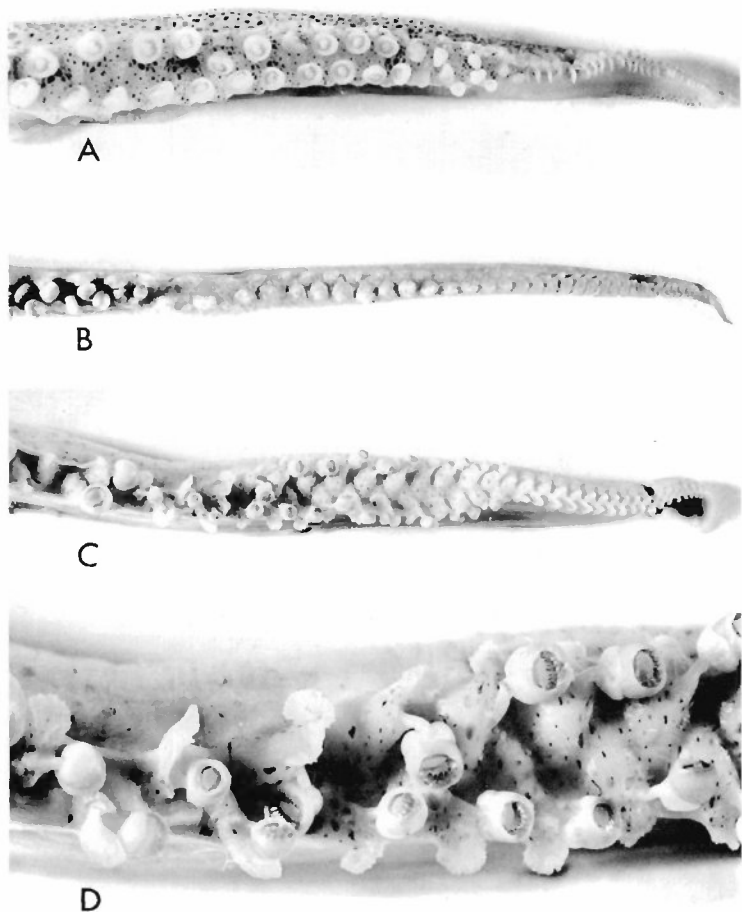
PLATE 9. Hectorcotyli of Illex species. A. I. illecebrosus , 252 mm ML; Newfoundland. B. I. argentinus , 167 mm ML; Argentina. C. I. coindetii , 166 mm ML; western Mediterranean. D. I. coindetii , enlargement of a portion of C. showing fringed trabeculae.
