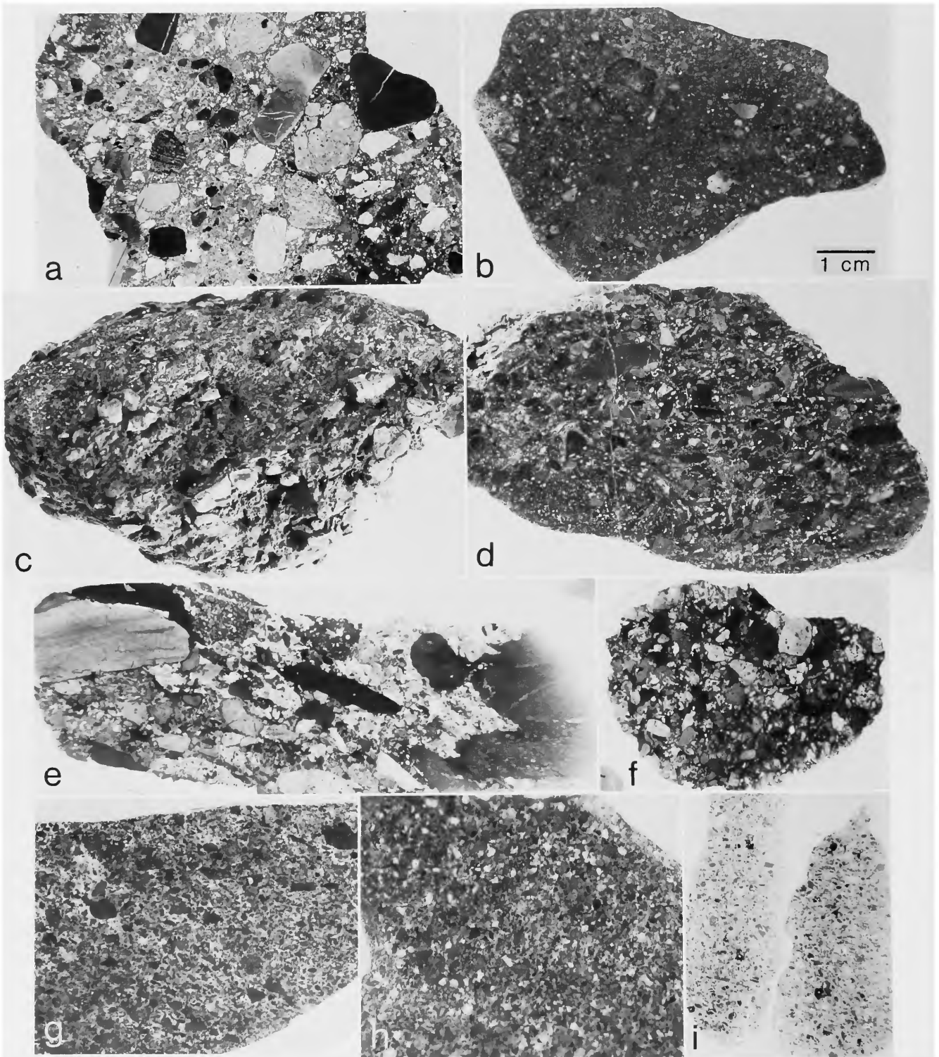
FIGURE 10.—Hand specimen ( c ), polished sections ( a, b, d–h ) and thin section ( i ) of different debris flow deposits (mostly volcaniclastics) showing diverse examples of clast size and shape and clast-to-matrix fabric. For example, some clasts tend to be angular in c, d , and e and subangular to subrounded in a, f , and g . Clasts appear to “float” in muddy sand matrix in b ; in contrast, clasts are in contact with each other in f . Localities (in Figure 2): a = site 17; b = site 46; c, d (respectively, hand and polished section of same sample) = site 27; e, f = site 50; g = site 34; h = site 57; i = site 14. Scale bar applies to all components.
