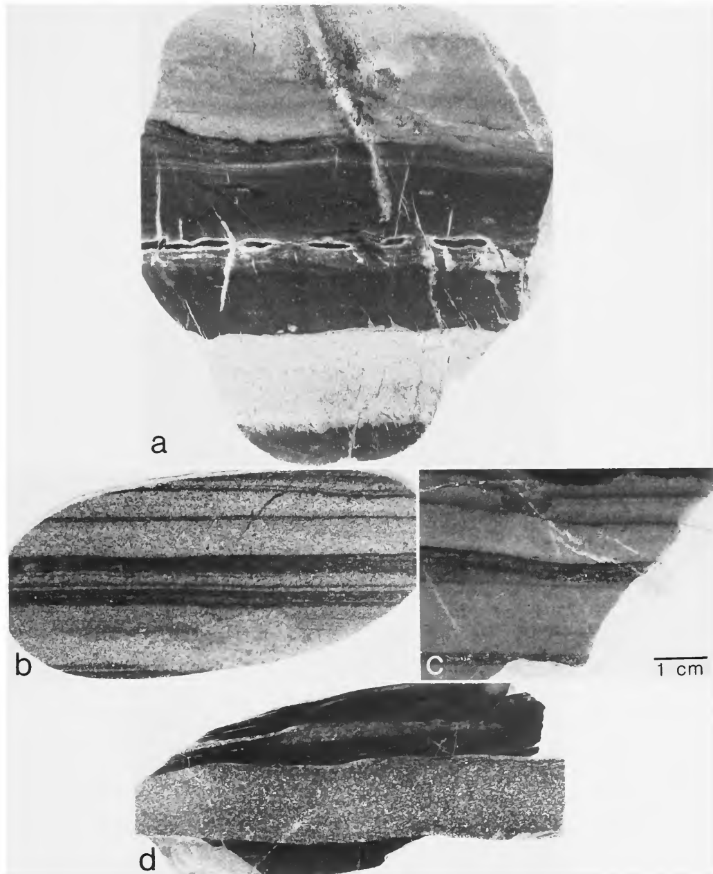
FIGURE 7.— Polished sections of almost structureless, sandy, volcaniclastic layers with sharp top and sharp base. These are interpreted as sand-flow (grain- or fluidized-flow) deposits. Lower sandstone layer in a , subtly graded, is similar to basal division A of turbidites. Localities (in Figure 2): a, b = site 50; c = site 57; d = site 27. Scale bar applies to all components.
