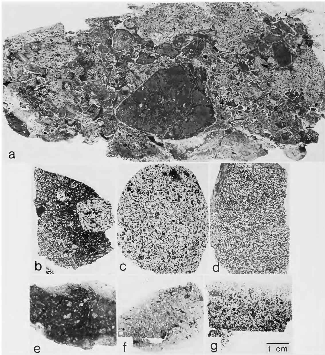
FIGURE 12.—Polished slab ( a,d,e ) and thin sections ( b,c,f,g ) of various submarine volcanoclastic flows. Hand specimen ( a ) was collected at the exposure shown in Figure 11 a . Samples show disorganized ( b ), to partially organized ( c ), to organized (graded bedding in d ) nature. Localities (in FIGURE 2): a = site 17; b = site 12; c = site 21; d = site 19; e-g = site 21. Scale bar applies to all components.
