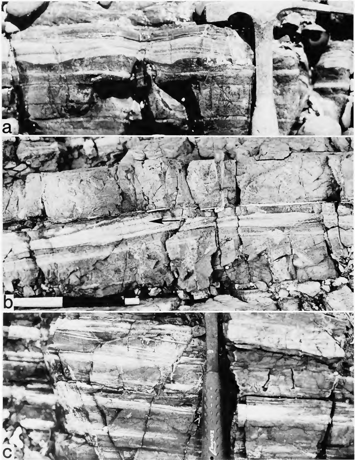
FIGURE 62.—Thin, laminated, sandstone strata showing some features commonly associated with turbidites (graded bedding and basal erosional markings in a ), but many lack the accepted, orderly, vertical turbidite sequence of A to E bedform divisions. Tractive current transport is recorded by foreset and wavy-ripple bedding and concentrations of heavy minerals ( b ). Discontinuous bedding and pinch-out also commonly observed. Sandy units, such as those in b and c , typical of most sandstone layers observed in Caledonia Formation in St. Croix and Buck Island and also some sections of the Judith Fancy Formation and other Cretaceous tuffaceous units in St. Croix. These sandy layers are probable reworked turbidites. Localities (Figure 2): a = site 3; b = site 19; c = site 29. Pen is 14 cm and hammer is 28 cm long.
