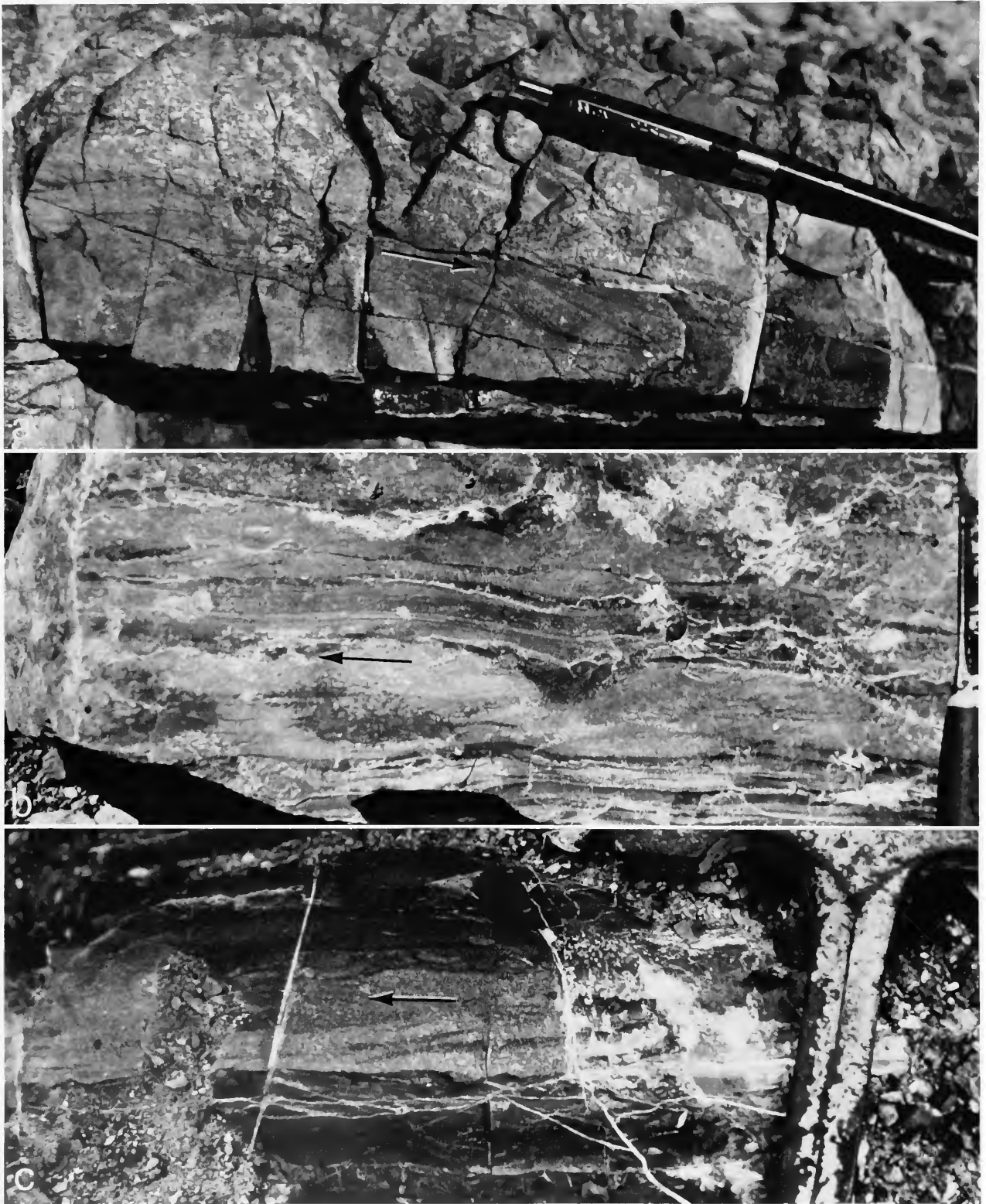
FIGURE 41.—Current laminated sandy strata, with sharp flat base but wavy upper surface. Apparent current transport, shown by arrows, toward right in a and toward left in b and c . Dark laminae in c highlighted by concentrations of heavy minerals. Localities (Figure 2): a = site 7; b = site 57; c = site 55. Pen is 13 cm and hammer is 28 cm long.
