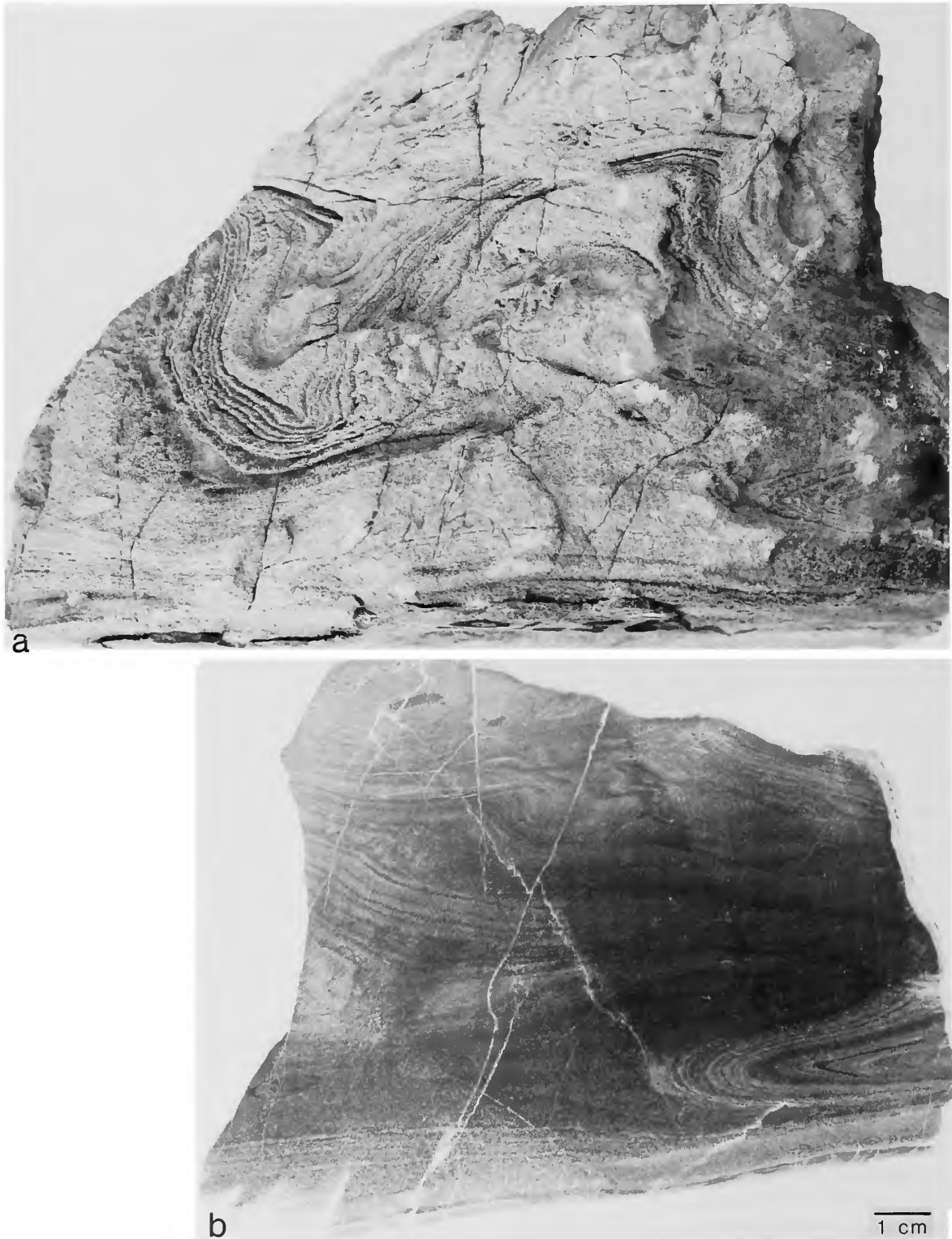
FIGURE 22.—Hand specimen showing syndeformational deformation structures (including very tight convolution and possible dewatering features) within sharp-based and -topped sandstone bed (see Figure 19a) at East End Point (site 19, Figure 2). a , Weathered surface; b , polished section. Scale bar applies to all components.
