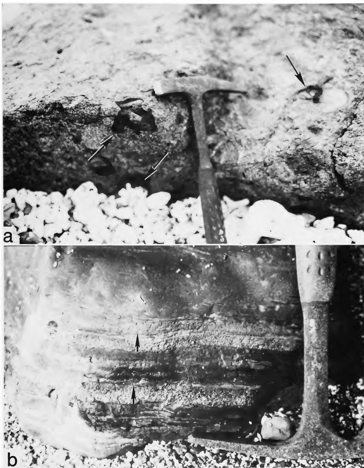
FIGURE 29.— a , Rip-up siltstone clasts (arrows) in basal massive (A) part of thick turbidite. b , Thin but very coarse sandstone turbidites. Note sharp base and well-developed fining-upward trends (arrows). Localities (in Figure 2): a = site 16; b = site 50. Hammer is 28 cm long.
