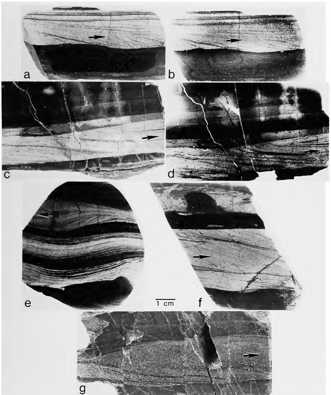
FIGURE 42.—Polished sections ( a,c,e-g ) and thin sections ( b,d ) showing non-graded sandy strata with sharp base and top. Foreset lamination (arrows indicate apparent current directions); some laminae highlighted by heavy minerals ( a-d ). Note lens-shaped ripple-bedded stratum in g . Localities (Figure 2): a-d = site 22; e = site 21; f = site 50; g = site 19. Scale bar applies to all components.
