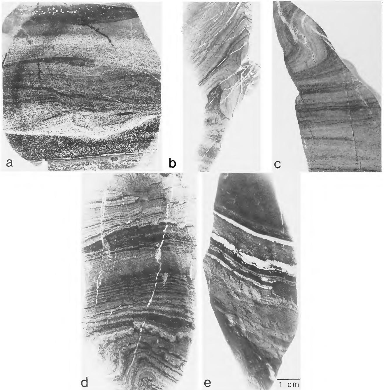
FIGURE 26.—Polished sections showing deformed structures, some ( b,d,e ) which probably have post-depositional component. Note offset of laminae in d . Petrographic analyses indicate recrystallization veins, and mineralogical alterations associated with low-grade metamorphism. Localities (in Figure 2): a = site 34; b = site 9; c = site 23; d = site 25; e = site 52. Scale bar applies to all components.
