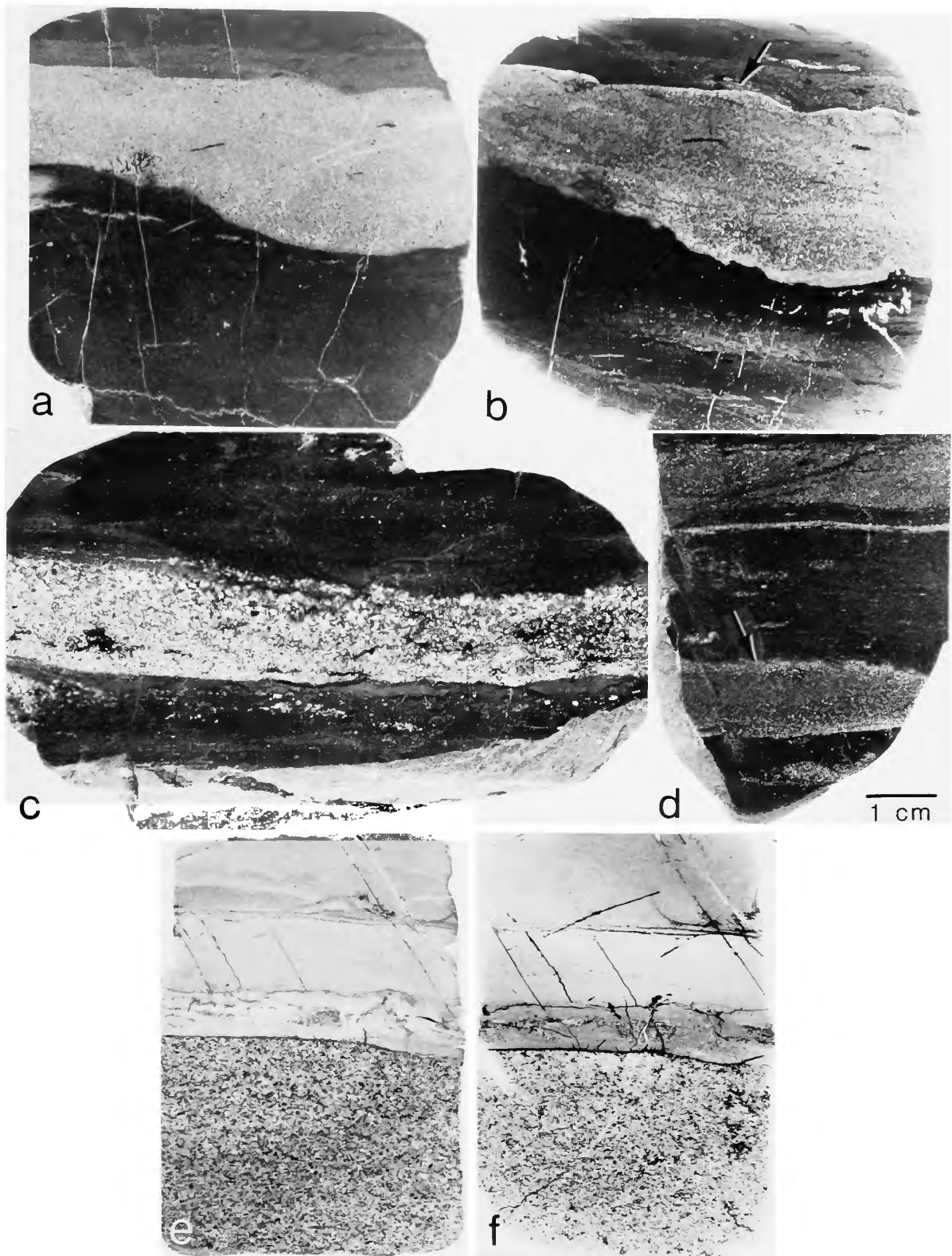
FIGURE 48.—Polished ( a, c-e ) and thin sections ( b, f ) showing non-graded ( e, f ) and reverse-graded bedding (in b-d ). Note rippled bedform in a, b , and lenticular configuration in d . Localities (Figure 2): a, b = site 21; c = site 50; d = site 53; e = site 14. Scale bar applies to all components.
