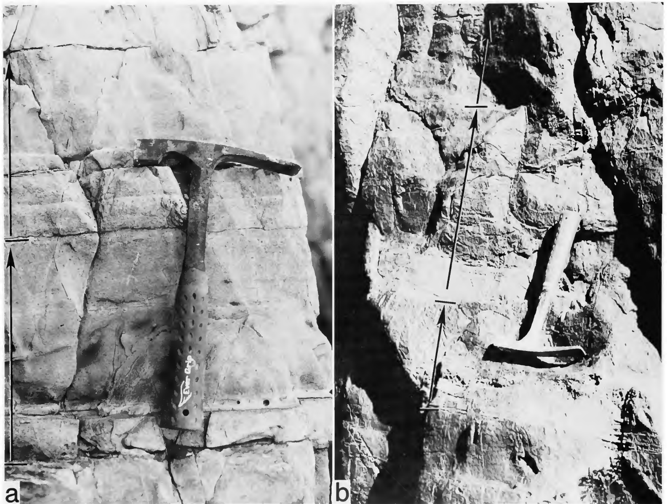
FIGURE 28.—Sections of superposed A-B and B-C turbidites. a , Lower turbidite division is massive graded (A). b , Lower division is plane laminated (B). Localities (in Figure 2): a = site 23; b = site 43. Hammer is 28 cm long.
