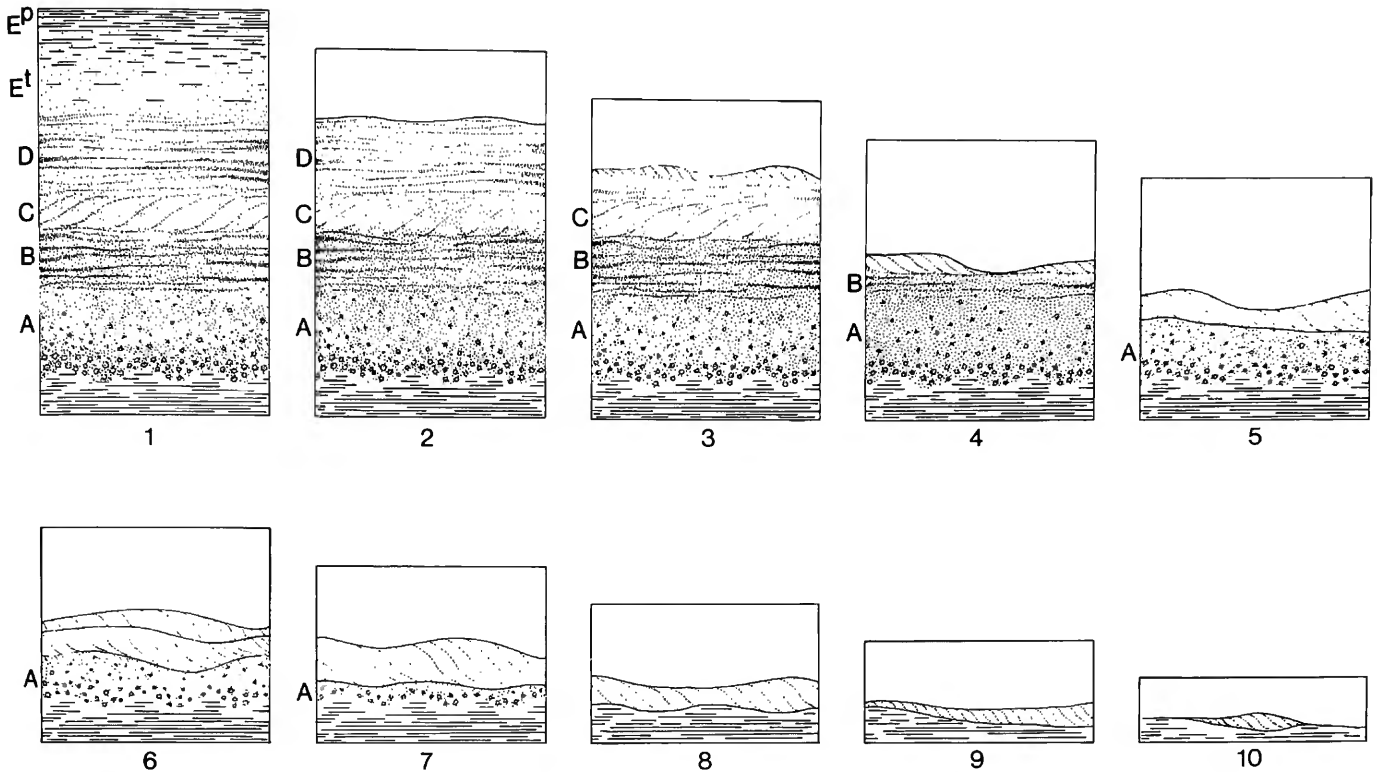
FIGURE 63.—Scheme showing possible continuum of structures that could result from reworking of sandy layer originally emplaced as complete A–E turbidite (1, at left). Reworking would result in partially eroded (2) and redeposited turbidite (variant layer) series (3–7), to completely remolded and entirely foreset laminated (8, 9) and discontinuous (10) layers. Stratal types 7 to 10 are end-products of reworking by bottom currents. Note progressive downward erosion and lateral disruption of original turbidite layer. Actual examples presented in this monograph that could be used to illustrate this series as follows: 1 = Figure 39a; 2 = Figure 28a; 3 = Figure 56a,b; 4–7 = Figure 53b; 8 = Figure 55b; 9 = Figure 62b; and 10 = Figure 45a.
