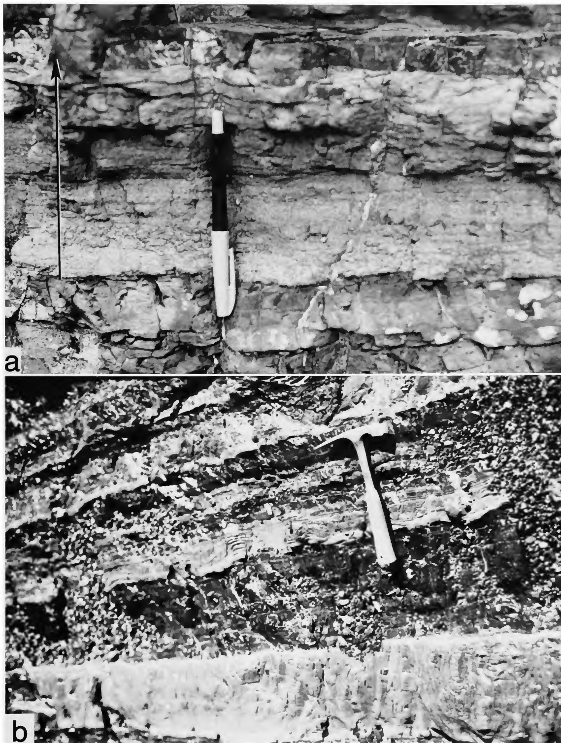
FIGURE 39.—Comparison of graded A–E sandstone turbidite ( a , arrow) and B–E turbidite ( b , stratum under hammer handle) with non-graded, sharp base-sharp top layer with poorly developed sequence of internal structures (20 cm-thick layer, at bottom of photo in b ). Origin of this latter sandstone stratum remains undefined. Localities (Figure 2): a = site 17; b = site 3. Pen is 14 cm and hammer is 28 cm long.
