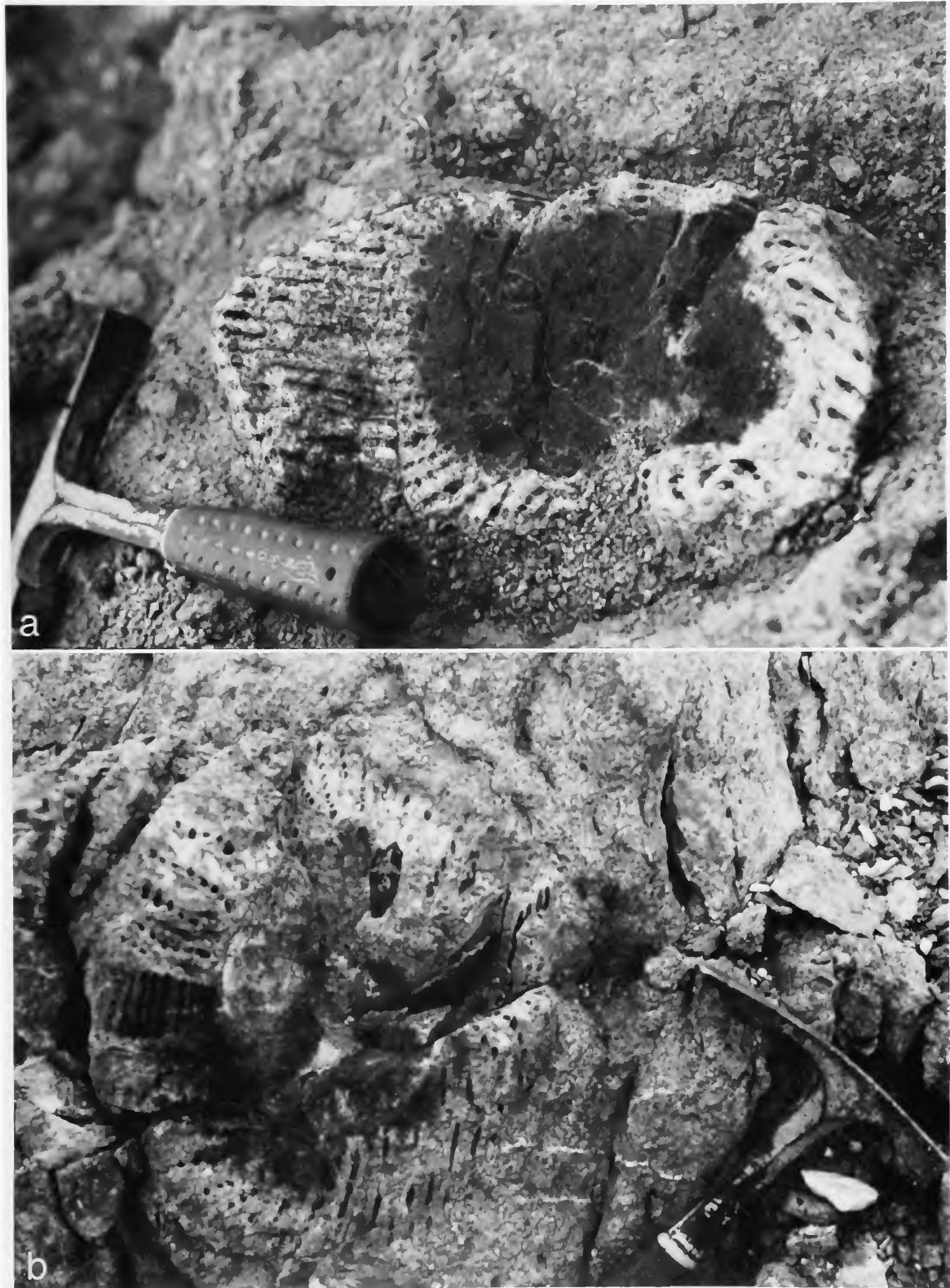
FIGURE 17.—Worn rudists ( Barrettia gigas ) embedded in coarse carbonate and fossil-bearing debris-flow deposits at Vagthus Point (Judith Fancy Formation, site 6, Figure 2; photo of exposure in Figure 14a). Long axis of specimens is flat-lying, not vertical as in their living position; such large fossils usually occur near base of beds. Hammer is 28 cm long.
