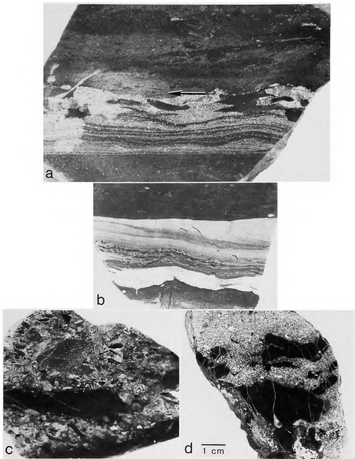
FIGURE 15.—Polished sections showing dark, mudstone rip-up clasts in medium- and fine-grained sandstone ( a,b ), and in coarse-grained sandstone ( c,d ). Angular fragments may be irregularly distributed ( c,d ) or concentrated along specific parts of layers ( a,b ). Elongate clasts sometimes imbricated (transport toward left in a ). Localities (in Figure 2): a-c = site 50; d = site 23. Scale bar applies to all components.
