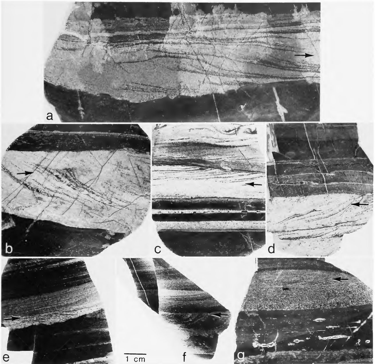
FIGURE 57.—Polished sections showing examples of thin, sharp-based (some with an erosional surface), and sharp-topped layers; some display moderate graded bedding at base. Upper foreset laminations may be truncated (particularly b–d, f ); small arrows indicate apparent direction of transport. Foreset laminations can extend from (or near) top to base of bed. In several cases, laminations are highlighted by heavy mineral concentrations ( b, c ). Geometry of such strata is diverse: wavy bedded ( a ), wedge-like ( c ) or lenticular ( g ). Localities (Figure 2): a, c, e = site 50; b = site 43; d = site 17; f = site 52; g = site 18. Scale bar applies to all components.
