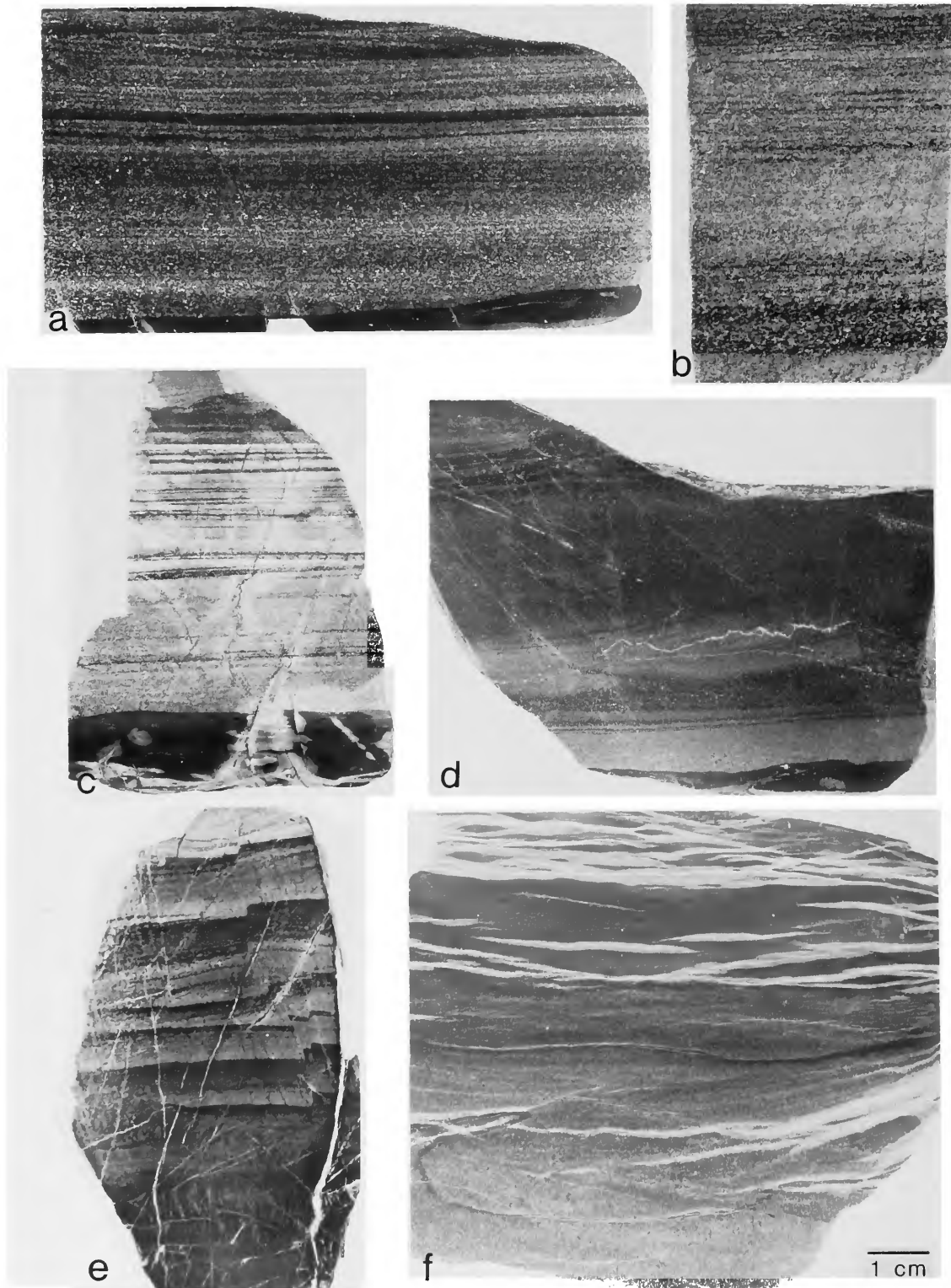
FIGURE 36.—Polished sections of thin sandy B-E ( a-c ) and C-E ( d,e ) turbidites. Note post-depositional effects such as vein filling ( d ), small-scale "micro-fault" and offsets ( e ) and extensive recrystallization associated with low grade metamorphism ( f ). Localities (Figure 2): a = site 1; b = site 18; c,f = site 50; d = site 52; e = site 9. Scale bar applies to all components.
