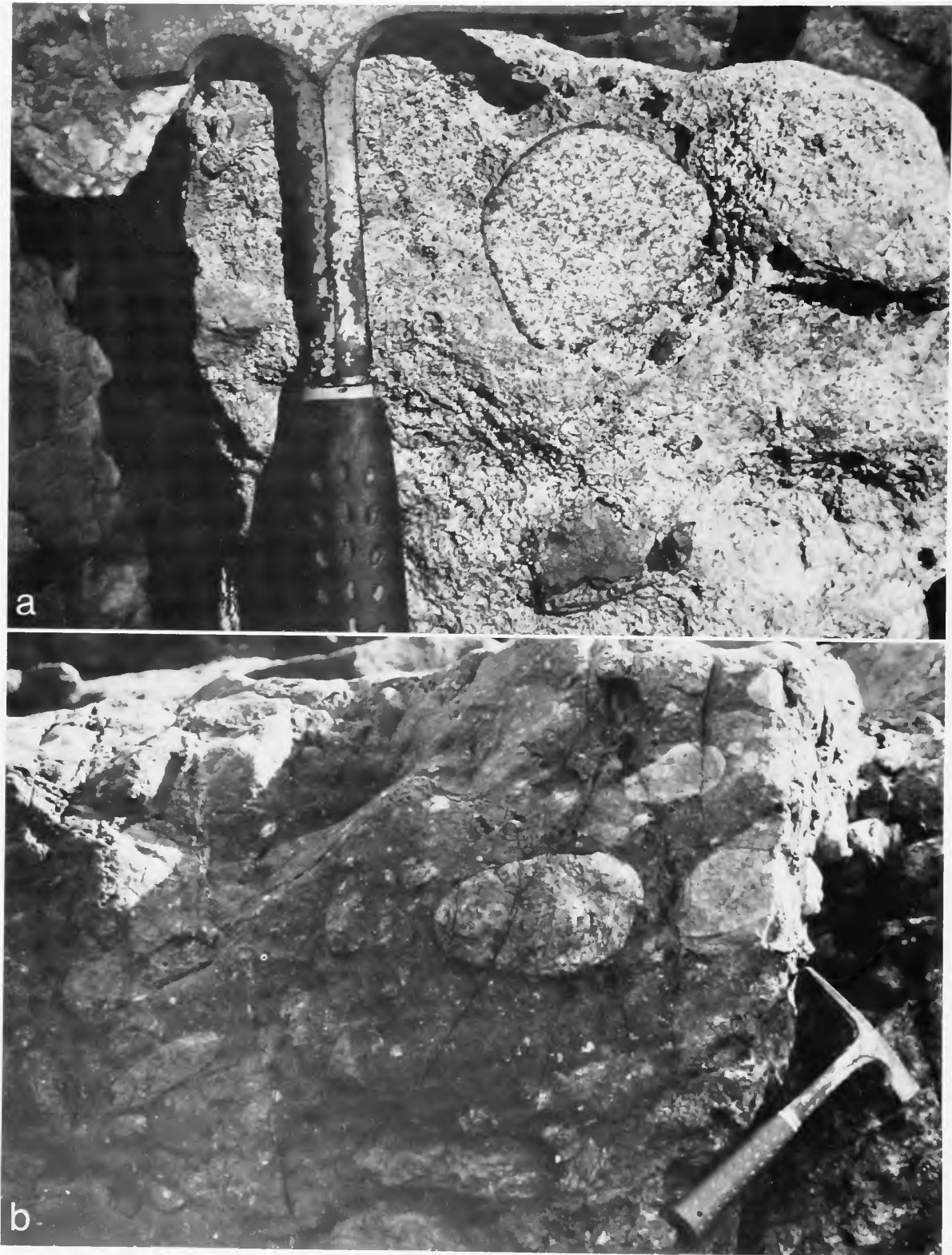
FIGURE 8.—Matrix-supported debris-flow deposits with rounded pebbles in sandstone ( a ) and muddy sandstone ( b ). Localities (in Figure 2): a = site 7; b = site 48. Hammer is 28 cm long.
