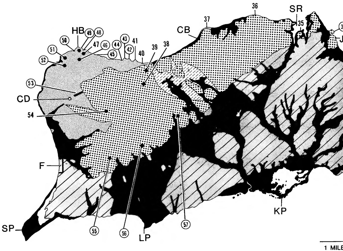
FIGURE 2.—Simplified geological map of St. Croix (modified after Whetten (1966b; 1974, fig. 1) showing 57 localities where samples were collected (geographic names of sites in Table 1 (below), and sample numbers in Table 2). Photographs of representative outcrop exposures, rock slabs, and thin sections presented in this study were selected from 38 localities (circled site number).
