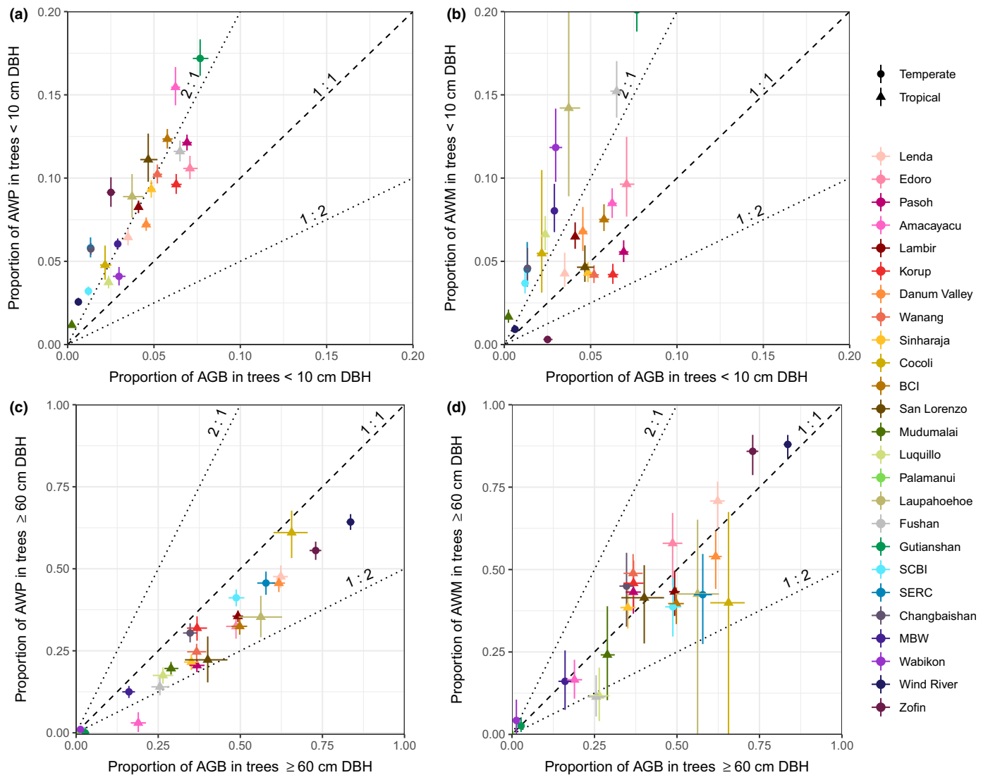
Fig. 4 Proportion of biomass stocks and fluxes in (a, b) small ( 1 \leq \text{DBH} < 10 \text{ cm} ) and (c, d) large trees ( \text{DBH} \geq 60 \text{ cm} ). AGB, aboveground biomass; AWP, aboveground woody productivity; AWM, aboveground woody mortality; DBH, diameter at breast height. Sites are listed in order of absolute latitude in the legend and are colored in warm colors (red to green) for tropical sites and in cold colors (green to blue) for temperate sites. Tropical sites are represented by triangles and temperate sites by circles. Error bars represent 95% confidence intervals after bootstrapping 20 m \times 20 m quadrats with 1000 replicates. Dashed lines correspond to (starting from the top): y = 2x , y = x , and y = x/2 . The upper limit of the x and y-axes on panels (a) and (b) has been set to 0.20 for readability reasons; the full graph (including the Palamanui site) is shown in Supporting Information Fig. S12. BCI, Barro Colorado Island; MBW, Michigan Big Woods; SCBI, Smithsonian Conservation Biology Institute; SERC, Smithsonian Environmental Research Center.
