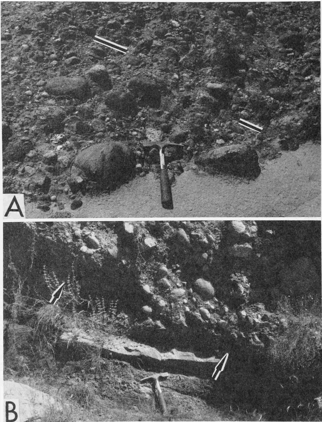
FIGURE 6.—Examples of structures in coarse lenticular facies association: A , matrix supported conglomerate with clasts showing some imbrication of elongate pebbles (bars highlight the a axis of clasts dipping upslope toward SE), basal cobbles, and boulders resting within top of underlying coarse, poorly sorted sandstone, section SE of St. Pierre; B , sharp based (arrows), clast supported conglomerate truncating underlying sandstone layer, megasequence B, NE of Saint-Antonin. (Hammer = 28 cm.)
