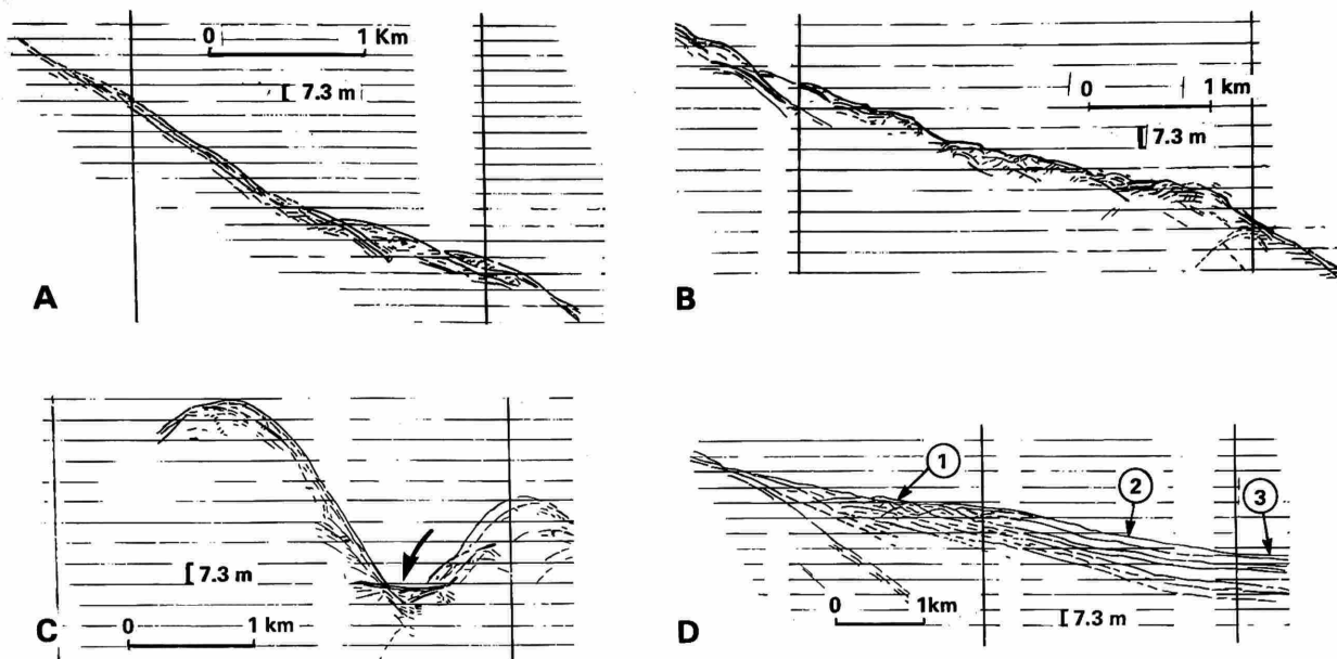
FIGURE 14.—Line drawings of selected 3.5 kHz seismic profiles from the Zakynthos-Strofádhēs Trench system that show sediment failure on steep slopes: A, Slumps with poorly defined internal structure. B, Overlapping series of mass failure deposits. C, Failed sediment accumulating in immediately adjacent depression in cobblestone terrain (arrow). D, Slump deposits showing undefined internal structure at base-of-slope (arrow 1); note improved definition of bedding basinward (arrow 2), and well-stratified ponded facies in the basin plain (arrow 3).
