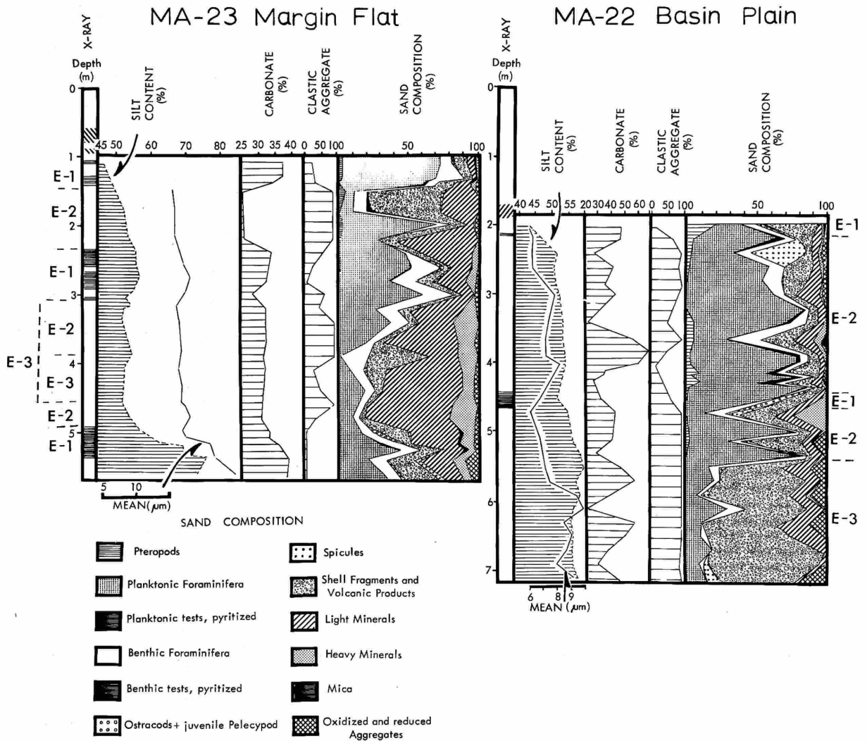
FIGURE 7.—Detailed logs of selected unifies in the Matapan Deep cores MA-23 (trench margin flat) and MA-22 (basin plain). Logs depict major bedform based on x-radiography, grain-size (silt content and mean), carbonate content, clastic aggregates, and other sand-size mineralogical components; the sand-size mineralogical components (excluding clastic aggregates) are recalculated to 100%. (E1 = laminated mud term; E2 = graded mud term; E3 = ungraded mud term; explanation in text.)
