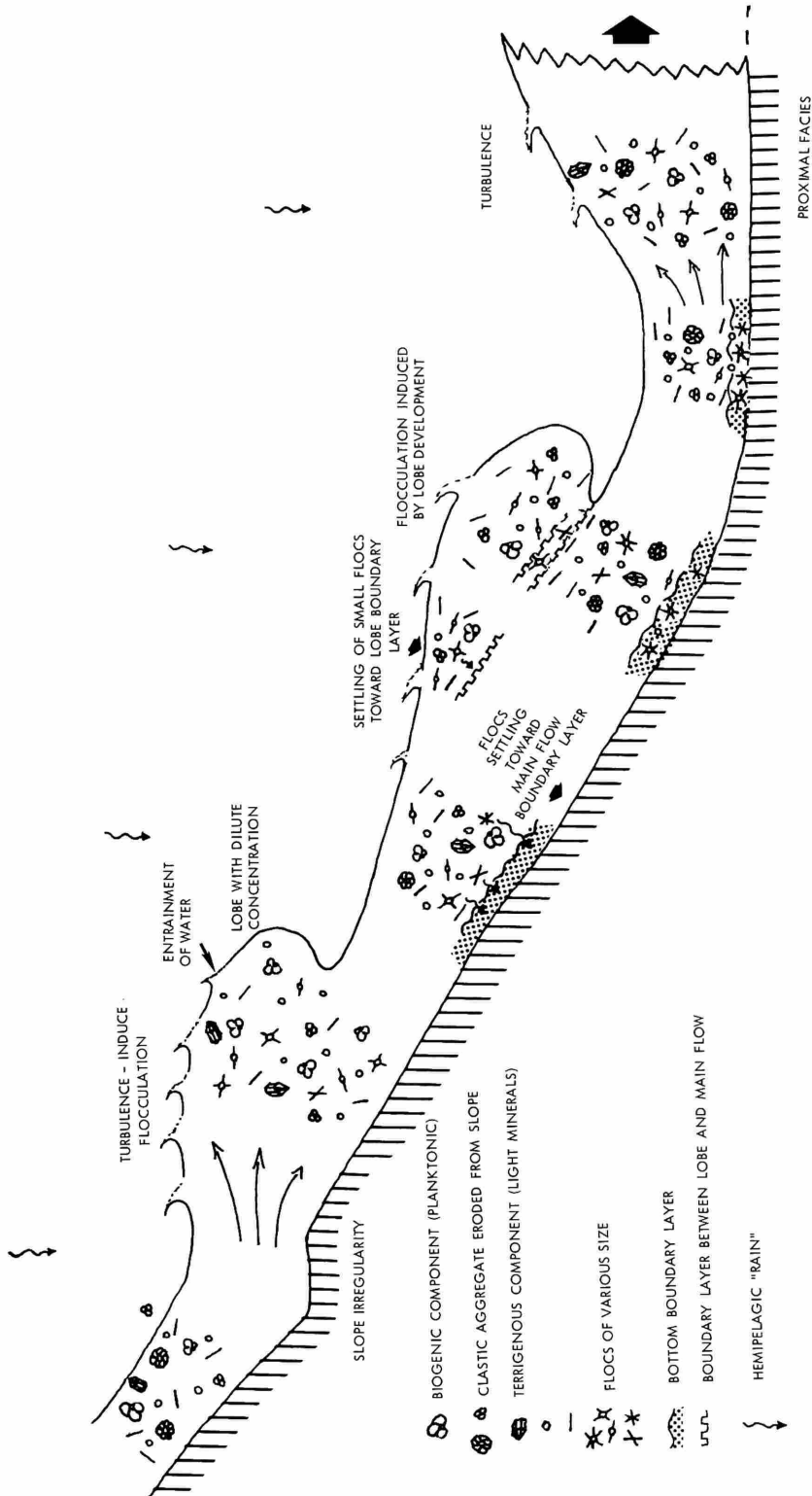
FIGURE 12.—Schemes depicting turbulent sediment gravity flows of the type likely to deposit unifites: A, Transport of largely fine-grained material on a relatively smooth slope. B, transport on an irregular slope produces successive lobes. The diagrams emphasize the effect of grain rearrangement, flocculation, and disaggregation related to the near-bottom boundary layer and the hydraulic jump phenomenon beyond the base-of-slope. These flow-related fluctuations are believed to produce the temporal and spatial petrologic variations of the Hellenic Trench unifites observed in this study. Explanation in text.
