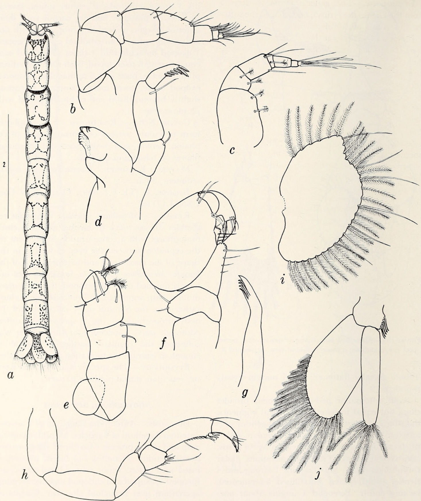
FIGURE 156.— Mesanthura reticulata new species, holotype, ♀: a , complete specimen; b , antenna; c , antennule; d , mandible; e , maxilliped; f , pereopod 1; g , maxilla; h , pereopod 7; i , uropodal exopod; j , pleopod 1.
