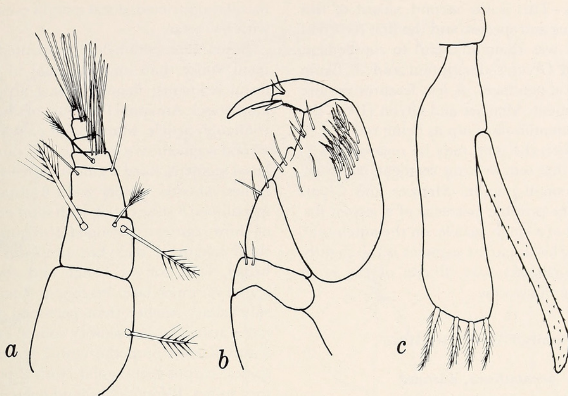
FIGURE 160.— Pendantura tanaiformis Menzies and Glynn, ♂: a , antennule; b , pereopod 1; c , pleopod 2 endopod.
