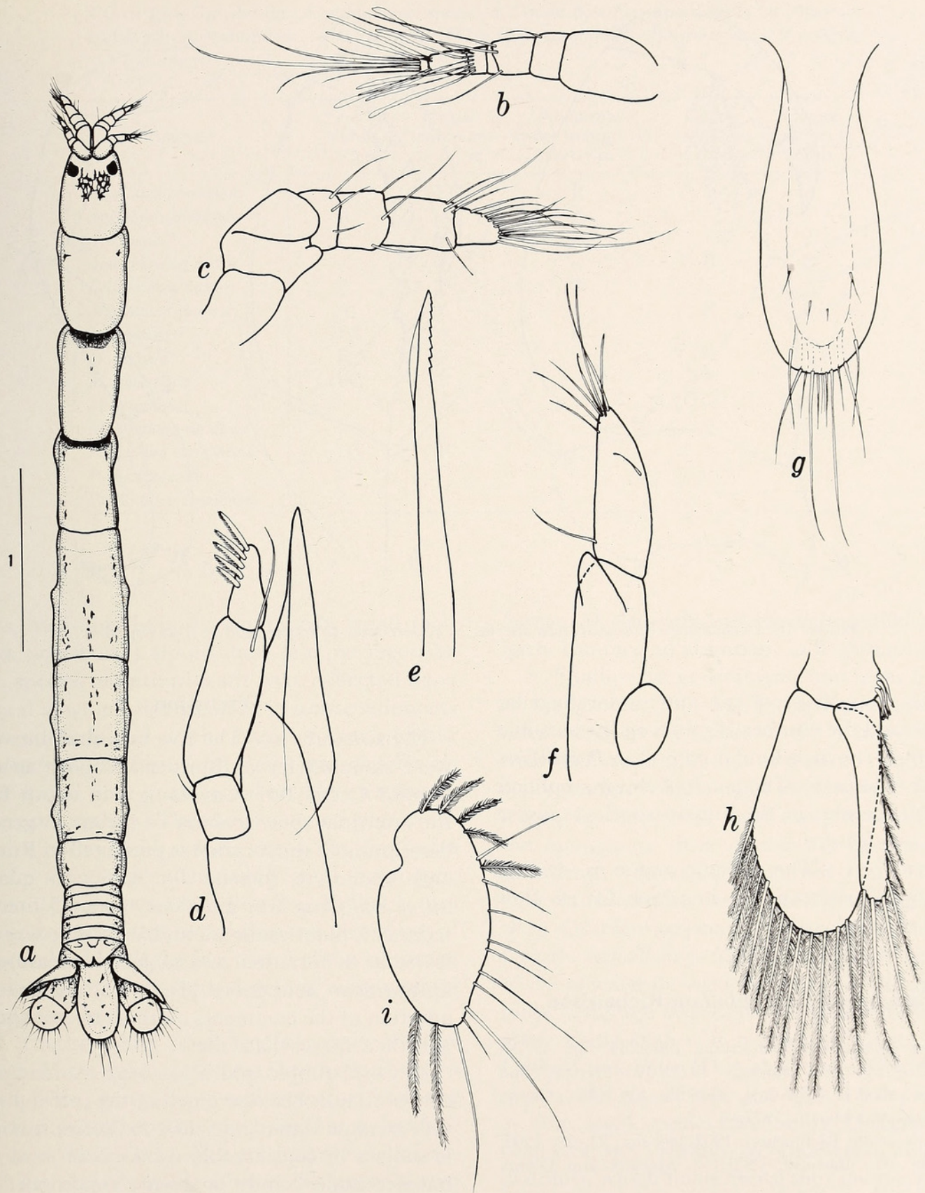
FIGURE 161.— Paranthura caribbiensis new species, holotype, ♀: a, complete specimen; b, antennule; c, antenna; d, mandible; e, maxilla; f, maxilliped; g, telson; h, pleopod 1; i, uropodal exopod.
