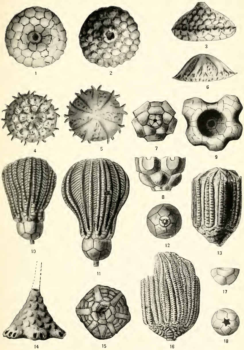
TRROOST'S CRINOIDS OF TENNESSEE.
