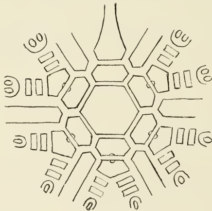
TROOST'S DIAGRAM SHOWING ARRANGEMENT OF PLATES OF A. TUBERCULOSA .
