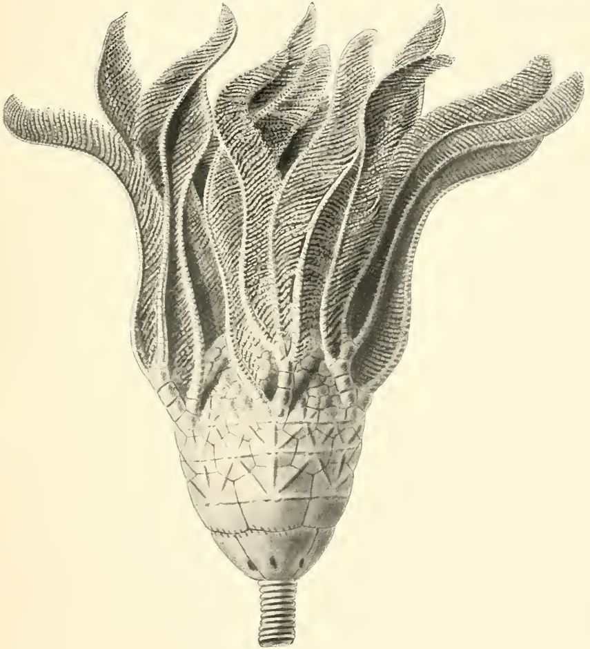
TROOST'S CRINOIDS OF TENNESSEE.
