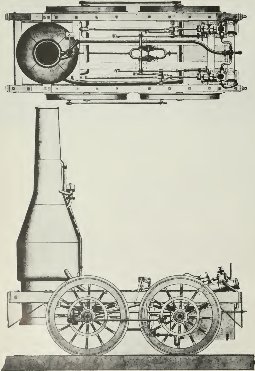
Figure 18.—Early drawing of Best Friend of Charleston , built in 1830.
