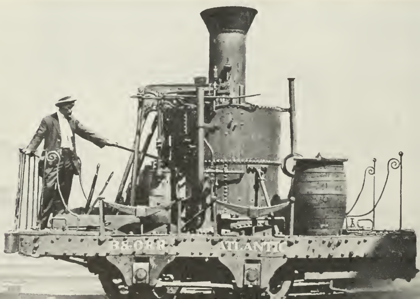
Figure 39. — Andrew Jackson , as remodeled to resemble Atlantic , with Charles B. Chaney at throttle—a photo taken at B & O Mount Clare shops, July 7, 1912. Note wooden barrel used as water tank.
