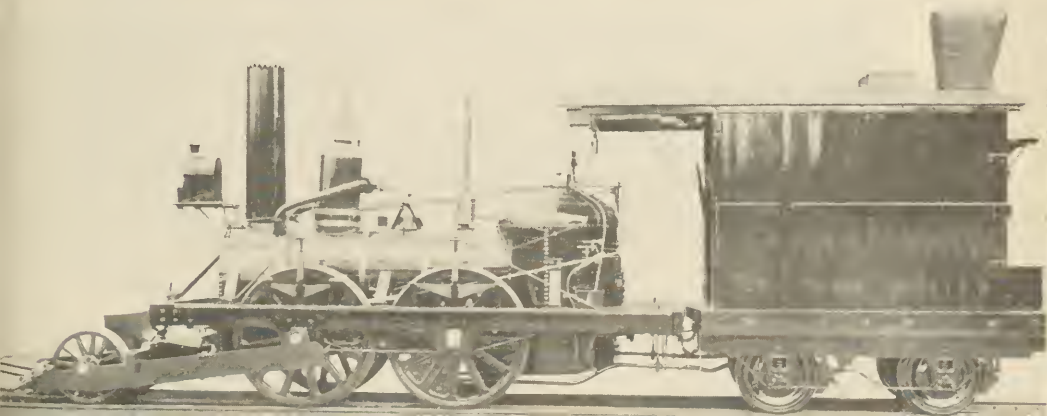
Figure 36.—Full sized operable replica of John Bull , built in 1940 by Pennsylvania Railroad Co.
