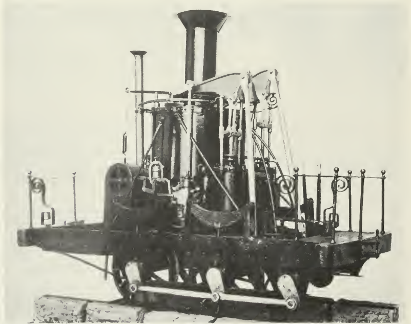
Figure 65.—Model of Davis and Gartner Arabian , 1834.
