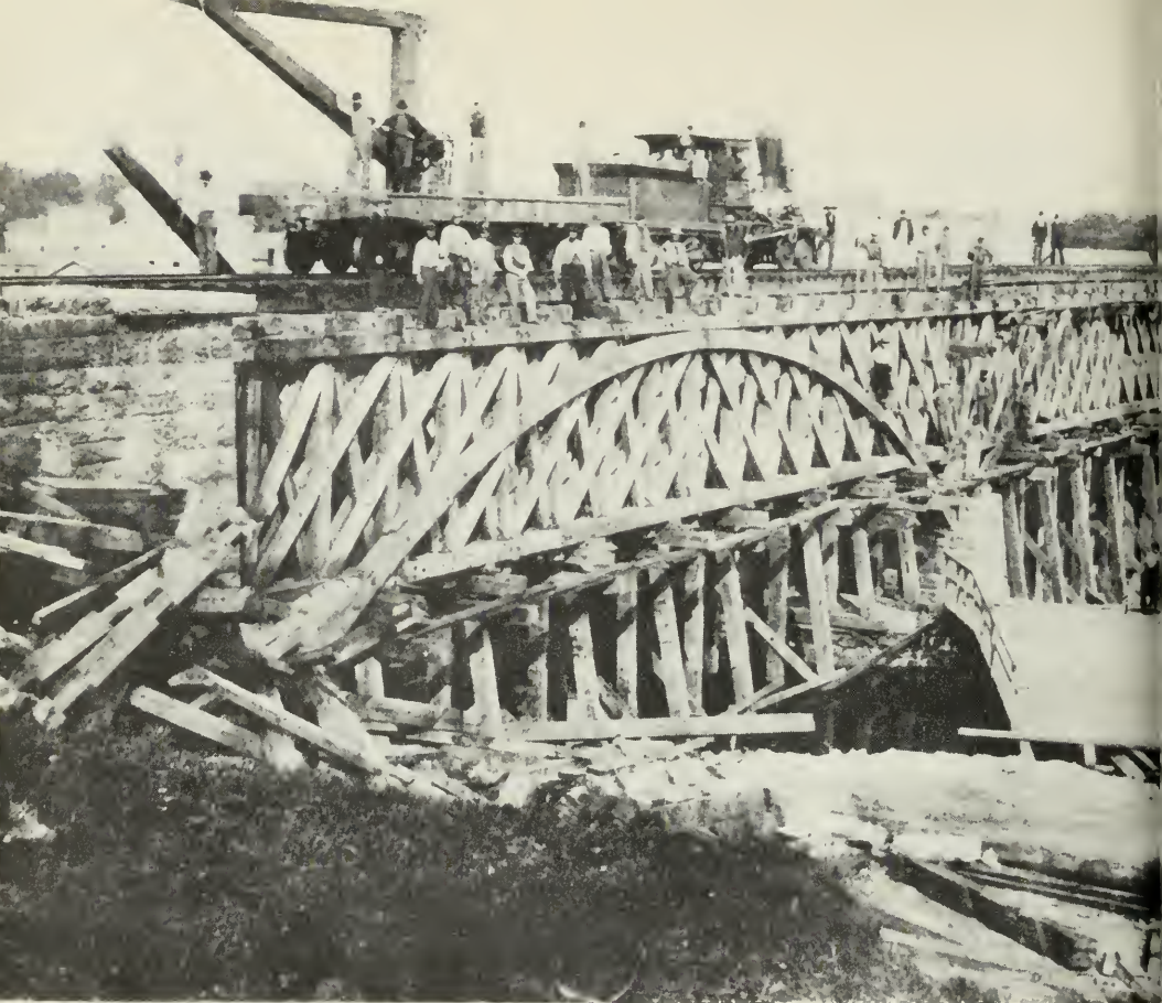
Figure 47.—Earliest known photo of Pioneer , showing it at work in bridge construction at Rockford, Ill., in 1869.
