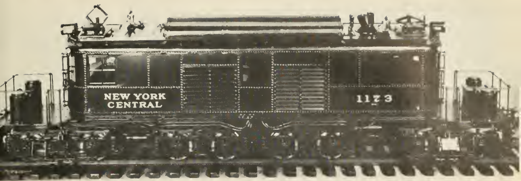
Figure 75.—Operable model of General Electric locomotive, 1926.
