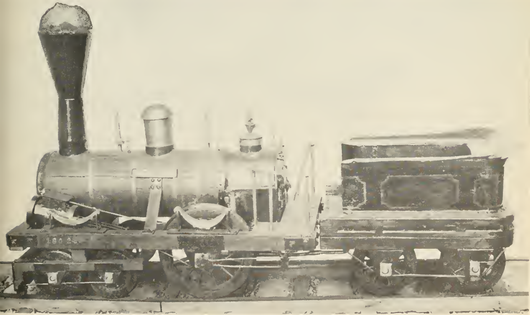
Figure 66.—Model of Rogers, Ketchum & Grosvenor Sandusky , 1837.
