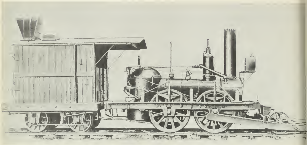
Figure 29.—Pre-1900 photo of John Bull , oldest complete and operable locomotive in North America, now in National Museum.
