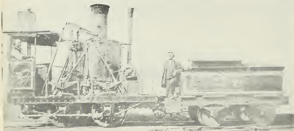
Figure 38. — Andrew Jackson , bearing number "7," in a photo taken between 1850 and January 1, 1884, at which time it was renumbered "2." Note tender.
