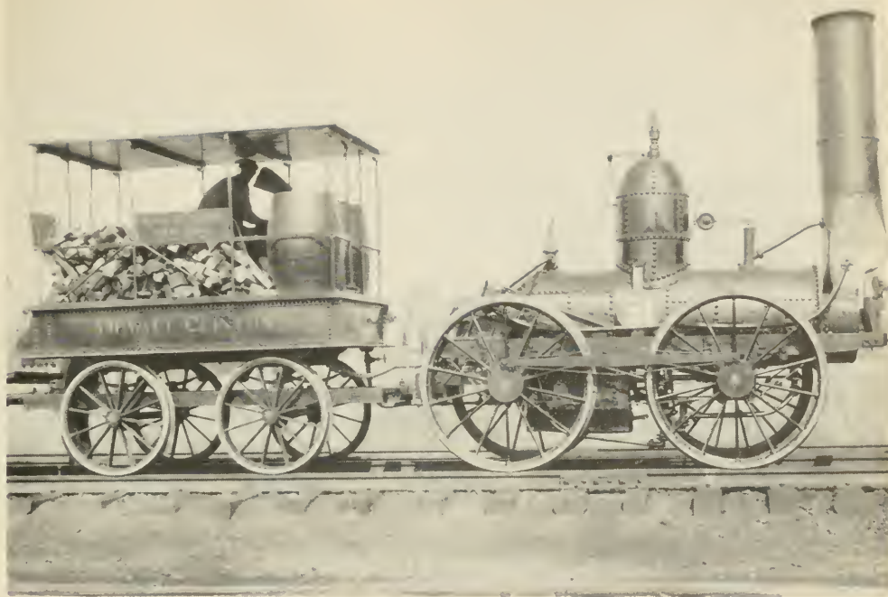
Figure 27.—Replica of De Witt Clinton at the Fair of the Iron Horse in 1927.
