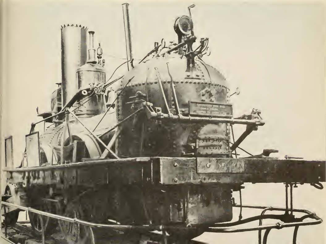
Figure 32.— John Bull on display in National Museum. Note controls and modern steam pressure gauge.
